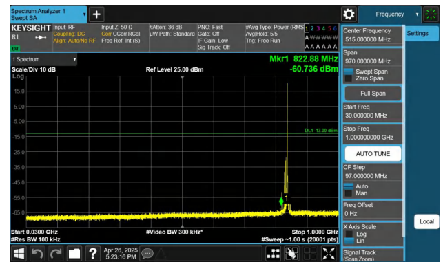
Band5-10MHz-QPSK-20525-1RB#49-30~1000-PASS
