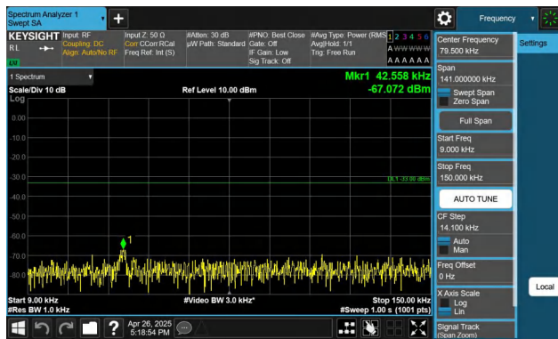
Band5-5MHz-QPSK-20625-1RB#0-0.009~0.15-PASS
