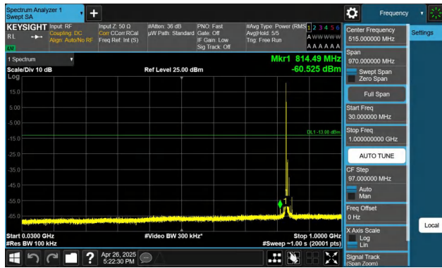
Band5-10MHz-QPSK-20525-1RB#0-30~1000-PASS
