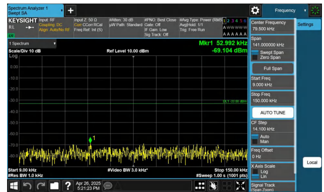
Band5-10MHz-QPSK-20450-1RB#49-0.009~0.15-PASS
