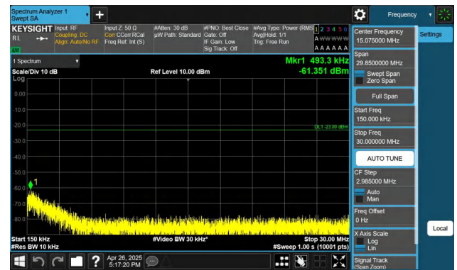
Band5-5MHz-QPSK-20525-1RB#0-0.15~30-PASS
