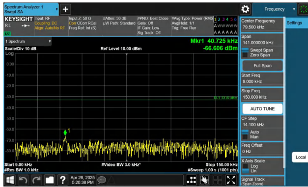
Band5-10MHz-QPSK-20450-1RB#0-0.009~0.15-PASS
