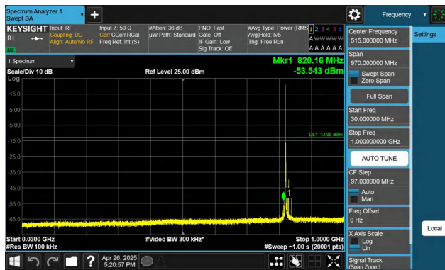
Band5-10MHz-QPSK-20450-1RB#0-30~1000-PASS
