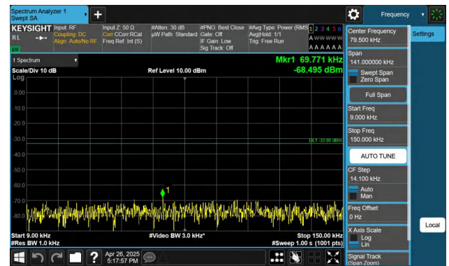
Band5-5MHz-QPSK-20525-1RB#24-0.009~0.15-PASS
