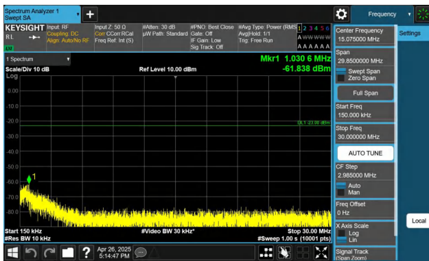
Band5-3MHz-QPSK-20635-1RB#14-0.15~30-PASS
