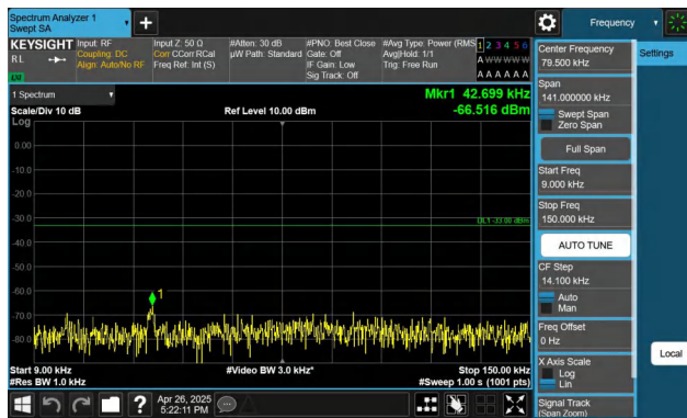
Band5-10MHz-QPSK-20525-1RB#0-0.009~0.15-PASS
