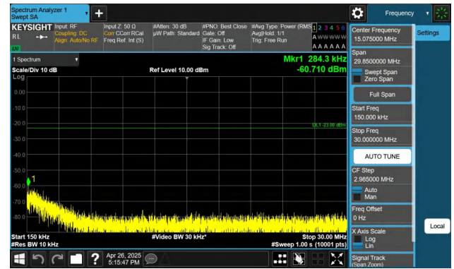
Band5-5MHz-QPSK-20425-1RB#0-0.15~30-PASS
