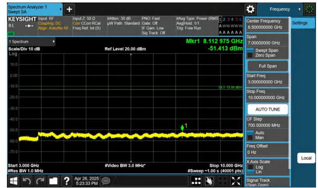
Band5-10MHz-QPSK-20525-1RB#49-3000~10000-PASS
