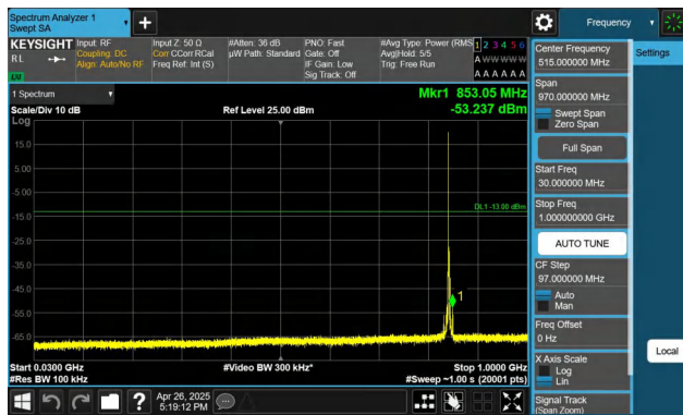
Band5-5MHz-QPSK-20625-1RB#0-30~1000-PASS
