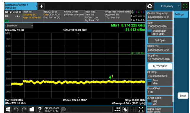
Band5-5MHz-QPSK-20625-1RB#24-3000~10000-PASS
