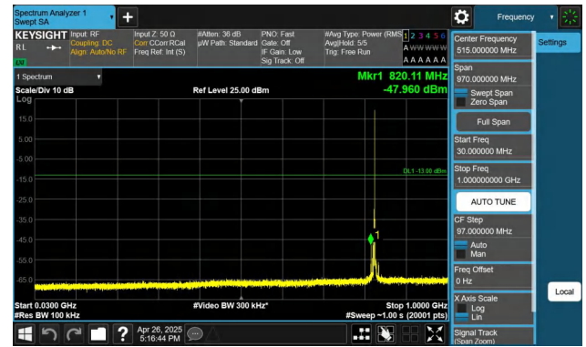
Band5-5MHz-QPSK-20425-1RB#24-30~1000-PASS
