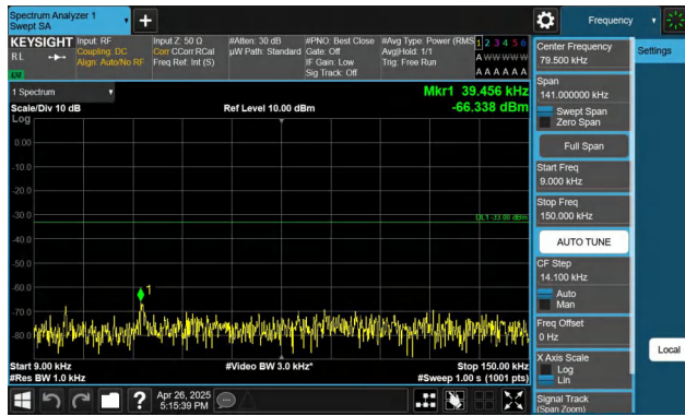
Band5-5MHz-QPSK-20425-1RB#0-0.009~0.15-PASS
