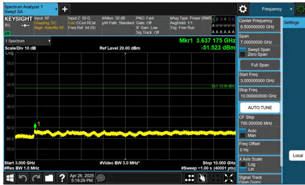
Band5-5MHz-QPSK-20625-1RB#0-3000~10000-PASS
