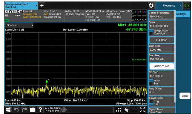
Band5-5MHz-QPSK-20625-1RB#24-0.009~0.15-PASS
