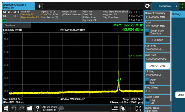
Band5-5MHz-QPSK-20425-1RB#0-30~1000-PASS
