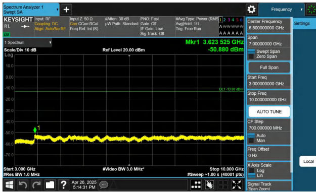
Band5-3MHz-QPSK-20635-1RB#0-3000~10000-PASS
