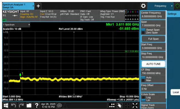
Band5-5MHz-QPSK-20425-1RB#0-3000~10000-PASS
