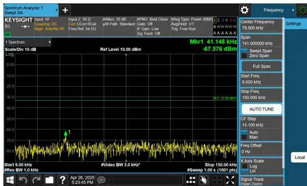
Band5-10MHz-QPSK-20600-1RB#0-0.009~0.15-PASS
