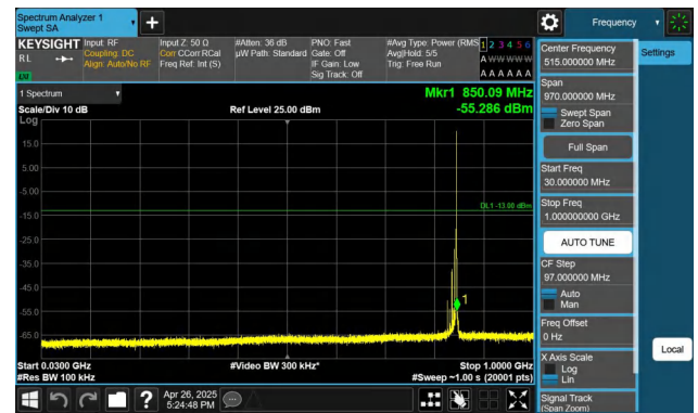
Band5-10MHz-QPSK-20600-1RB#49-30~1000-PASS
