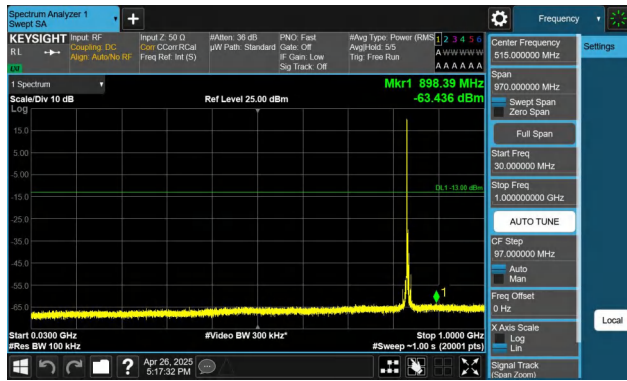
Band5-5MHz-QPSK-20525-1RB#0-30~1000-PASS
