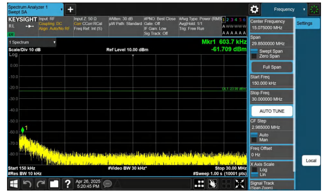
Band5-10MHz-QPSK-20450-1RB#0-0.15~30-PASS
