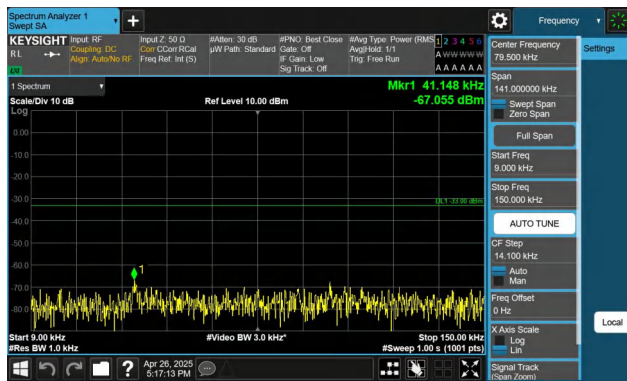
Band5-5MHz-QPSK-20525-1RB#0-0.009~0.15-PASS
