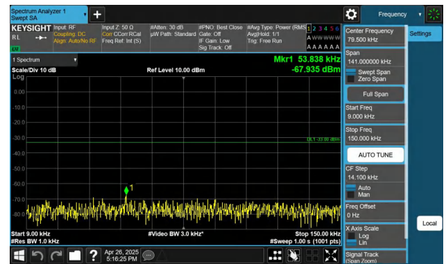
Band5-5MHz-QPSK-20425-1RB#24-0.009~0.15-PASS
