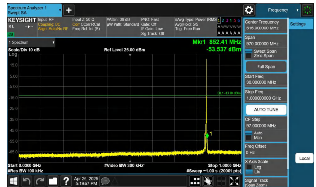
Band5-5MHz-QPSK-20625-1RB#24-30~1000-PASS
