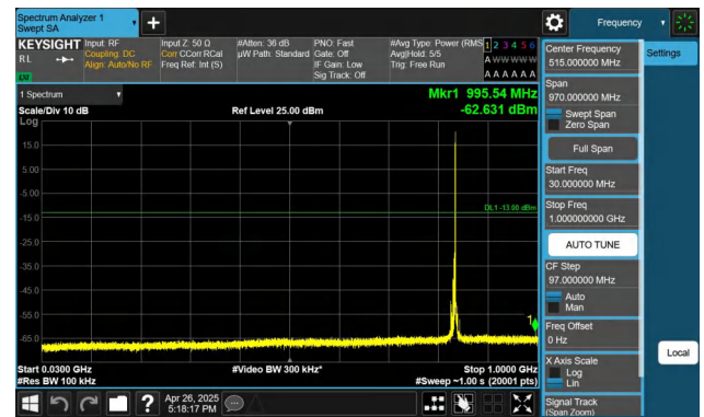
Band5-5MHz-QPSK-20525-1RB#24-30~1000-PASS
