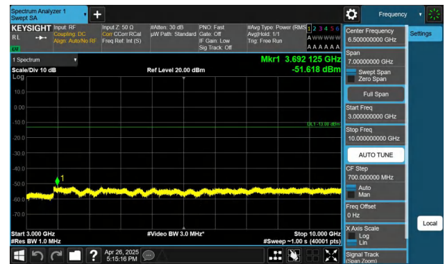
Band5-3MHz-QPSK-20635-1RB#14-3000~10000-PASS
