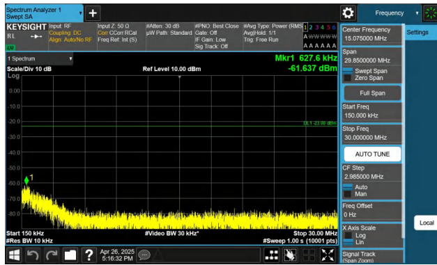
Band5-5MHz-QPSK-20425-1RB#24-0.15~30-PASS
