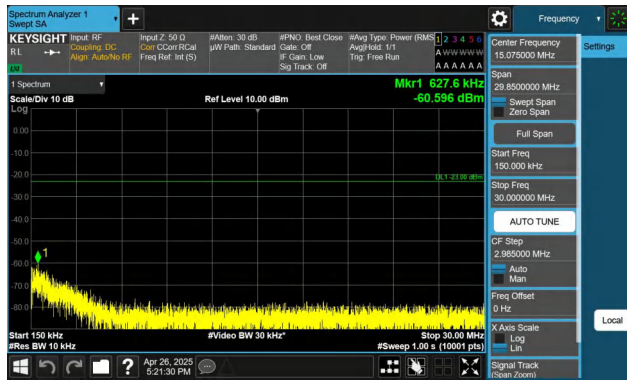
Band5-10MHz-QPSK-20450-1RB#49-0.15~30-PASS
