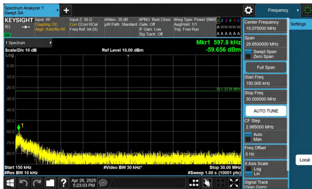
Band5-10MHz-QPSK-20525-1RB#49-0.15~30-PASS
