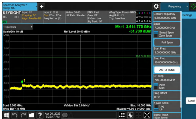
Band5-10MHz-QPSK-20525-1RB#0-3000~10000-PASS
