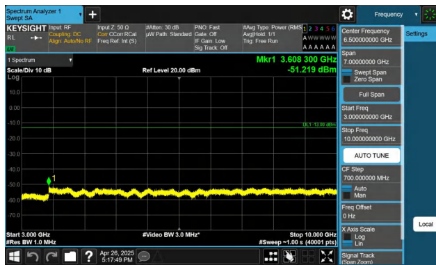
Band5-5MHz-QPSK-20525-1RB#0-3000~10000-PASS
