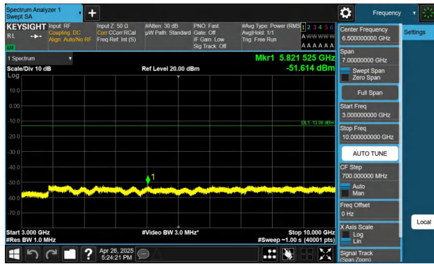
Band5-10MHz-QPSK-20600-1RB#0-3000~10000-PASS
