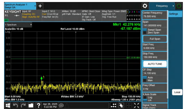
Band5-10MHz-QPSK-20525-1RB#49-0.009~0.15-PASS
