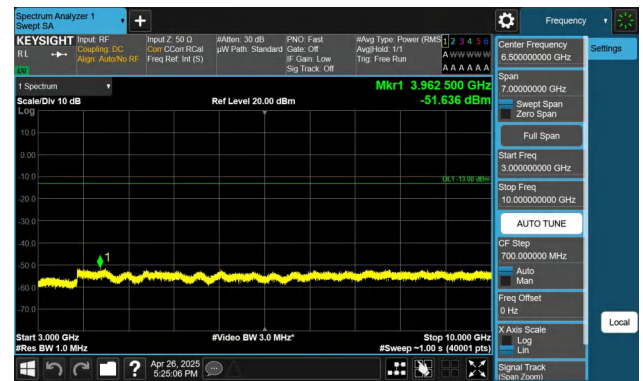
Band5-10MHz-QPSK-20600-1RB#49-3000~10000-PASS
