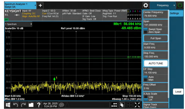
Band5-10MHz-QPSK-20600-1RB#49-0.009~0.15-PASS
