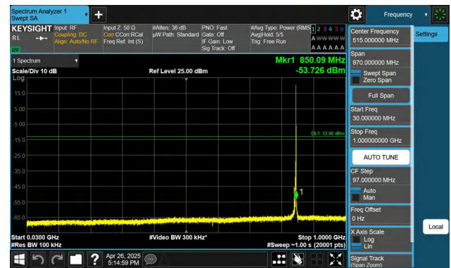
Band5-3MHz-QPSK-20635-1RB#14-30~1000-PASS
