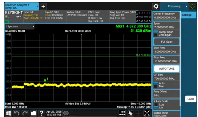
Band5-5MHz-QPSK-20425-1RB#24-3000~10000-PASS
