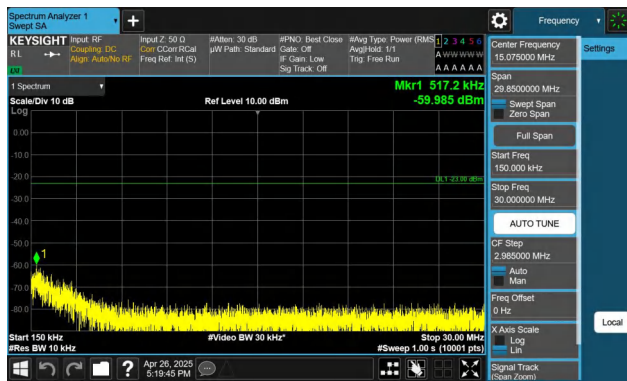
Band5-5MHz-QPSK-20625-1RB#24-0.15~30-PASS
