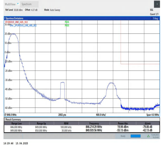
Band5-3MHz-QPSK-20635-1RB#0-PASS
