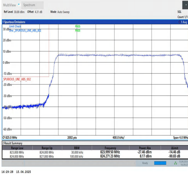
Band5-3MHz-QPSK-20415-15RB#0-PASS
