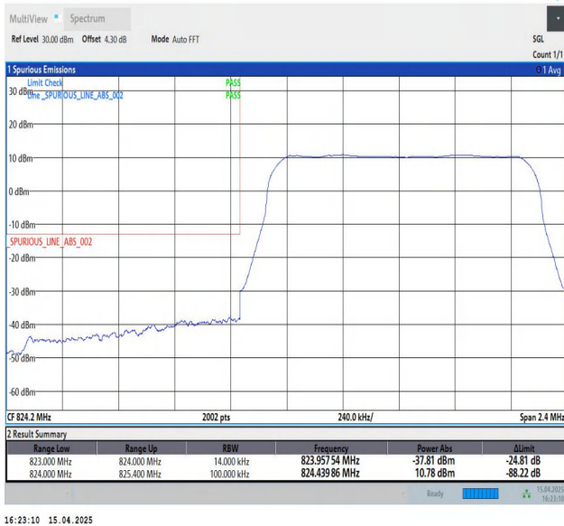
Band5-1.4MHz-QPSK-20407-6RB#0-PASS
