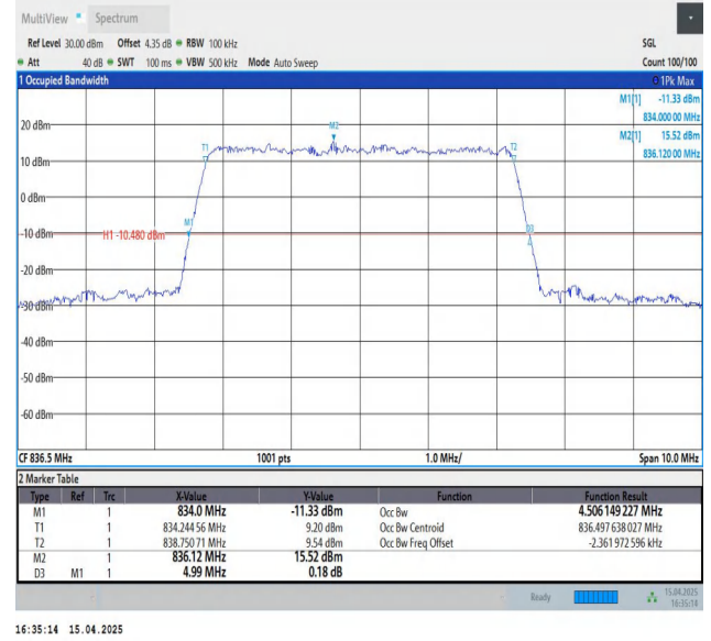
Band5-5MHz-16QAM-20525-25RB#0-PASS
