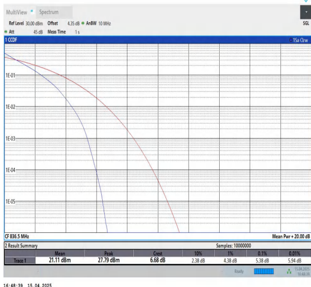
Band5-10MHz-QPSK-20525-50RB#0-PASS
