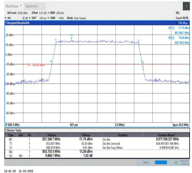
Band5-10MHz-16QAM-20525-50RB#0-PASS
