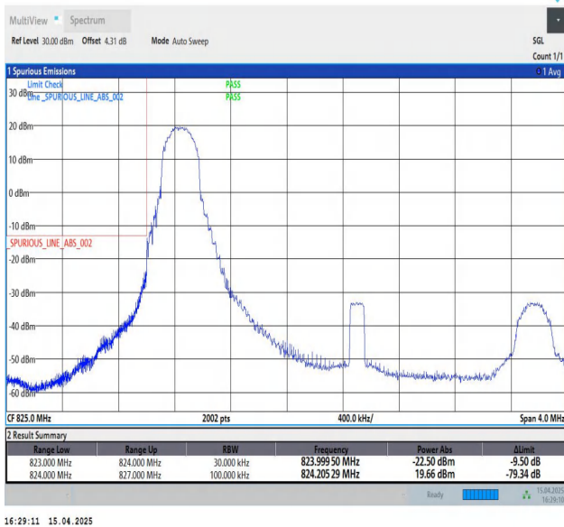
Band5-3MHz-QPSK-20415-1RB#0-PASS
