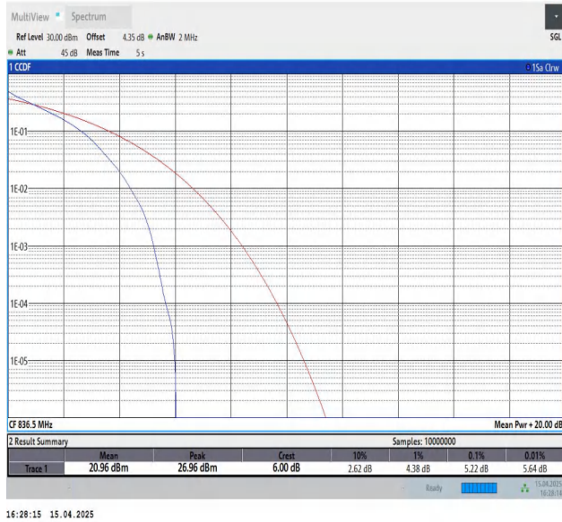
Band5-1.4MHz-QPSK-20525-6RB#0-PASS
