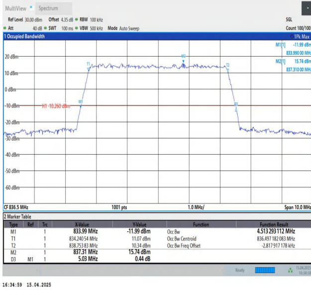
Band5-5MHz-QPSK-20525-25RB#0-PASS
