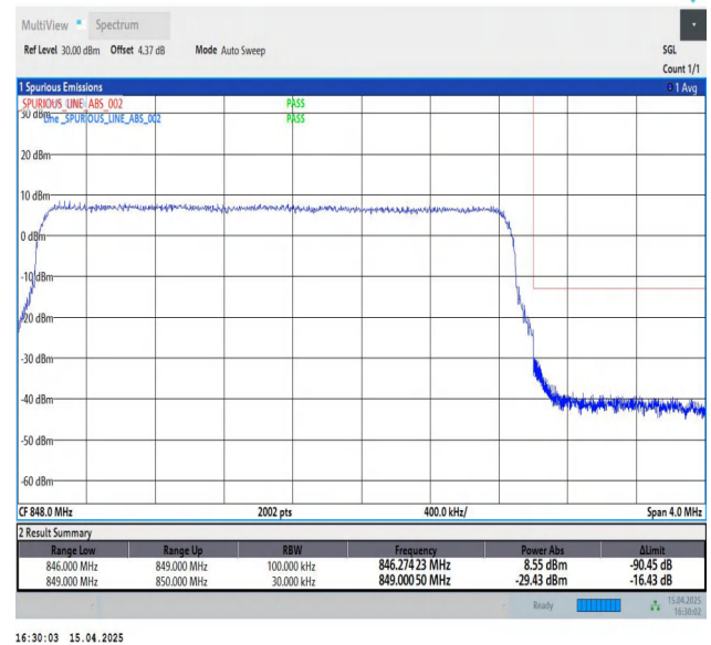
Band5-3MHz-QPSK-20635-15RB#0-PASS
