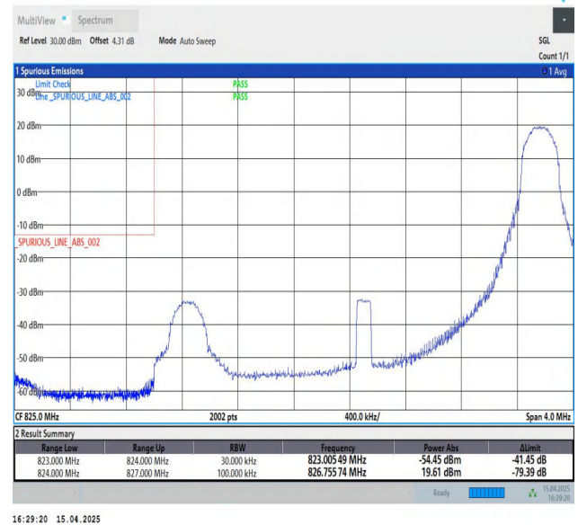
Band5-3MHz-QPSK-20415-1RB#14-PASS
