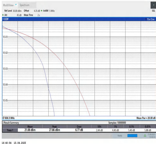
Band5-5MHz-QPSK-20525-25RB#0-PASS
