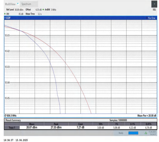
Band5-3MHz-16QAM-20525-15RB#0-PASS
