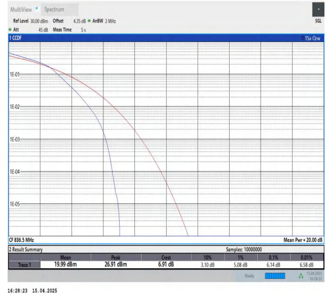
Band5-1.4MHz-16QAM-20525-6RB#0-PASS
