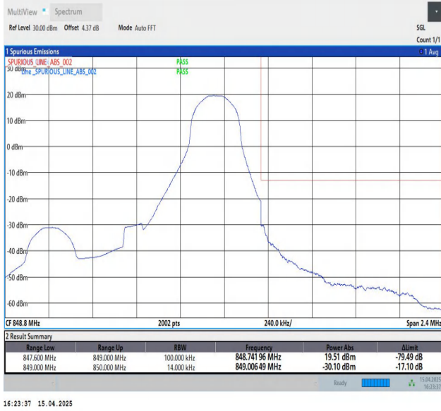
Band5-1.4MHz-QPSK-20643-1RB#5-PASS
