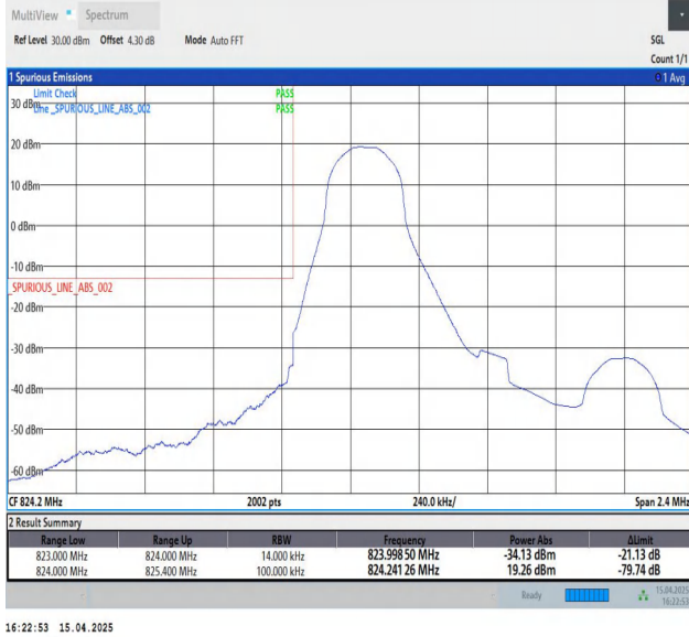
Band5-1.4MHz-QPSK-20407-1RB#0-PASS
