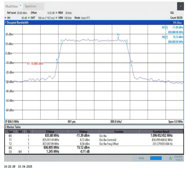
Band5-1.4MHz-16QAM-20525-6RB#0-PASS
