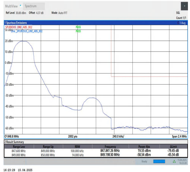
Band5-1.4MHz-QPSK-20643-1RB#0-PASS
