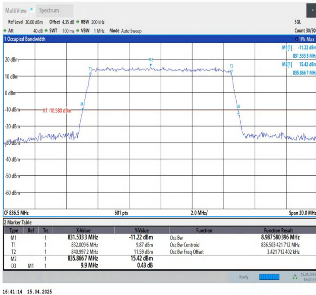
Band5-10MHz-QPSK-20525-50RB#0-PASS
