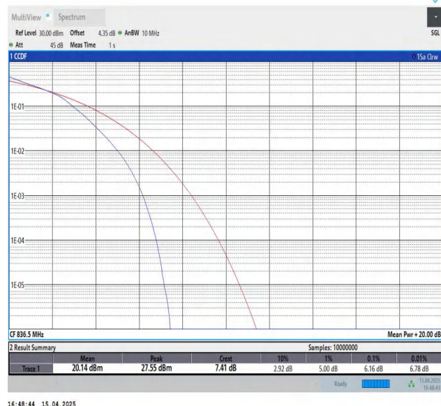
Band5-10MHz-16QAM-20525-50RB#0-PASS
