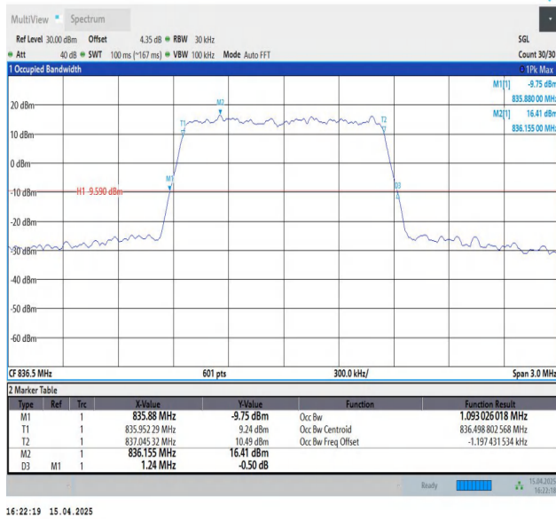
Band5-1.4MHz-QPSK-20525-6RB#0-PASS
