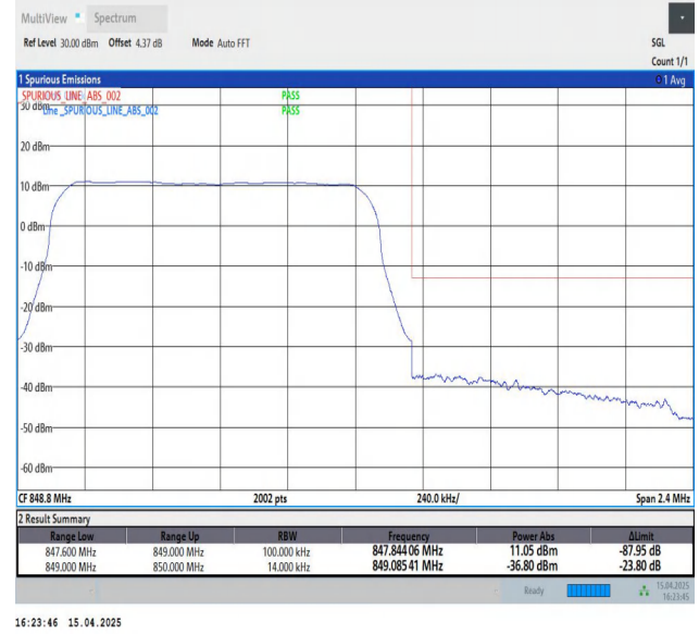
Band5-1.4MHz-QPSK-20643-6RB#0-PASS
