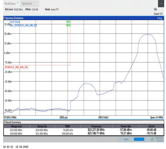
Band5-1.4MHz-QPSK-20407-1RB#5-PASS
