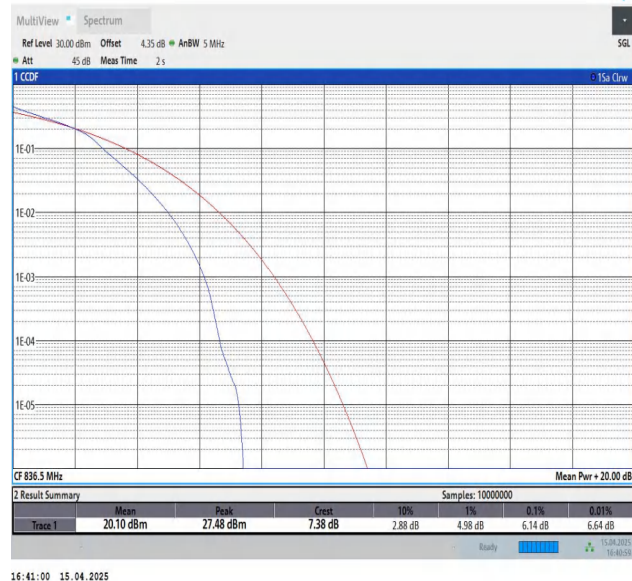
Band5-5MHz-16QAM-20525-25RB#0-PASS
