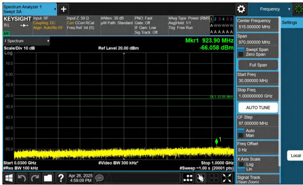
Band4-15MHz-QPSK-20325-1RB#0-30~1000-PASS
