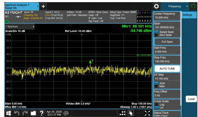
Band4-20MHz-QPSK-20050-1RB#99-0.009~0.15-PASS
