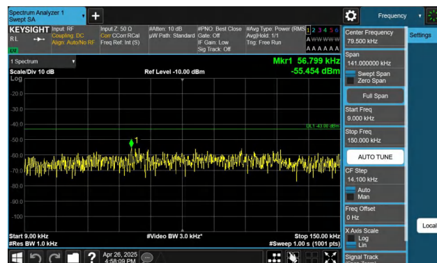
Band4-15MHz-QPSK-20175-1RB#74-0.009~0.15-PASS
