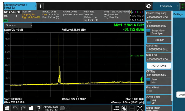
Band4-15MHz-QPSK-20175-1RB#0-1000~3000-PASS
