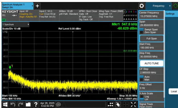
Band4-20MHz-QPSK-20175-1RB#99-0.15~30-PASS
