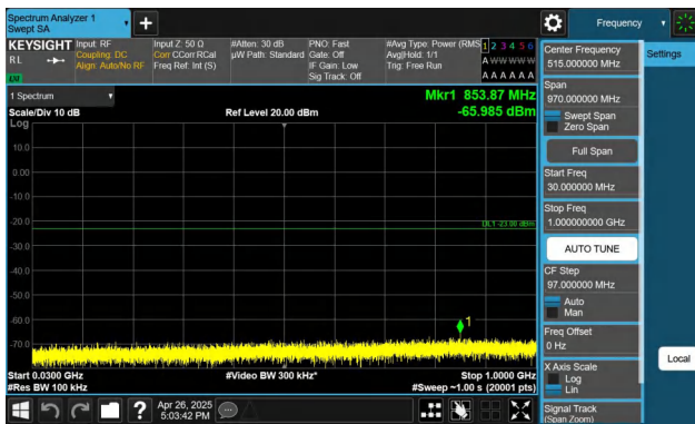
Band4-20MHz-QPSK-20300-1RB#0-30~1000-PASS
