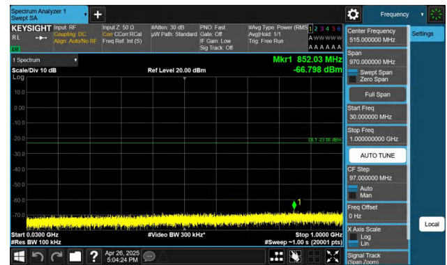
Band4-20MHz-QPSK-20300-1RB#99-30~1000-PASS
