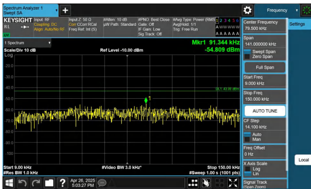
Band4-20MHz-QPSK-20300-1RB#0-0.009~0.15-PASS
