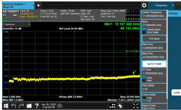
Band4-15MHz-QPSK-20325-1RB#0-3000~20000-PASS
