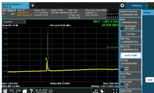
Band4-15MHz-QPSK-20025-1RB#74-1000~3000-PASS
