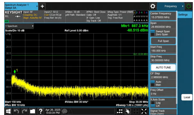
Band4-20MHz-QPSK-20300-1RB#0-0.15~30-PASS
