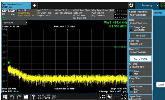
Band4-20MHz-QPSK-20300-1RB#99-0.15~30-PASS
