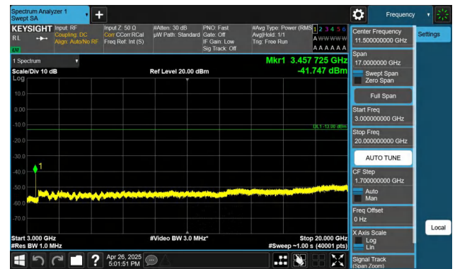
Band4-20MHz-QPSK-20050-1RB#99-3000~20000-PASS
