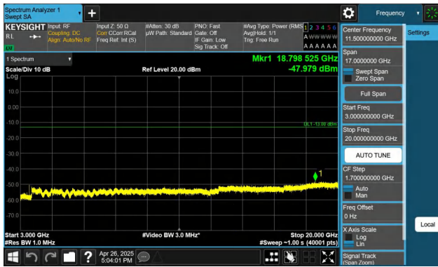
Band4-20MHz-QPSK-20300-1RB#0-3000~20000-PASS
