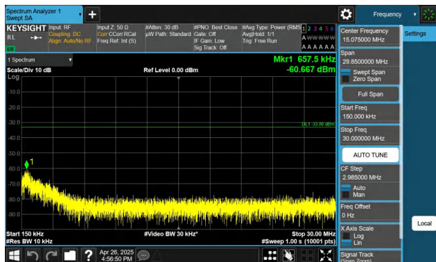
Band4-15MHz-QPSK-20025-1RB#74-0.15~30-PASS
