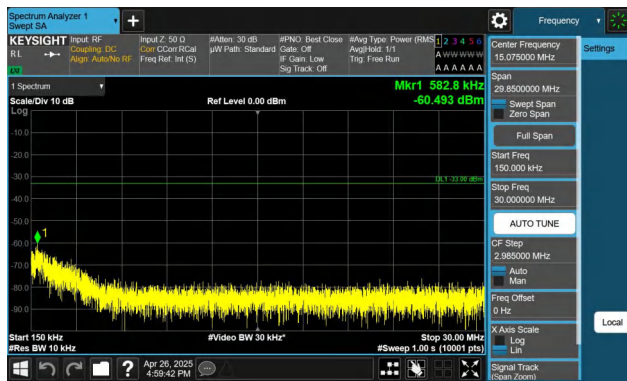
Band4-15MHz-QPSK-20325-1RB#74-0.15~30-PASS
