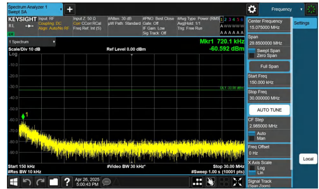
Band4-20MHz-QPSK-20050-1RB#0-0.15~30-PASS
