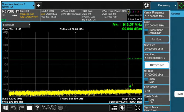
Band4-20MHz-QPSK-20175-1RB#0-30~1000-PASS
