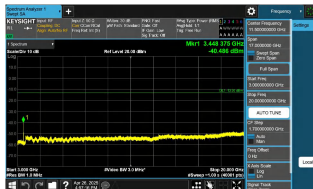
Band4-15MHz-QPSK-20025-1RB#74-3000~20000-PASS
