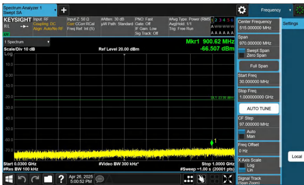
Band4-20MHz-QPSK-20050-1RB#0-30~1000-PASS
