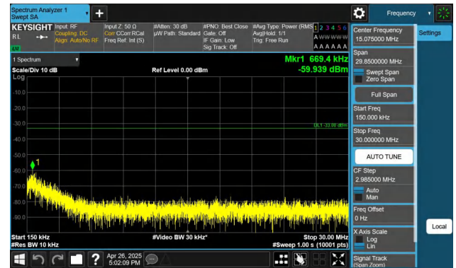
Band4-20MHz-QPSK-20175-1RB#0-0.15~30-PASS
