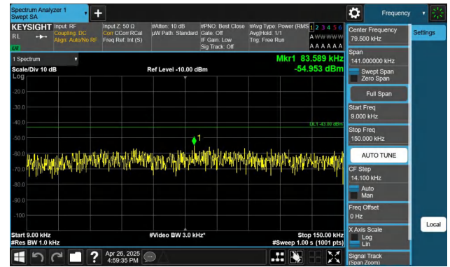
Band4-15MHz-QPSK-20325-1RB#74-0.009~0.15-PASS
