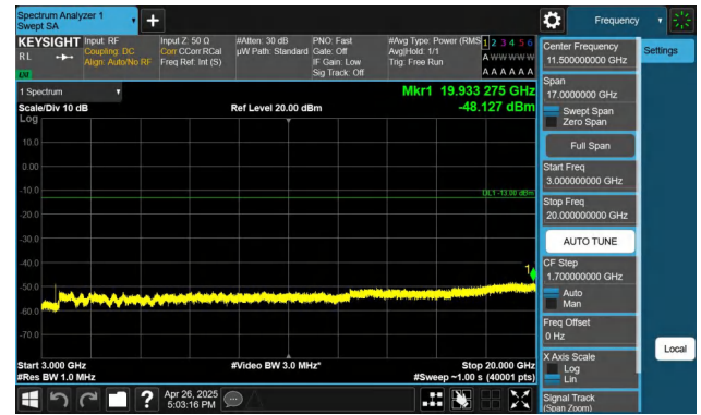
Band4-20MHz-QPSK-20175-1RB#99-3000~20000-PASS
