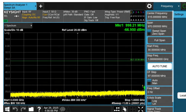
Band4-15MHz-QPSK-20025-1RB#74-30~1000-PASS
