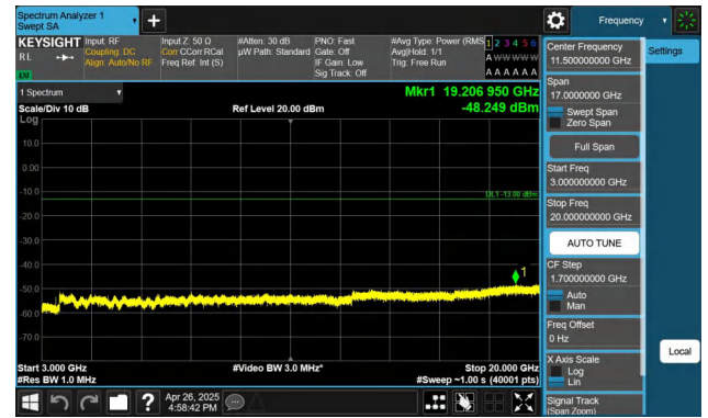
Band4-15MHz-QPSK-20175-1RB#74-3000~20000-PASS
