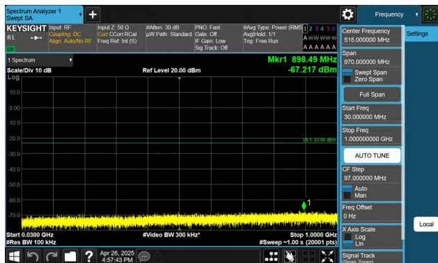
Band4-15MHz-QPSK-20175-1RB#0-30~1000-PASS
