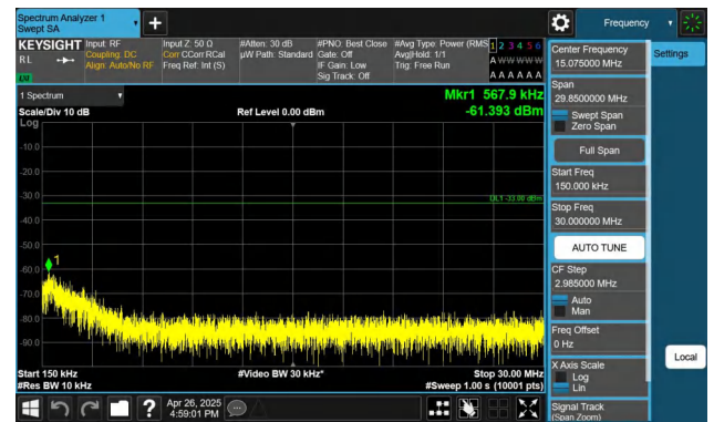
Band4-15MHz-QPSK-20325-1RB#0-0.15~30-PASS
