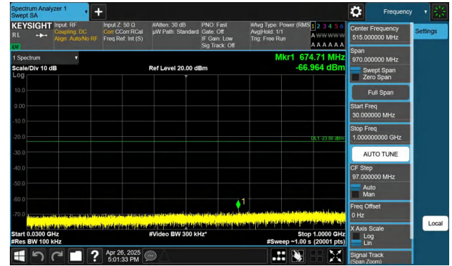
Band4-20MHz-QPSK-20050-1RB#99-30~1000-PASS
