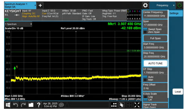
Band4-20MHz-QPSK-20300-1RB#99-3000~20000-PASS
