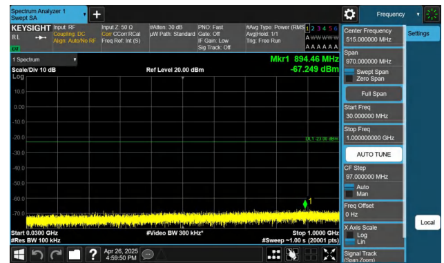
Band4-15MHz-QPSK-20325-1RB#74-30~1000-PASS
