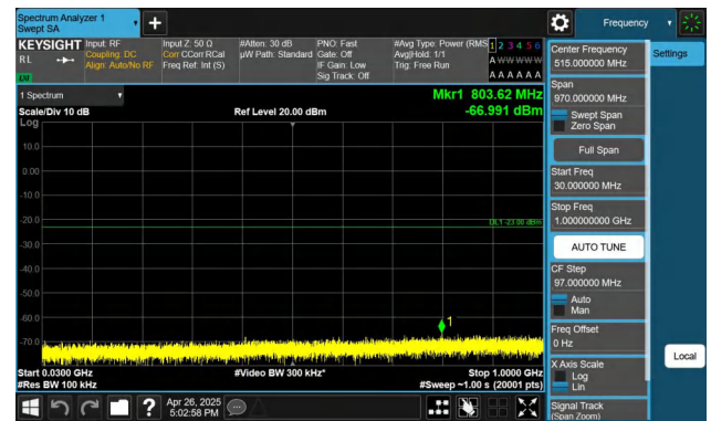
Band4-20MHz-QPSK-20175-1RB#99-30~1000-PASS
