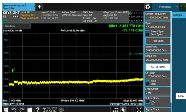
Band4-15MHz-QPSK-20175-1RB#0-3000~20000-PASS
