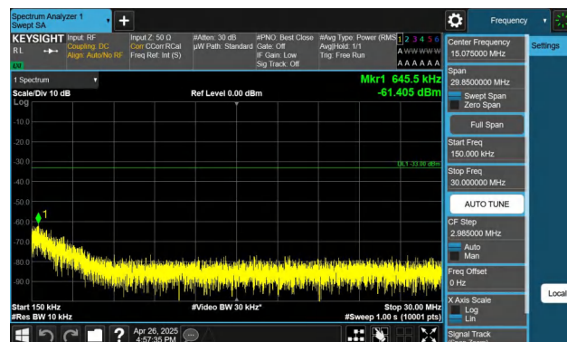
Band4-15MHz-QPSK-20175-1RB#0-0.15~30-PASS
