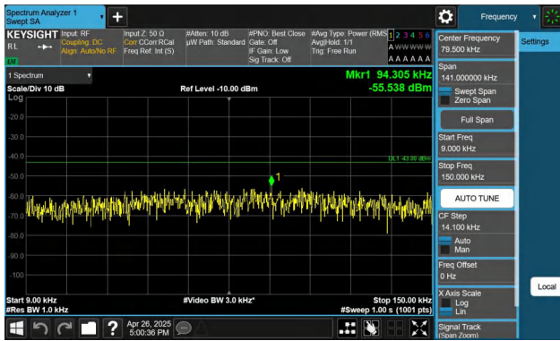
Band4-20MHz-QPSK-20050-1RB#0-0.009~0.15-PASS
