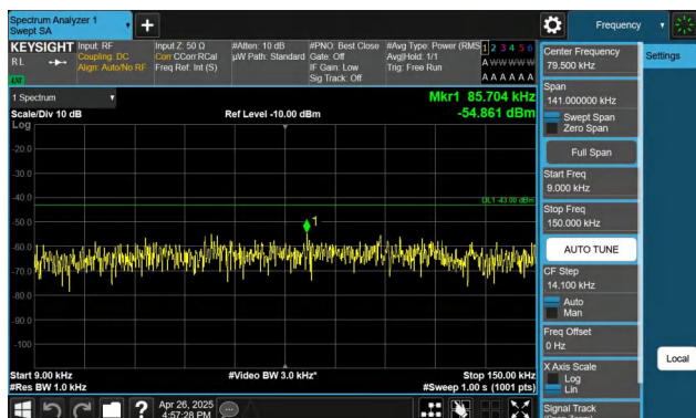
Band4-15MHz-QPSK-20175-1RB#0-0.009~0.15-PASS
