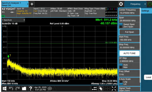
Band4-20MHz-QPSK-20050-1RB#99-0.15~30-PASS
