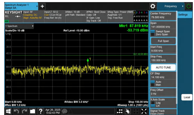
Band4-20MHz-QPSK-20175-1RB#99-0.009~0.15-PASS
