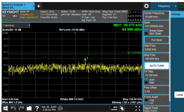
Band4-15MHz-QPSK-20325-1RB#0-0.009~0.15-PASS
