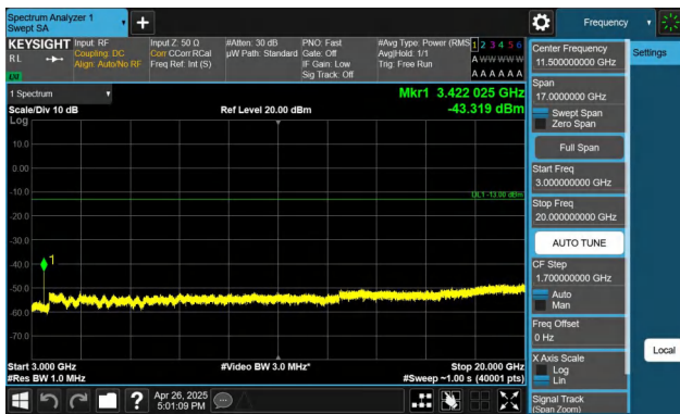
Band4-20MHz-QPSK-20050-1RB#0-3000~20000-PASS
