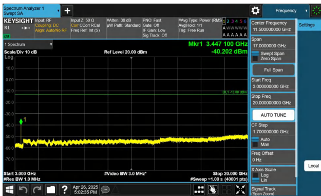
Band4-20MHz-QPSK-20175-1RB#0-3000~20000-PASS
