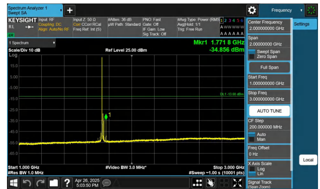
Band4-20MHz-QPSK-20300-1RB#0-1000~3000-PASS
