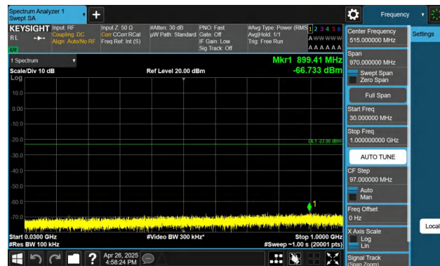
Band4-15MHz-QPSK-20175-1RB#74-30~1000-PASS
