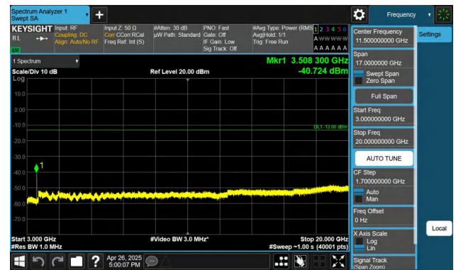
Band4-15MHz-QPSK-20325-1RB#74-3000~20000-PASS
