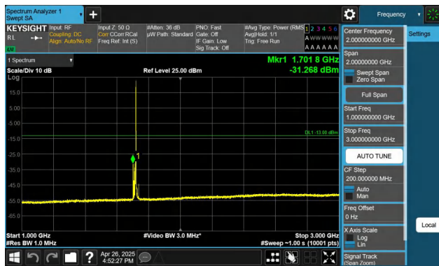
Band4-10MHz-QPSK-20000-1RB#49-1000~3000-PASS
