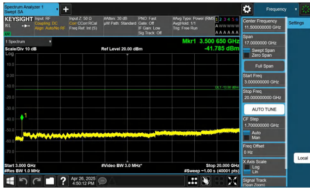
Band4-5MHz-QPSK-20375-1RB#0-3000~20000-PASS
