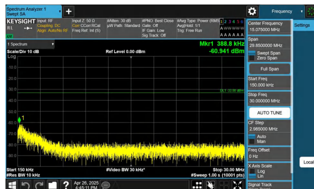
Band4-3MHz-QPSK-20385-1RB#0-0.15~30-PASS
