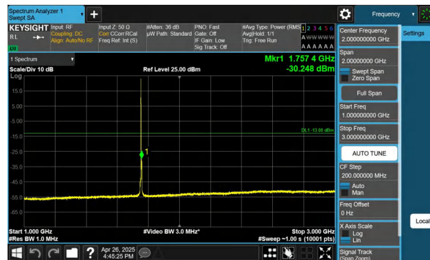
Band4-3MHz-QPSK-20385-1RB#0-1000~3000-PASS
