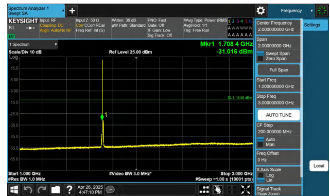
Band4-5MHz-QPSK-19975-1RB#0-1000~3000-PASS
