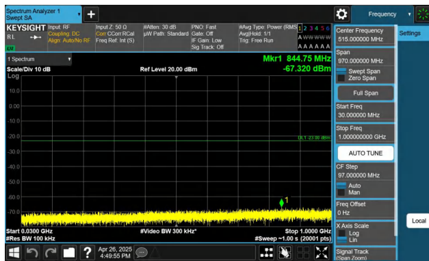
Band4-5MHz-QPSK-20375-1RB#0-30~1000-PASS
