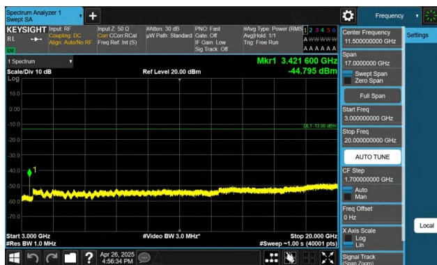
Band4-15MHz-QPSK-20025-1RB#0-3000~20000-PASS
