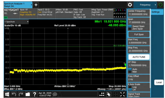
Band4-10MHz-QPSK-20175-1RB#49-3000~20000-PASS
