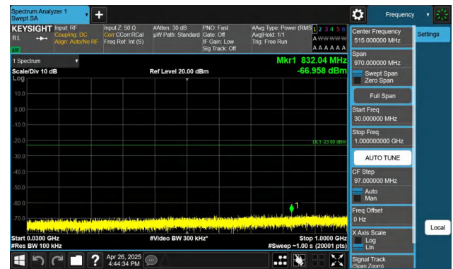
Band4-3MHz-QPSK-20175-1RB#14-30~1000-PASS
