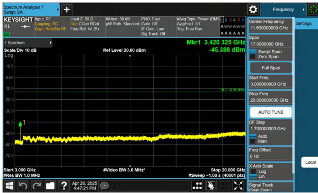
Band4-5MHz-QPSK-19975-1RB#0-3000~20000-PASS
