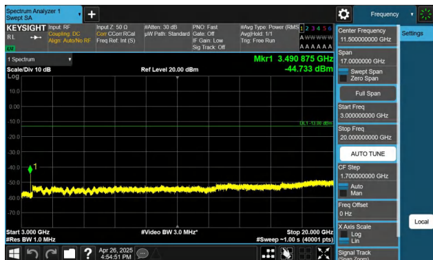
Band4-10MHz-QPSK-20350-1RB#0-3000~20000-PASS
