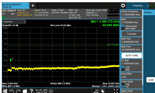
Band4-5MHz-QPSK-20175-1RB#0-3000~20000-PASS
