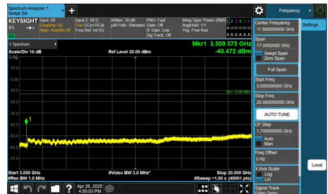
Band4-5MHz-QPSK-20375-1RB#24-3000~20000-PASS
