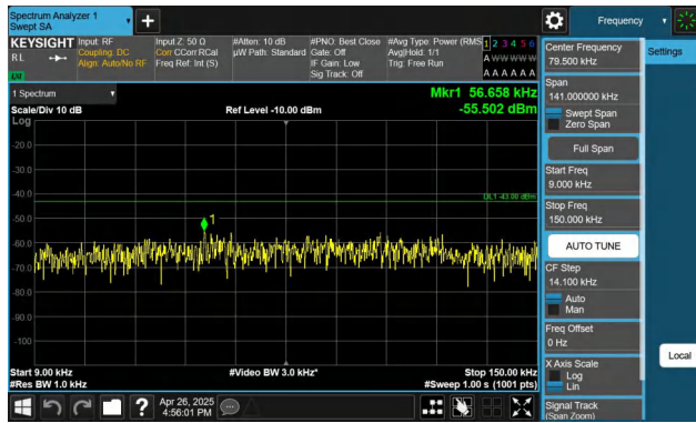
Band4-15MHz-QPSK-20025-1RB#0-0.009~0.15-PASS
