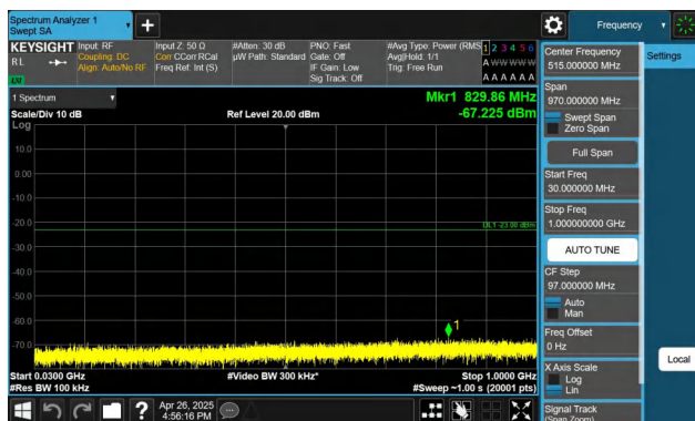
Band4-15MHz-QPSK-20025-1RB#0-30~1000-PASS
