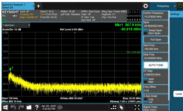
Band4-3MHz-QPSK-20385-1RB#14-0.15~30-PASS
