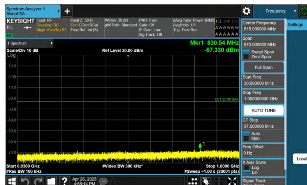
Band4-10MHz-QPSK-20350-1RB#49-30~1000-PASS
