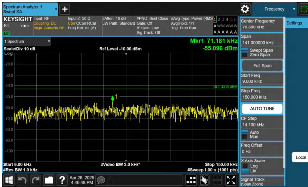
Band4-5MHz-QPSK-19975-1RB#0-0.009~0.15-PASS
