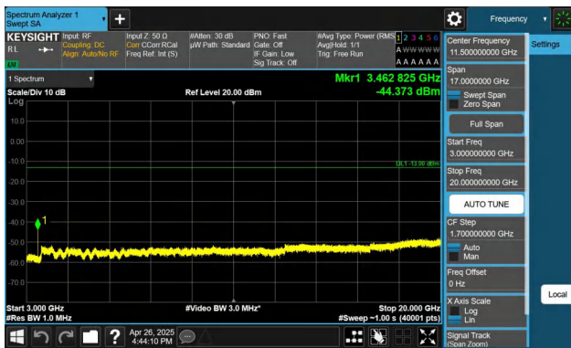
Band4-3MHz-QPSK-20175-1RB#0-3000~20000-PASS
