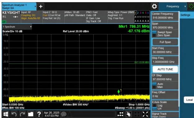
Band4-5MHz-QPSK-19975-1RB#0-30~1000-PASS
