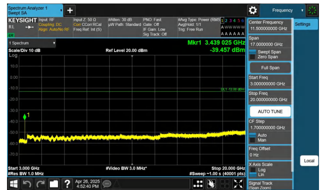
Band4-10MHz-QPSK-20000-1RB#49-3000~20000-PASS
