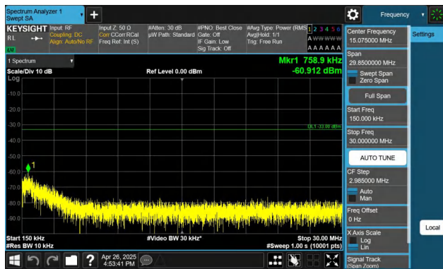
Band4-10MHz-QPSK-20175-1RB#49-0.15~30-PASS
