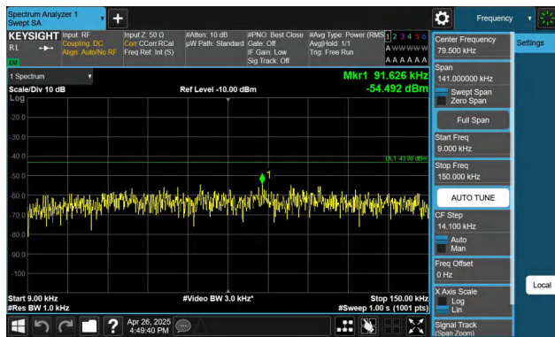
Band4-5MHz-QPSK-20375-1RB#0-0.009~0.15-PASS
