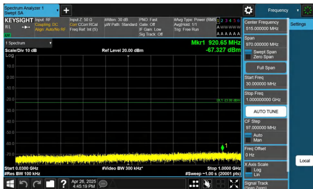
Band4-3MHz-QPSK-20385-1RB#0-30~1000-PASS
