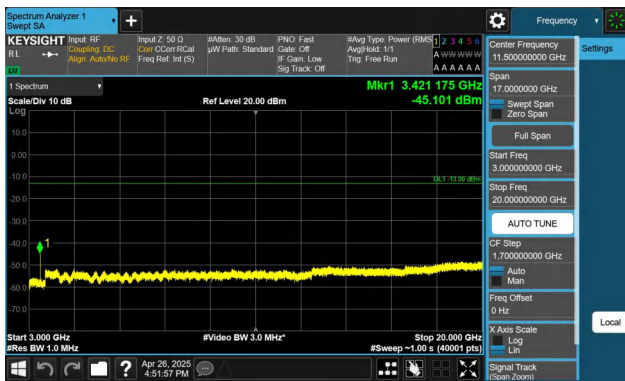
Band4-10MHz-QPSK-20000-1RB#0-3000~20000-PASS
