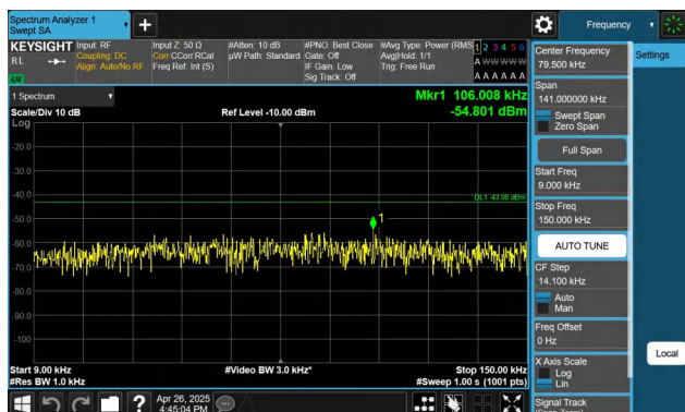
Band4-3MHz-QPSK-20385-1RB#0-0.009~0.15-PASS
