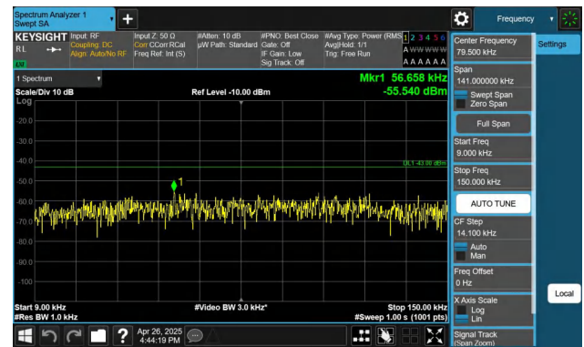
Band4-3MHz-QPSK-20175-1RB#14-0.009~0.15-PASS
