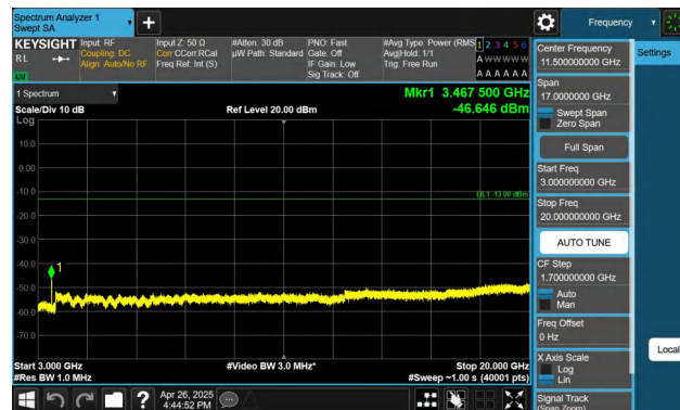
Band4-3MHz-QPSK-20175-1RB#14-3000~20000-PASS
