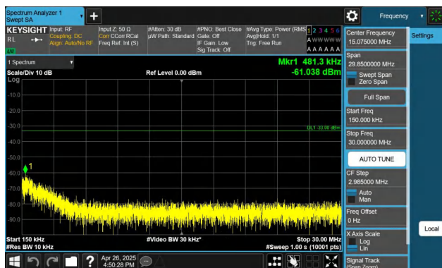
Band4-5MHz-QPSK-20375-1RB#24-0.15~30-PASS
