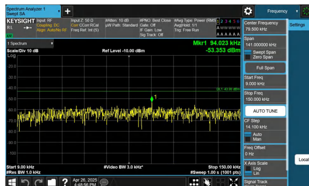
Band4-5MHz-QPSK-20175-1RB#24-0.009~0.15-PASS
