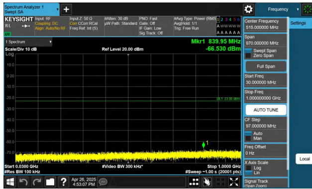
Band4-10MHz-QPSK-20175-1RB#0-30~1000-PASS
