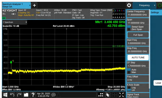
Band4-10MHz-QPSK-20175-1RB#0-3000~20000-PASS
