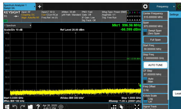
Band4-5MHz-QPSK-20175-1RB#24-30~1000-PASS
