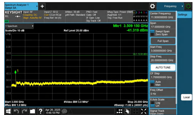
Band4-3MHz-QPSK-20385-1RB#14-3000~20000-PASS
