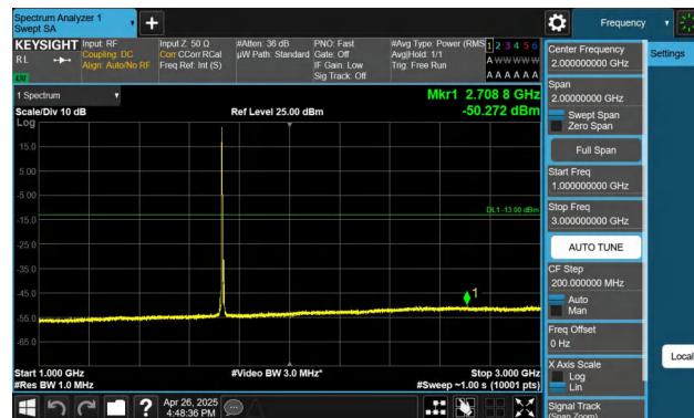
Band4-5MHz-QPSK-20175-1RB#0-1000~3000-PASS
