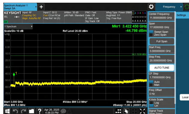
Band4-1.4MHz-QPSK-19957-1RB#5-3000~20000-PASS
