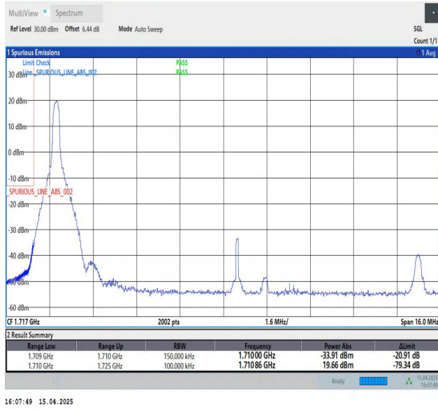
Band4-15MHz-QPSK-20025-1RB#0-PASS
