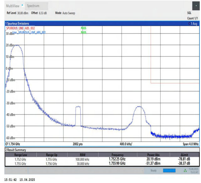
Band4-3MHz-QPSK-20385-1RB#0-PASS
