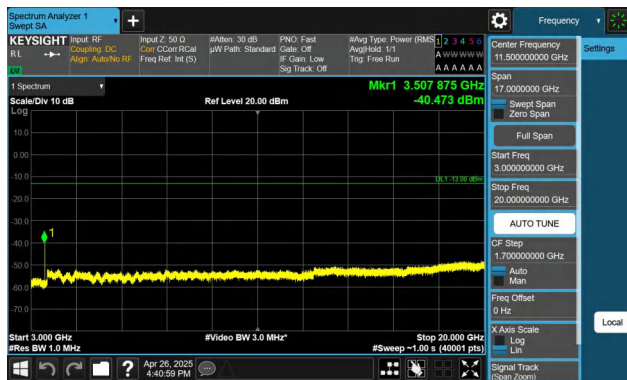
Band4-1.4MHz-QPSK-20393-1RB#0-3000~20000-PASS
