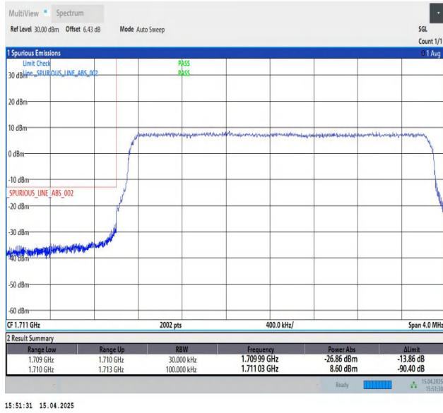
Band4-3MHz-QPSK-19965-15RB#0-PASS
