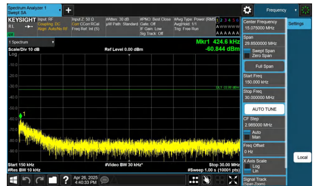
Band4-1.4MHz-QPSK-20393-1RB#0-0.15~30-PASS
