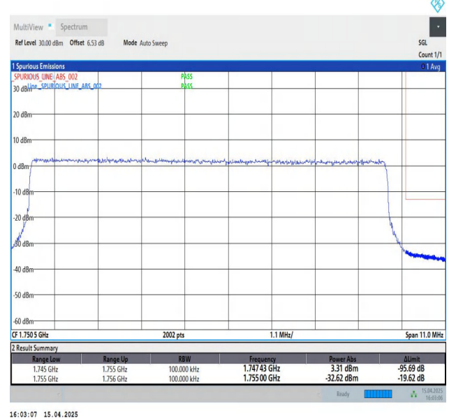
Band4-10MHz-QPSK-20350-50RB#0-PASS
