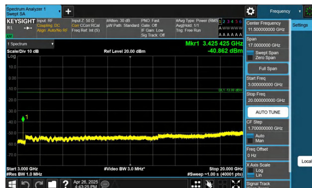
Band4-3MHz-QPSK-19965-1RB#14-3000~20000-PASS
