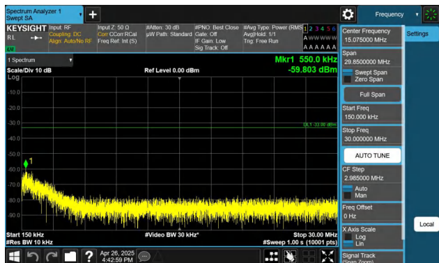
Band4-3MHz-QPSK-19965-1RB#14-0.15~30-PASS
