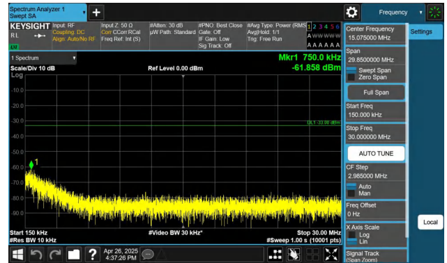
Band4-1.4MHz-QPSK-19957-1RB#0-0.15~30-PASS
