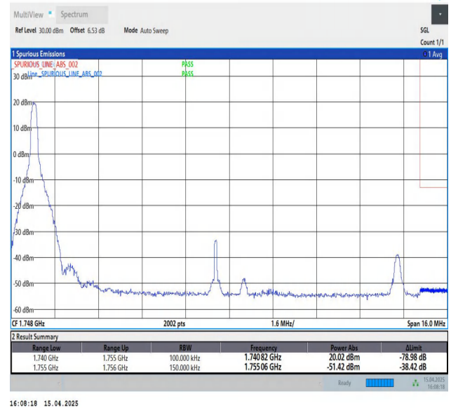
Band4-15MHz-QPSK-20325-1RB#0-PASS
