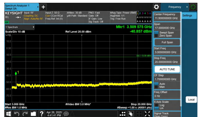
Band4-1.4MHz-QPSK-20393-1RB#5-3000~20000-PASS
