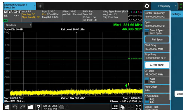
Band4-3MHz-QPSK-19965-1RB#14-30~1000-PASS
