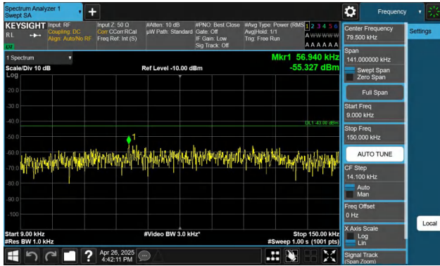
Band4-3MHz-QPSK-19965-1RB#0-0.009~0.15-PASS
