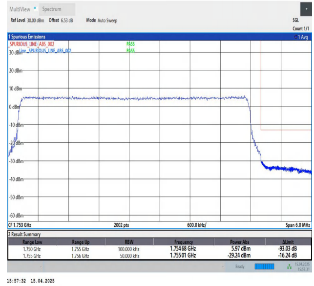
Band4-5MHz-QPSK-20375-25RB#0-PASS
