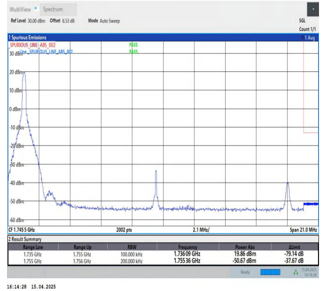
Band4-20MHz-QPSK-20300-1RB#0-PASS
