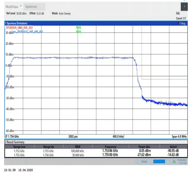
Band4-3MHz-QPSK-20385-15RB#0-PASS
