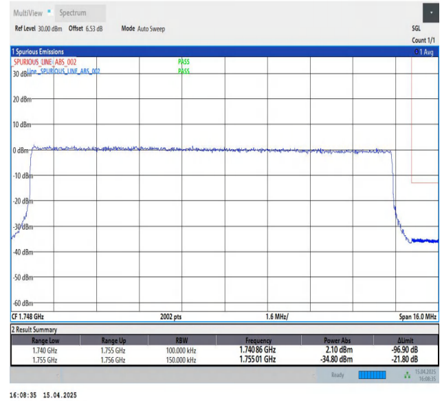
Band4-15MHz-QPSK-20325-75RB#0-PASS
