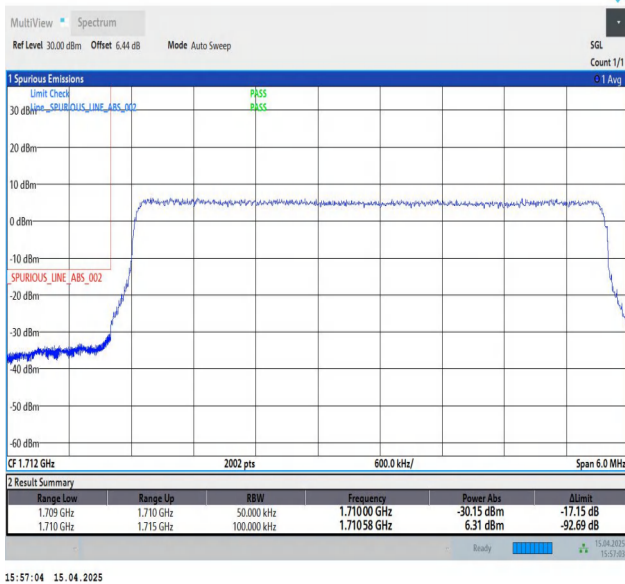
Band4-5MHz-QPSK-19975-25RB#0-PASS
