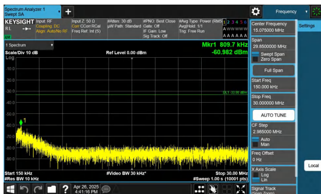
Band4-1.4MHz-QPSK-20393-1RB#5-0.15~30-PASS
