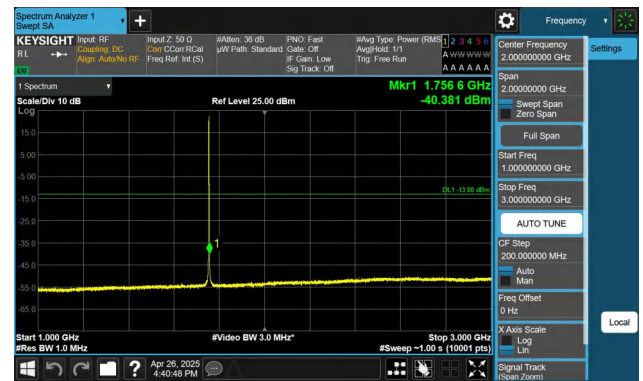
Band4-1.4MHz-QPSK-20393-1RB#0-1000~3000-PASS
