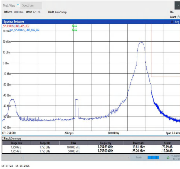
Band4-5MHz-QPSK-20375-1RB#24-PASS
