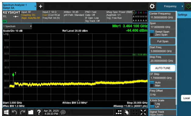
Band4-1.4MHz-QPSK-20175-1RB#0-3000~20000-PASS
