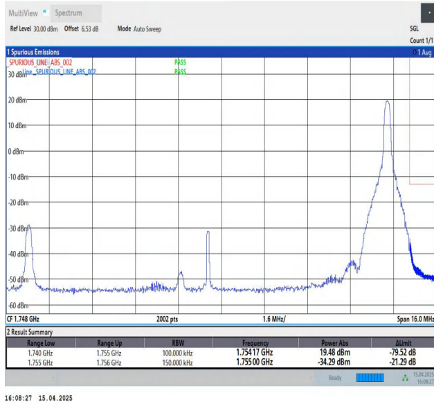
Band4-15MHz-QPSK-20325-1RB#74-PASS
