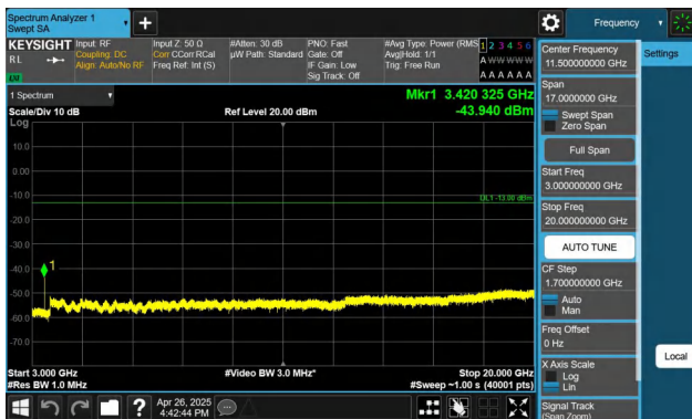
Band4-3MHz-QPSK-19965-1RB#0-3000~20000-PASS
