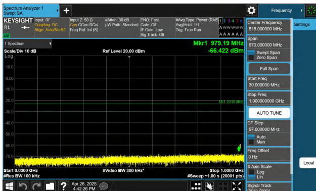
Band4-3MHz-QPSK-19965-1RB#0-30~1000-PASS
