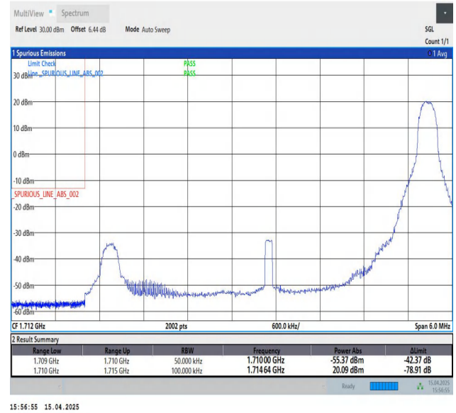
Band4-5MHz-QPSK-19975-1RB#24-PASS
