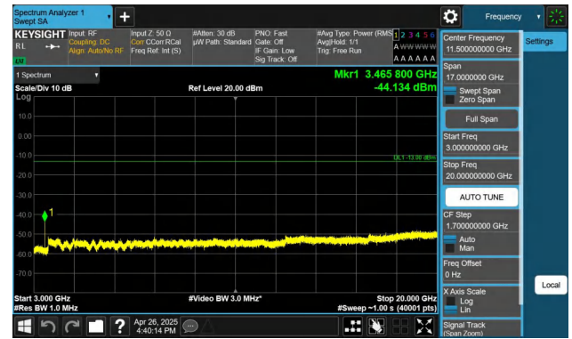
Band4-1.4MHz-QPSK-20175-1RB#5-3000~20000-PASS
