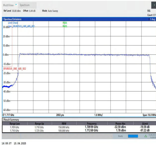
Band4-15MHz-QPSK-20025-75RB#0-PASS
