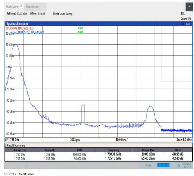
Band4-5MHz-QPSK-20375-1RB#0-PASS
