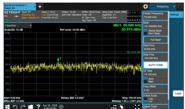
Band4-1.4MHz-QPSK-19957-1RB#5-0.009~0.15-PASS
