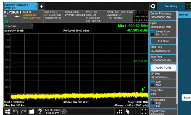
Band4-1.4MHz-QPSK-19957-1RB#5-30~1000-PASS
