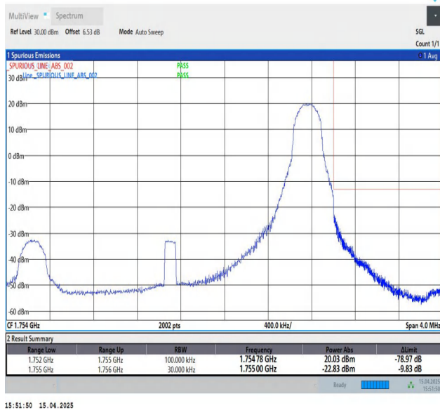
Band4-3MHz-QPSK-20385-1RB#14-PASS
