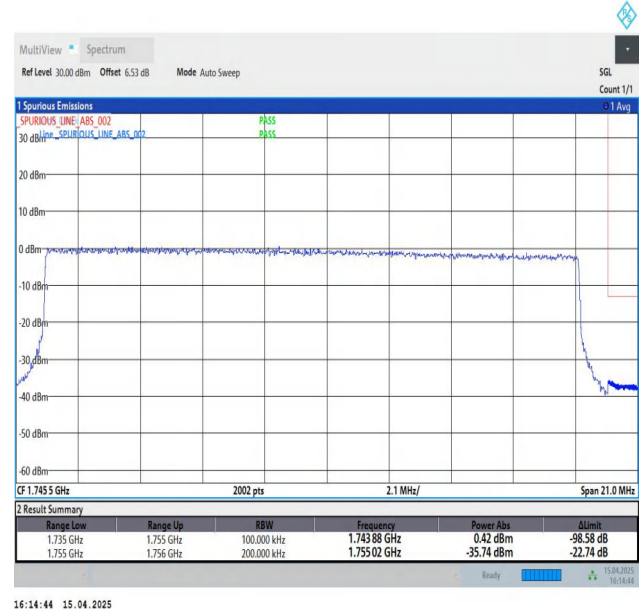
Band4-20MHz-QPSK-20300-100RB#0-PASS
