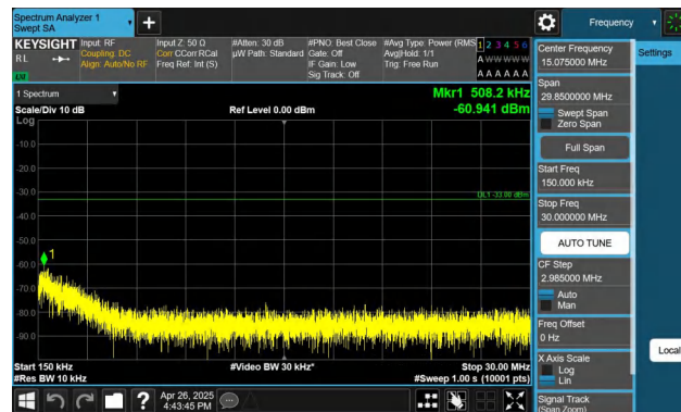
Band4-3MHz-QPSK-20175-1RB#0-0.15~30-PASS
