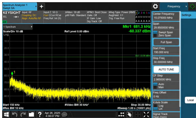
Band4-1.4MHz-QPSK-19957-1RB#5-0.15~30-PASS
