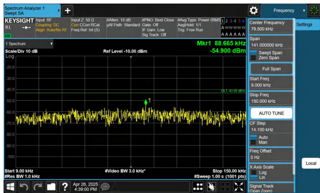
Band4-1.4MHz-QPSK-20175-1RB#0-0.009~0.15-PASS
