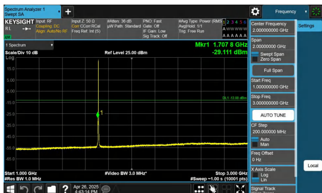
Band4-3MHz-QPSK-19965-1RB#14-1000~3000-PASS
