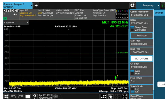
Band2-15MHz-QPSK-18675-1RB#74-30~1000-PASS
