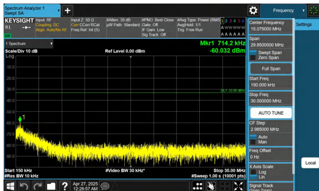
Band2-15MHz-QPSK-18675-1RB#74-0.15~30-PASS
