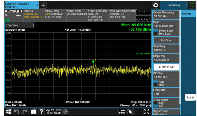
Band2-20MHz-QPSK-19100-1RB#99-0.009~0.15-PASS
