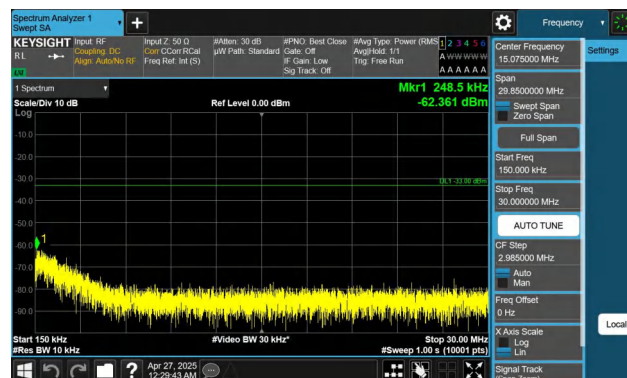
Band2-15MHz-QPSK-18900-1RB#0-0.15~30-PASS
