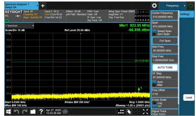
Band2-20MHz-QPSK-18700-1RB#99-30~1000-PASS
