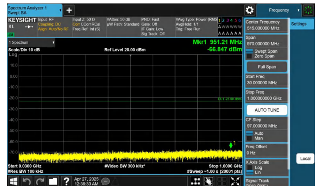
Band2-20MHz-QPSK-19100-1RB#99-30~1000-PASS
