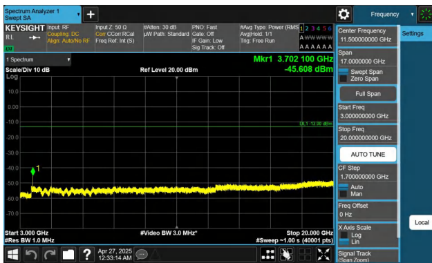
Band2-20MHz-QPSK-18700-1RB#0-3000~20000-PASS
