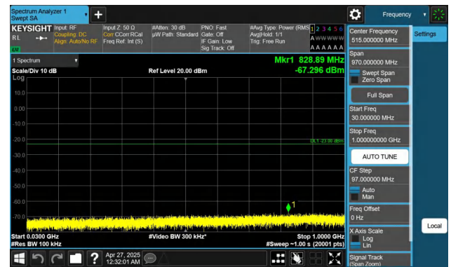
Band2-15MHz-QPSK-19125-1RB#74-30~1000-PASS
