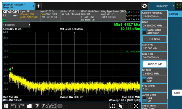
Band2-15MHz-QPSK-18900-1RB#74-0.15~30-PASS
