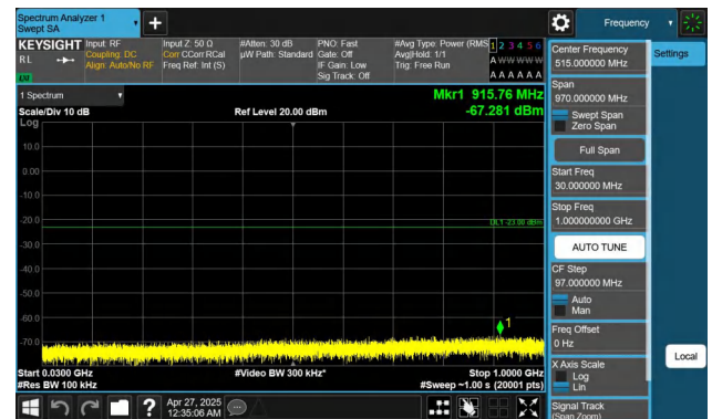
Band2-20MHz-QPSK-18900-1RB#99-30~1000-PASS
