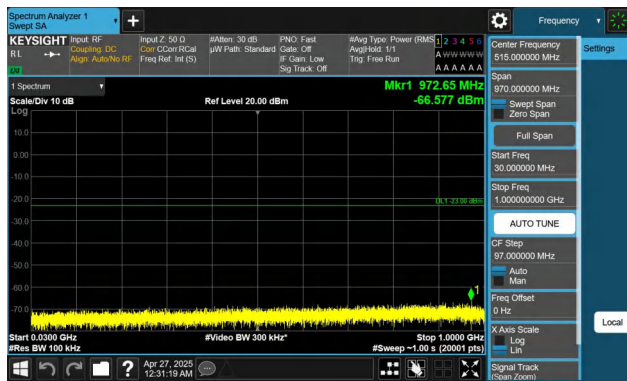
Band2-15MHz-QPSK-19125-1RB#0-30~1000-PASS
