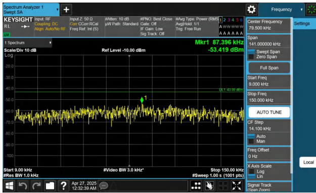
Band2-20MHz-QPSK-18700-1RB#0-0.009~0.15-PASS
