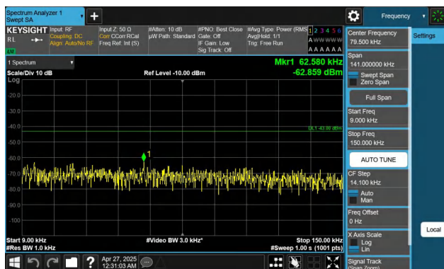
Band2-15MHz-QPSK-19125-1RB#0-0.009~0.15-PASS
