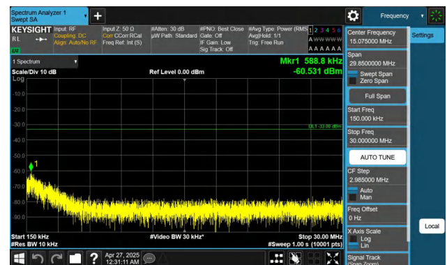
Band2-15MHz-QPSK-19125-1RB#0-0.15~30-PASS
