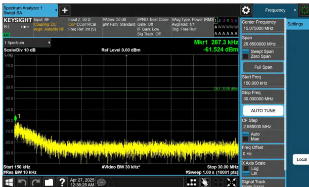
Band2-20MHz-QPSK-19100-1RB#99-0.15~30-PASS
