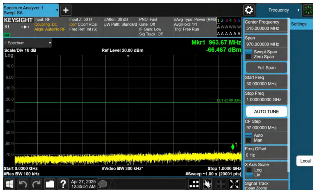
Band2-20MHz-QPSK-19100-1RB#0-30~1000-PASS
