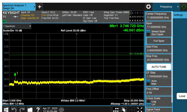
Band2-15MHz-QPSK-18900-1RB#0-3000~20000-PASS
