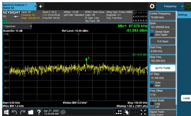
Band2-20MHz-QPSK-18900-1RB#0-0.009~0.15-PASS
