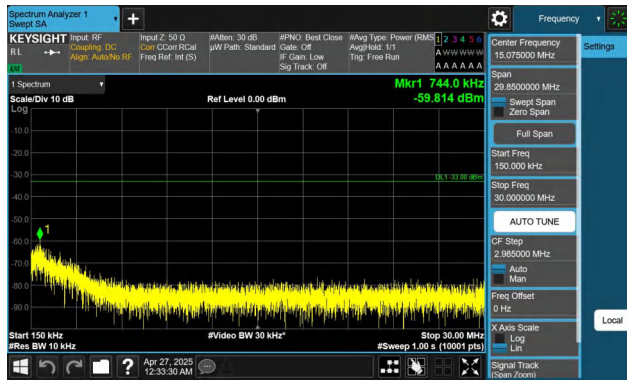
Band2-20MHz-QPSK-18700-1RB#99-0.15~30-PASS
