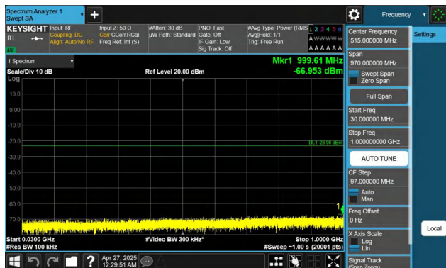
Band2-15MHz-QPSK-18900-1RB#0-30~1000-PASS
