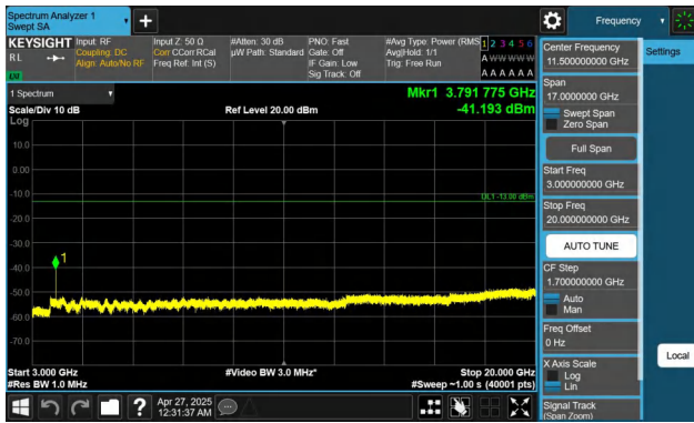
Band2-15MHz-QPSK-19125-1RB#0-3000~20000-PASS
