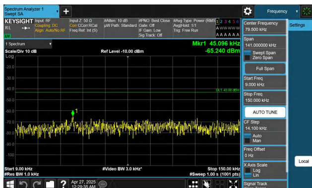
Band2-15MHz-QPSK-18900-1RB#0-0.009~0.15-PASS
