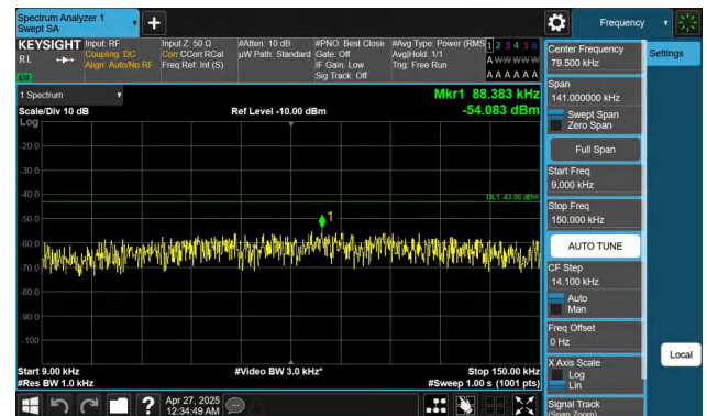
Band2-20MHz-QPSK-18900-1RB#99-0.009~0.15-PASS
