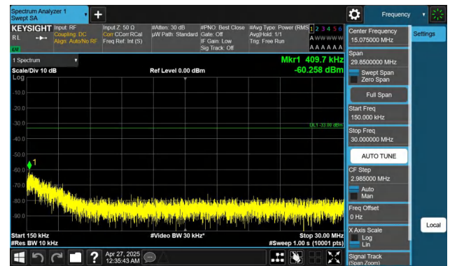
Band2-20MHz-QPSK-19100-1RB#0-0.15~30-PASS
