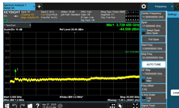
Band2-15MHz-QPSK-18675-1RB#74-3000~20000-PASS
