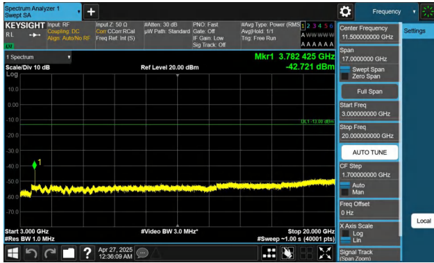
Band2-20MHz-QPSK-19100-1RB#0-3000~20000-PASS
