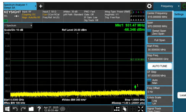
Band2-15MHz-QPSK-18900-1RB#74-30~1000-PASS
