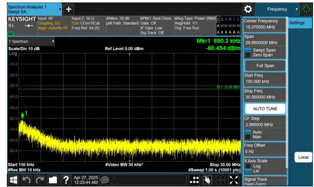
Band2-10MHz-QPSK-18650-1RB#0-0.15~30-PASS
