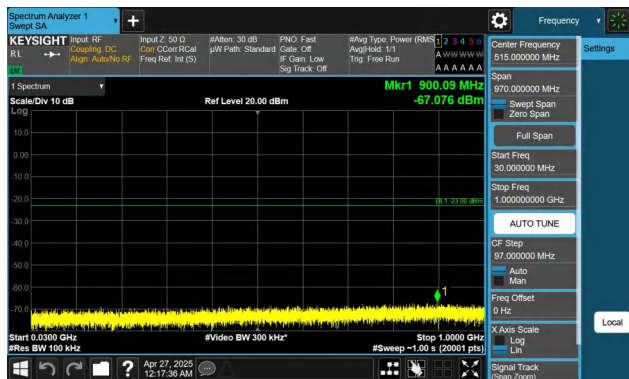
Band2-3MHz-QPSK-19185-1RB#0-30~1000-PASS
