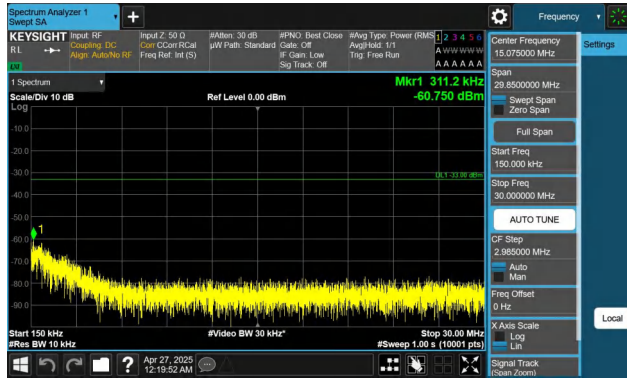
Band2-5MHz-QPSK-18625-1RB#24-0.15~30-PASS
