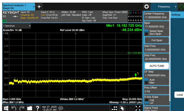
Band2-10MHz-QPSK-18900-1RB#0-3000~20000-PASS
