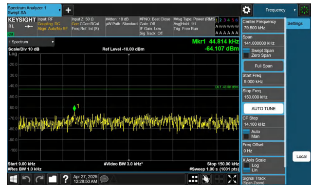
Band2-15MHz-QPSK-18675-1RB#74-0.009~0.15-PASS
