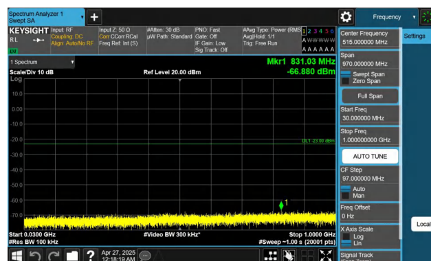
Band2-3MHz-QPSK-19185-1RB#14-30~1000-PASS
