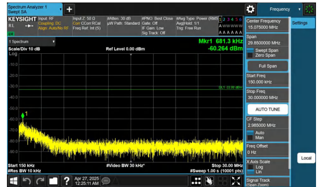
Band2-10MHz-QPSK-18900-1RB#0-0.15~30-PASS
