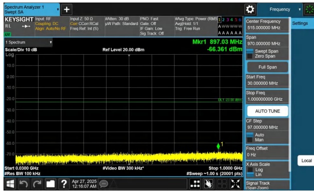
Band2-3MHz-QPSK-18900-1RB#0-30~1000-PASS
