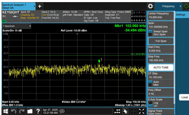
Band2-5MHz-QPSK-19175-1RB#0-0.009~0.15-PASS
