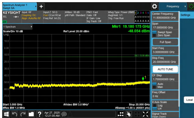
Band2-5MHz-QPSK-18900-1RB#0-3000~20000-PASS
