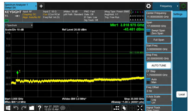
Band2-5MHz-QPSK-19175-1RB#24-3000~20000-PASS
