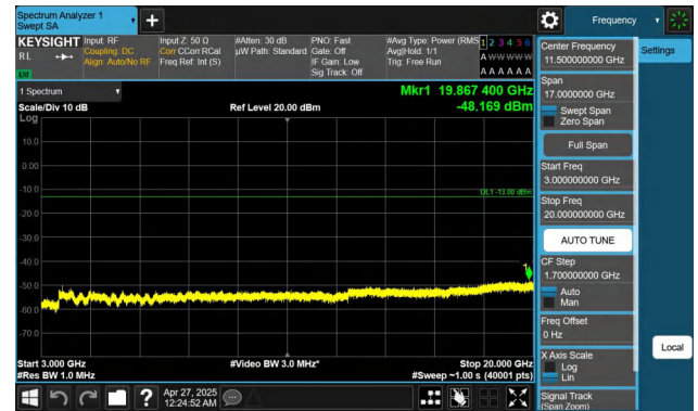
Band2-10MHz-QPSK-18650-1RB#49-3000~20000-PASS
