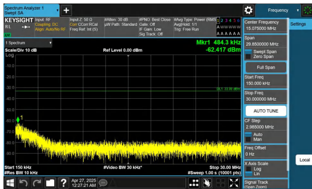
Band2-10MHz-QPSK-19150-1RB#49-0.15~30-PASS
