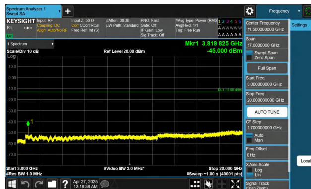
Band2-3MHz-QPSK-19185-1RB#14-3000~20000-PASS
