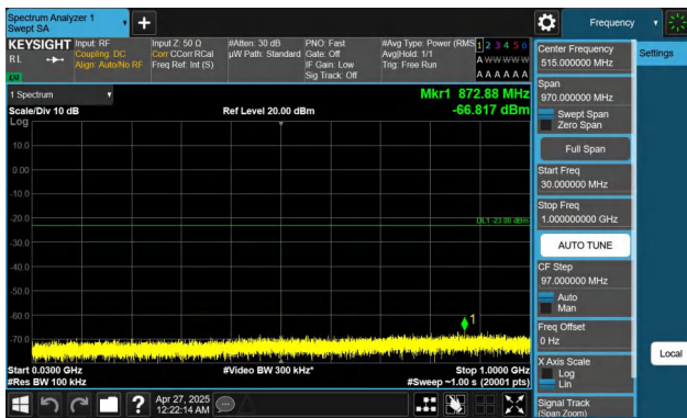
Band2-5MHz-QPSK-19175-1RB#0-30~1000-PASS
