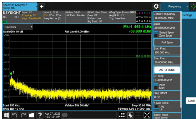
Band2-5MHz-QPSK-18900-1RB#24-0.15~30-PASS
