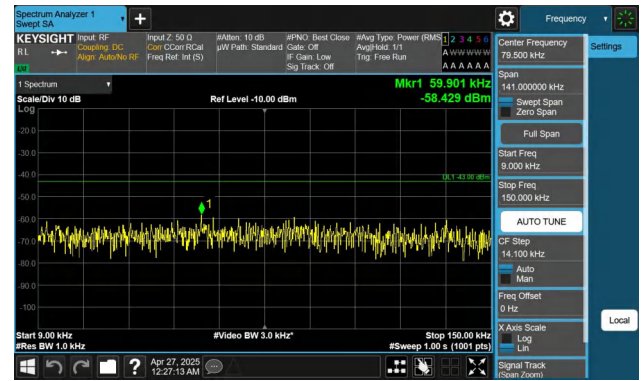
Band2-10MHz-QPSK-19150-1RB#49-0.009~0.15-PASS
