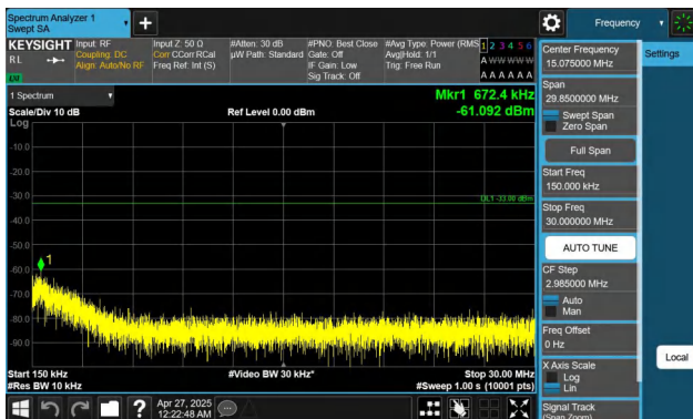
Band2-5MHz-QPSK-19175-1RB#24-0.15~30-PASS
