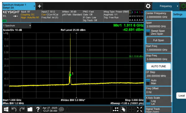
Band2-10MHz-QPSK-19150-1RB#49-1000~3000-PASS
