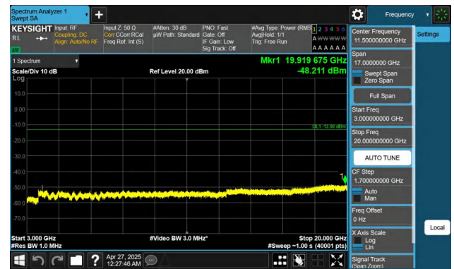
Band2-10MHz-QPSK-19150-1RB#49-3000~20000-PASS
