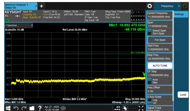
Band2-5MHz-QPSK-18625-1RB#24-3000~20000-PASS
