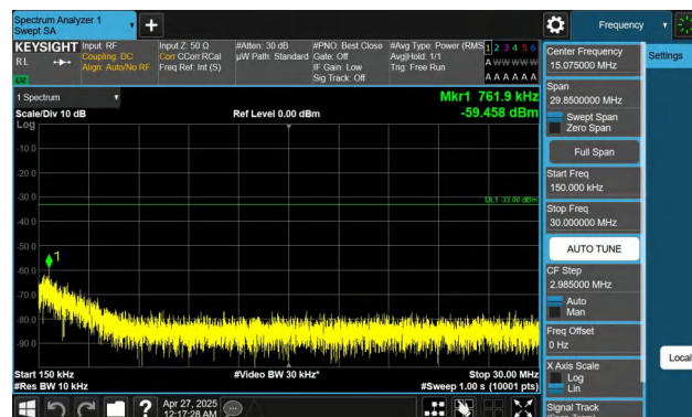
Band2-3MHz-QPSK-19185-1RB#0-0.15~30-PASS
