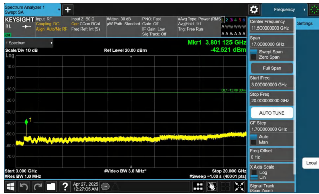
Band2-10MHz-QPSK-19150-1RB#0-3000~20000-PASS
