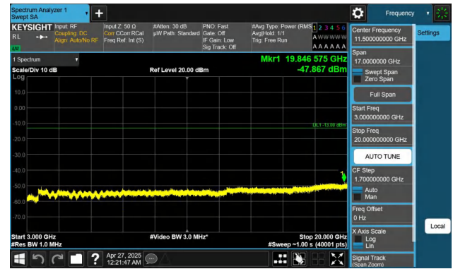
Band2-5MHz-QPSK-18900-1RB#24-3000~20000-PASS
