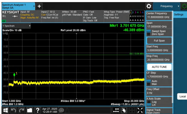
Band2-15MHz-QPSK-18675-1RB#0-3000~20000-PASS
