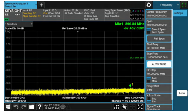
Band2-10MHz-QPSK-18650-1RB#49-30~1000-PASS
