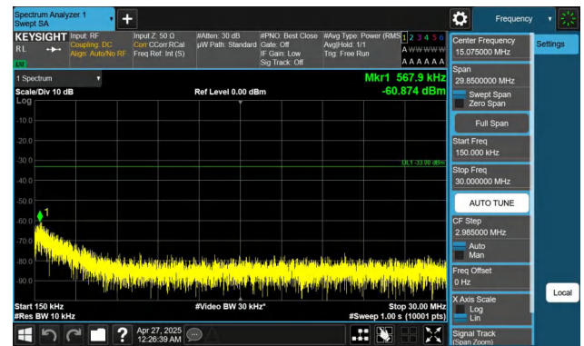
Band2-10MHz-QPSK-19150-1RB#0-0.15~30-PASS
