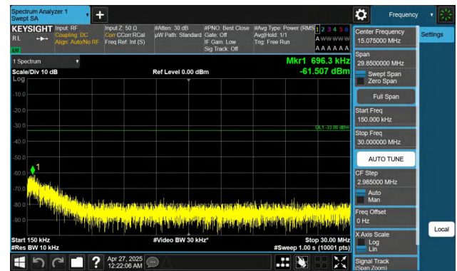
Band2-5MHz-QPSK-19175-1RB#0-0.15~30-PASS
