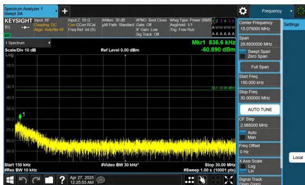
Band2-10MHz-QPSK-18900-1RB#49-0.15~30-PASS
