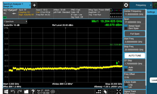
Band2-3MHz-QPSK-18900-1RB#14-3000~20000-PASS
