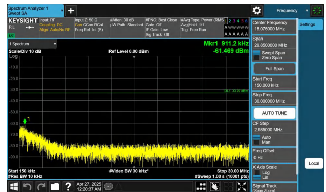
Band2-5MHz-QPSK-18900-1RB#0-0.15~30-PASS
