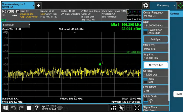
Band2-15MHz-QPSK-18675-1RB#0-0.009~0.15-PASS
