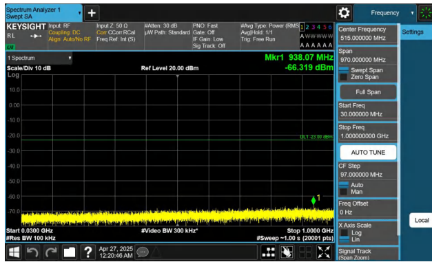
Band2-5MHz-QPSK-18900-1RB#0-30~1000-PASS
