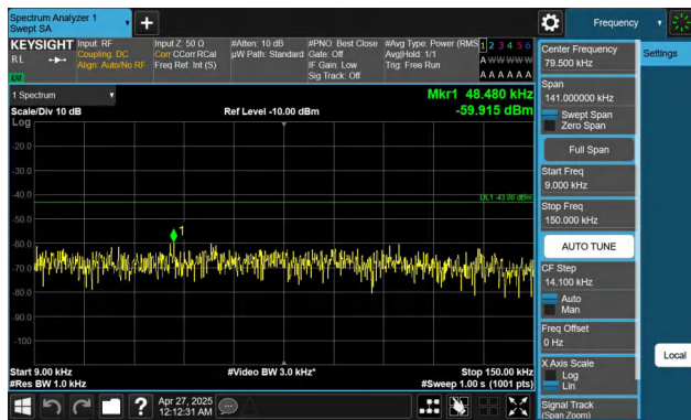
Band2-1.4MHz-QPSK-19193-1RB#0-0.009~0.15-PASS
