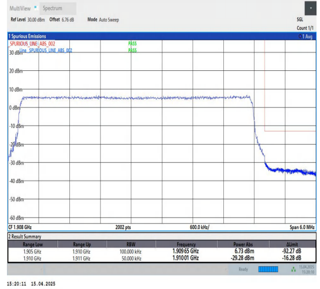
Band2-5MHz-QPSK-19175-25RB#0-PASS
