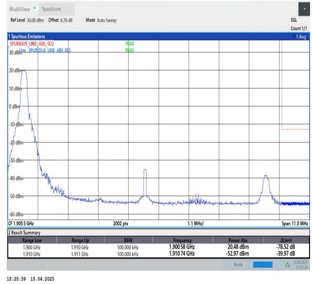
Band2-10MHz-QPSK-19150-1RB#0-PASS
