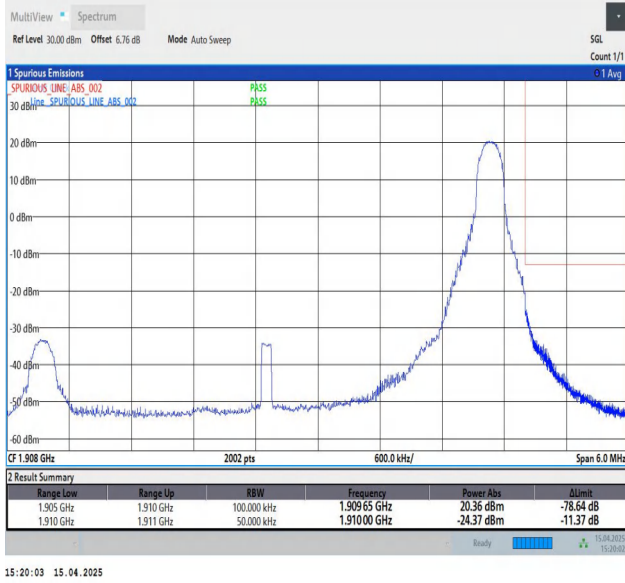
Band2-5MHz-QPSK-19175-1RB#24-PASS
