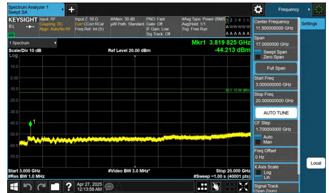
Band2-1.4MHz-QPSK-19193-1RB#5-3000~20000-PASS
