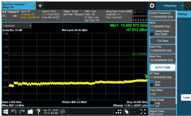
Band2-3MHz-QPSK-18615-1RB#0-3000~20000-PASS
