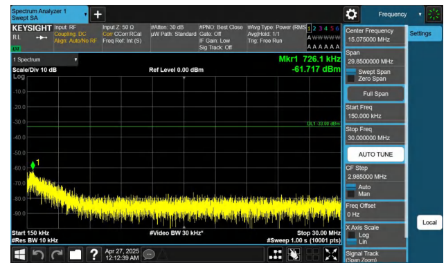
Band2-1.4MHz-QPSK-19193-1RB#0-0.15~30-PASS
