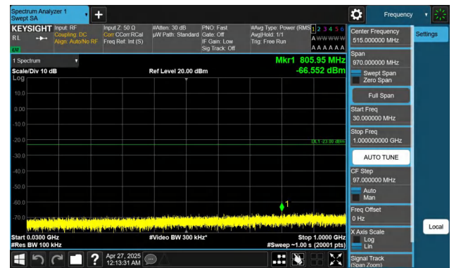
Band2-1.4MHz-QPSK-19193-1RB#5-30~1000-PASS
