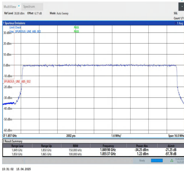
Band2-15MHz-QPSK-18675-75RB#0-PASS
