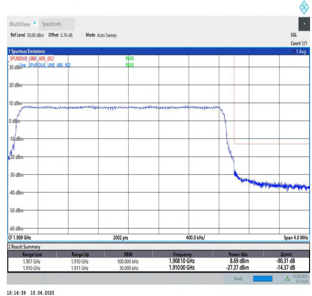
Band2-3MHz-QPSK-19185-15RB#0-PASS
