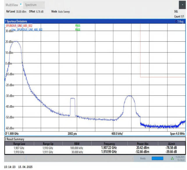
Band2-3MHz-QPSK-19185-1RB#0-PASS
