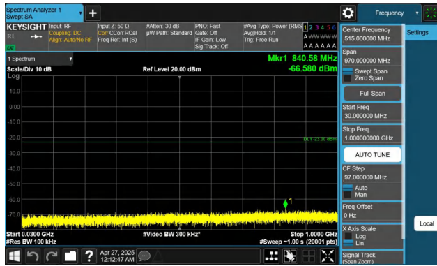
Band2-1.4MHz-QPSK-19193-1RB#0-30~1000-PASS
