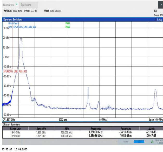
Band2-15MHz-QPSK-18675-1RB#0-PASS
