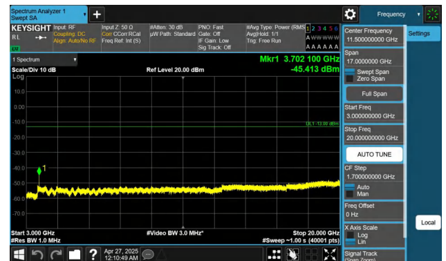
Band2-1.4MHz-QPSK-18607-1RB#5-3000~20000-PASS
