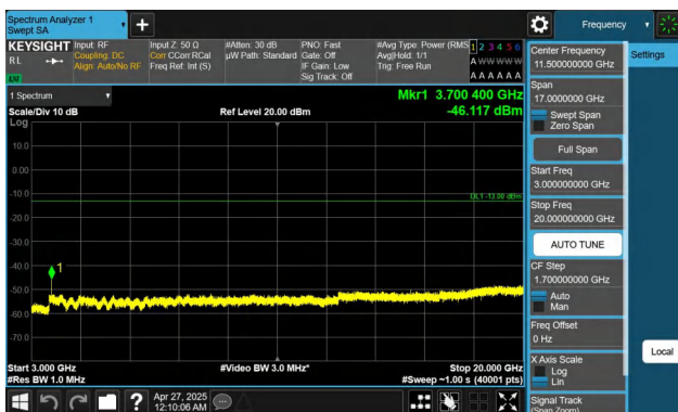
Band2-1.4MHz-QPSK-18607-1RB#0-3000~20000-PASS
