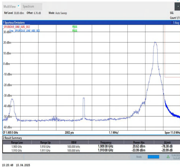
Band2-10MHz-QPSK-19150-1RB#49-PASS
