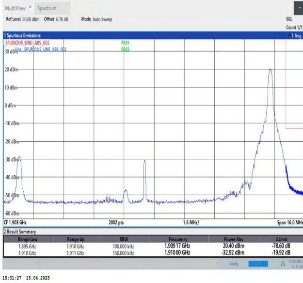
Band2-15MHz-QPSK-19125-1RB#74-PASS
