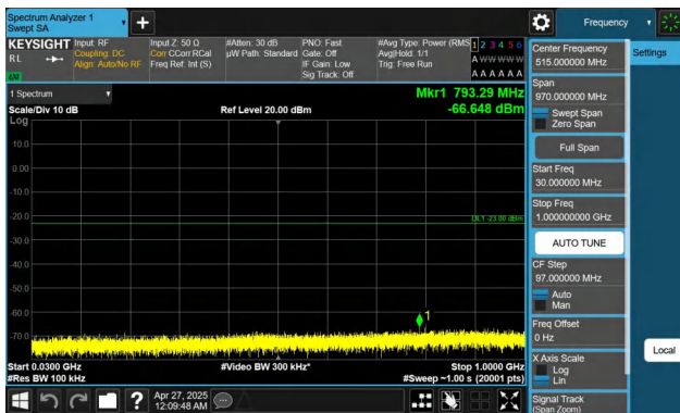
Band2-1.4MHz-QPSK-18607-1RB#0-30~1000-PASS
