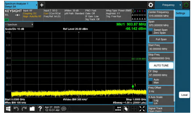
Band2-1.4MHz-QPSK-18607-1RB#5-30~1000-PASS
