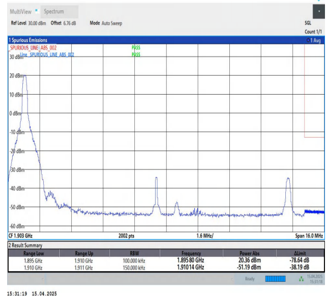
Band2-15MHz-QPSK-19125-1RB#0-PASS
