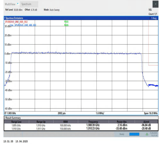
Band2-15MHz-QPSK-19125-75RB#0-PASS
