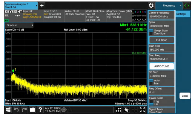
Band2-3MHz-QPSK-18615-1RB#0-0.15~30-PASS
