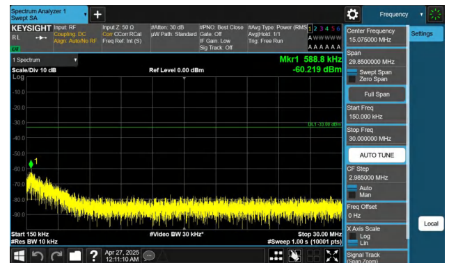
Band2-1.4MHz-QPSK-18900-1RB#0-0.15~30-PASS
