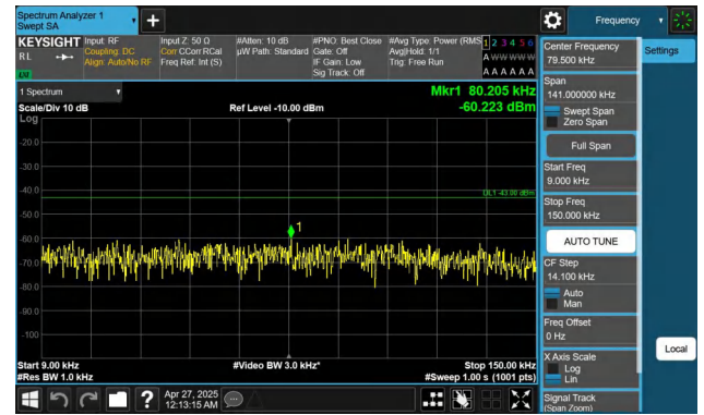
Band2-1.4MHz-QPSK-19193-1RB#5-0.009~0.15-PASS
