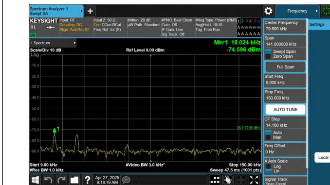
Band48-20MHz-QPSK-56640-1RB#0-0.009~0.15-PASS
