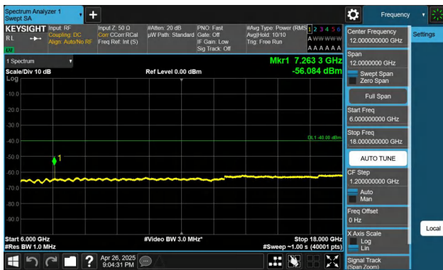
Band48-15MHz-QPSK-55990-1RB#74-6000~18000-PASS
