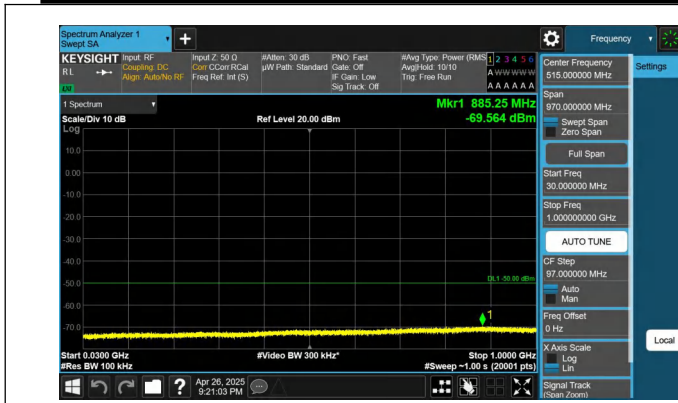
Band48-20MHz-QPSK-56640-1RB#0-30~1000-PASS
