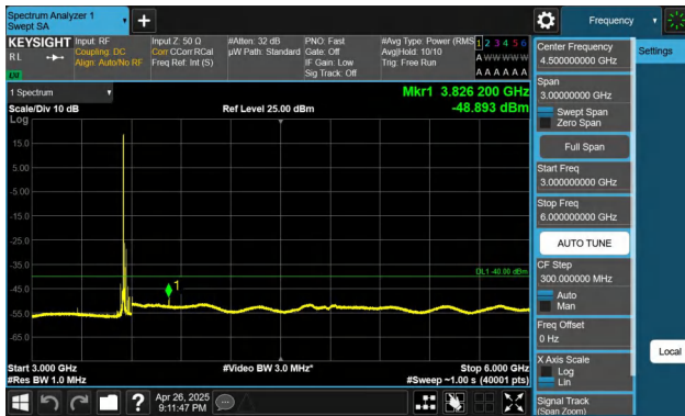
Band48-20MHz-QPSK-55340-1RB#0-3000~6000-PASS
