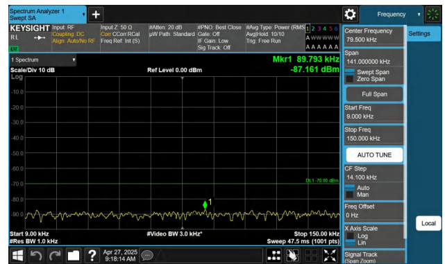
Band48-20MHz-QPSK-55990-1RB#99-0.009~0.15-PASS
