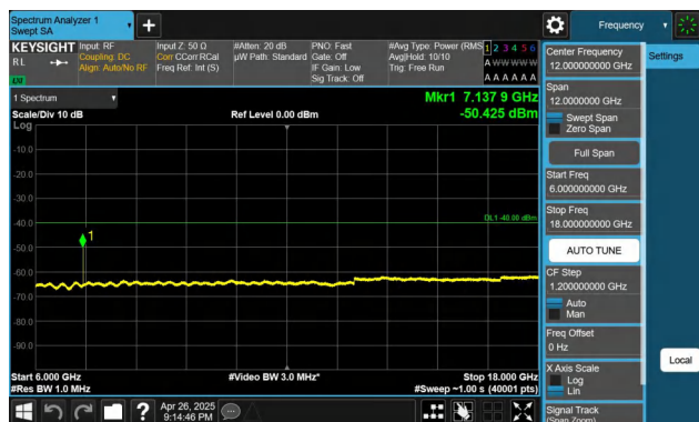
Band48-20MHz-QPSK-55340-1RB#99-6000~18000-PASS
