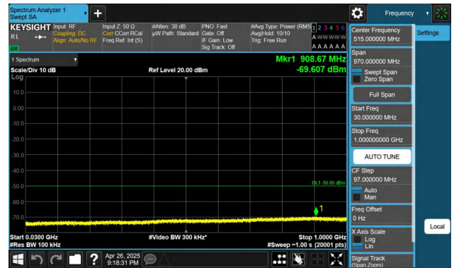
Band48-20MHz-QPSK-55990-1RB#99-30~1000-PASS
