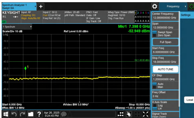
Band48-20MHz-QPSK-56640-1RB#99-6000~18000-PASS
