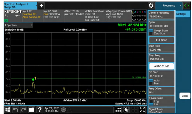
Band48-20MHz-QPSK-55340-1RB#99-0.009~0.15-PASS
