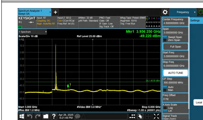
Band48-20MHz-QPSK-56640-1RB#0-3000~6000-PASS
