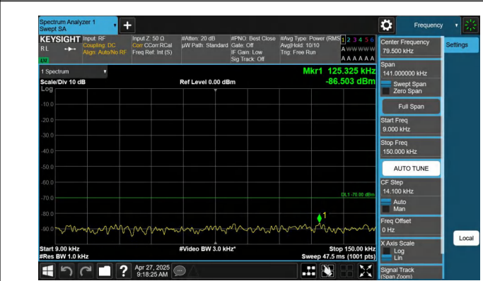
Band48-20MHz-QPSK-56640-1RB#99-0.009~0.15-PASS
