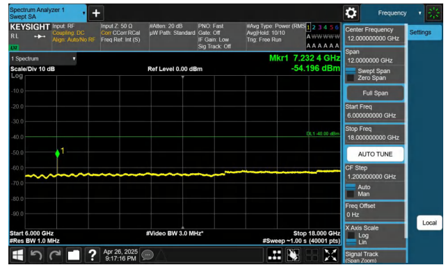
Band48-20MHz-QPSK-55990-1RB#0-6000~18000-PASS
