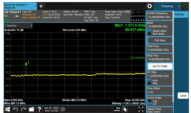
Band48-15MHz-QPSK-56665-1RB#0-6000~18000-PASS
