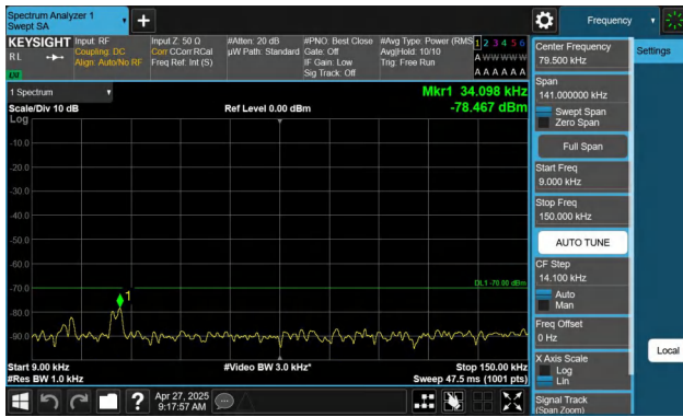
Band48-20MHz-QPSK-55340-1RB#0-0.009~0.15-PASS
