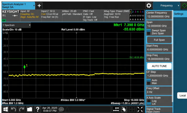
Band48-15MHz-QPSK-56665-1RB#74-6000~18000-PASS
