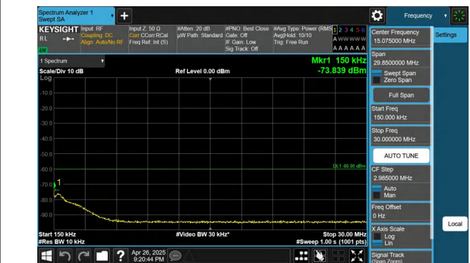
Band48-20MHz-QPSK-56640-1RB#0-0.15~30-PASS
