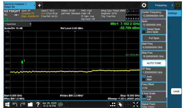
Band48-20MHz-QPSK-55340-1RB#0-6000~18000-PASS
