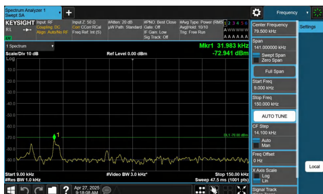
Band48-20MHz-QPSK-55990-1RB#0-0.009~0.15-PASS
