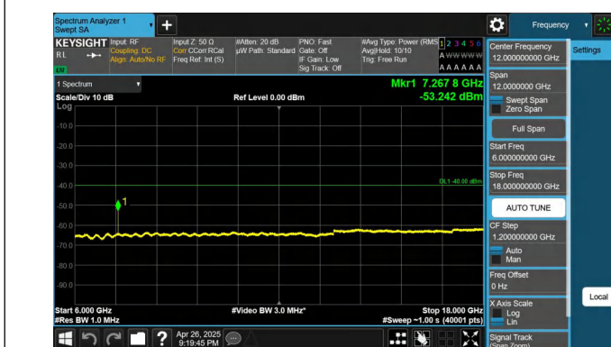
Band48-20MHz-QPSK-55990-1RB#99-6000~18000-PASS
