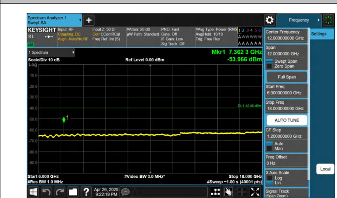
Band48-20MHz-QPSK-56640-1RB#0-6000~18000-PASS
