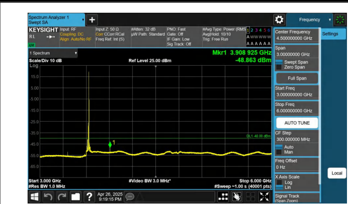
Band48-20MHz-QPSK-55990-1RB#99-3000~6000-PASS
