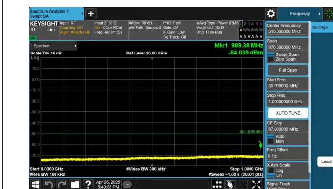
Band48-10MHz-QPSK-55290-1RB#0-30~1000-PASS
