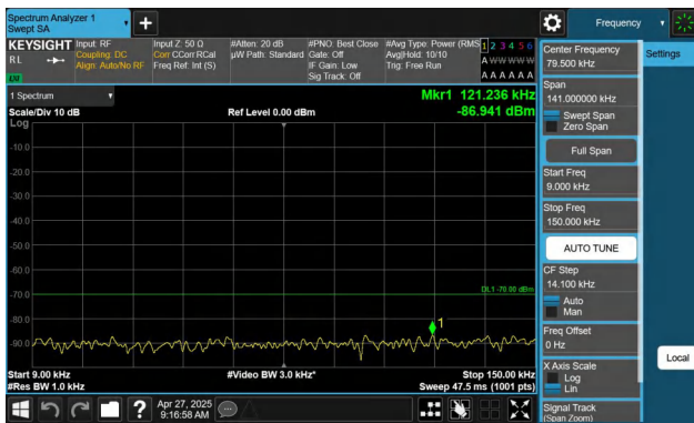
Band48-10MHz-QPSK-55990-1RB#0-0.009~0.15-PASS
