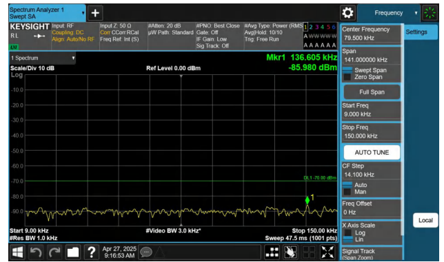
Band48-10MHz-QPSK-55290-1RB#49-0.009~0.15-PASS
