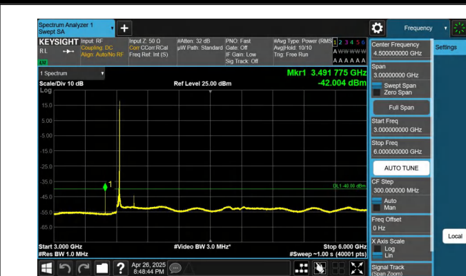
Band48-10MHz-QPSK-55990-1RB#49-3000~6000-PASS
