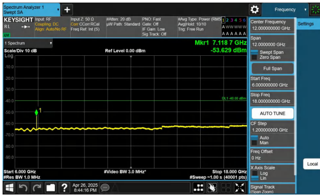
Band48-10MHz-QPSK-55290-1RB#49-6000~18000-PASS
