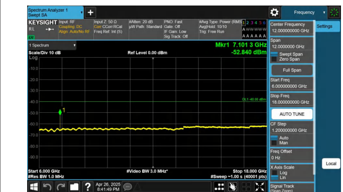
Band48-10MHz-QPSK-55290-1RB#0-6000~18000-PASS
