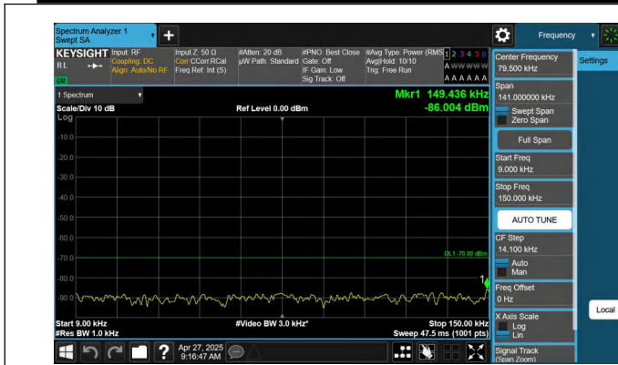
Band48-10MHz-QPSK-55290-1RB#0-0.009~0.15-PASS
