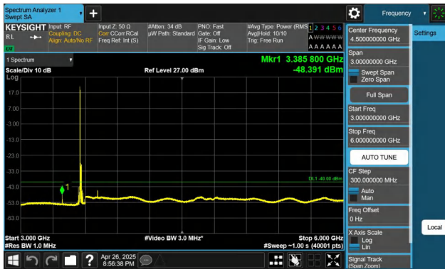
Band48-15MHz-QPSK-55315-1RB#0-3000~6000-PASS
