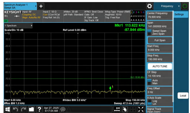
Band48-10MHz-QPSK-55990-1RB#49-0.009~0.15-PASS
