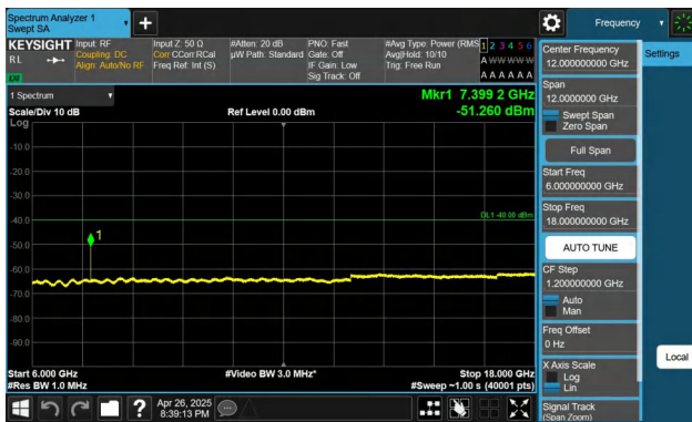
Band48-5MHz-QPSK-56715-1RB#24-6000~18000-PASS
