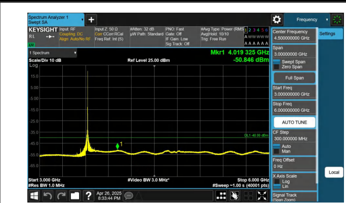
Band48-5MHz-QPSK-55990-1RB#24-3000~6000-PASS
