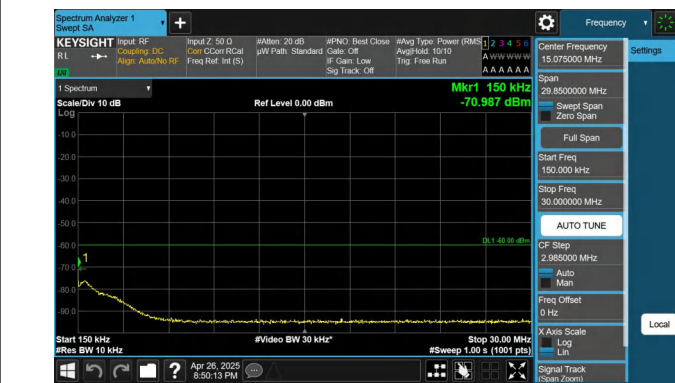
Band48-10MHz-QPSK-56690-1RB#0-0.15~30-PASS
