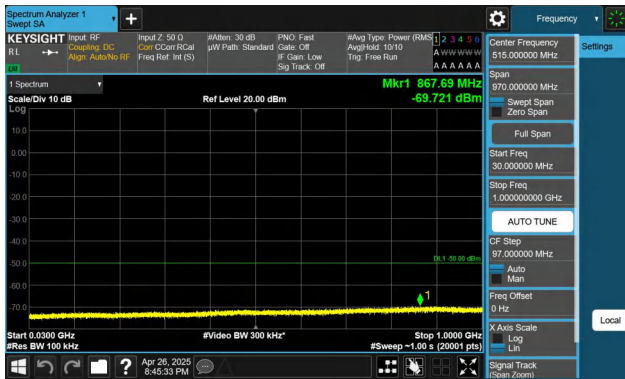
Band48-10MHz-QPSK-55990-1RB#0-30~1000-PASS
