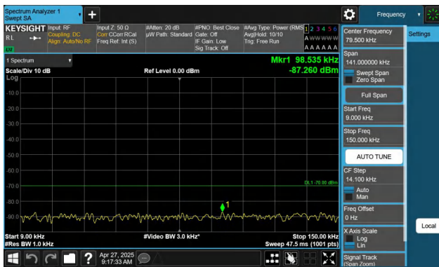
Band48-15MHz-QPSK-55990-1RB#0-0.009~0.15-PASS
