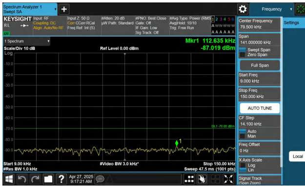
Band48-15MHz-QPSK-55315-1RB#0-0.009~0.15-PASS
