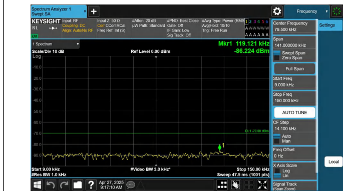
Band48-10MHz-QPSK-56690-1RB#0-0.009~0.15-PASS
