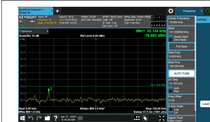
Band48-5MHz-QPSK-56715-1RB#0-0.009~0.15-PASS
