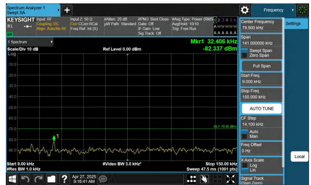
Band48-5MHz-QPSK-56715-1RB#24-0.009~0.15-PASS
