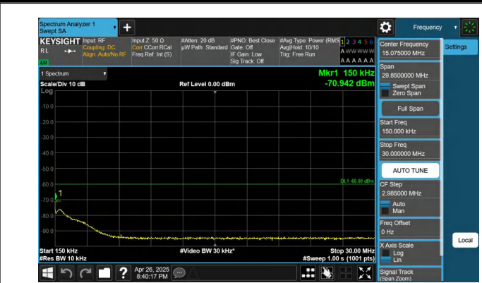
Band48-10MHz-QPSK-55290-1RB#0-0.15~30-PASS
