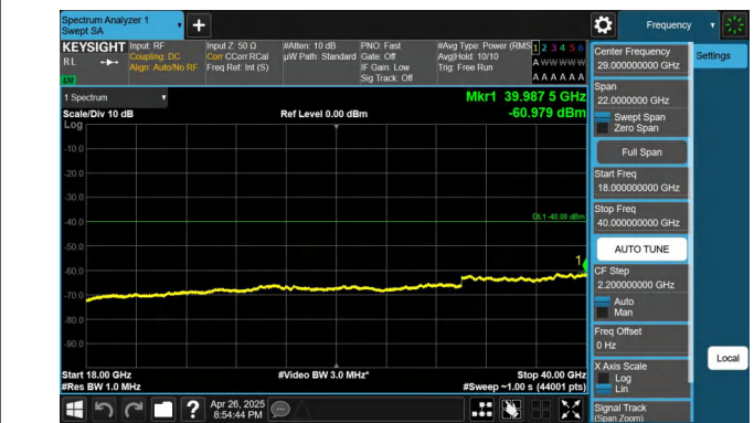
Band48-10MHz-QPSK-56690-1RB#49-18000~40000-PASS
