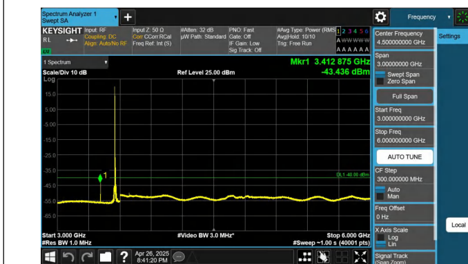
Band48-10MHz-QPSK-55290-1RB#0-3000~6000-PASS
