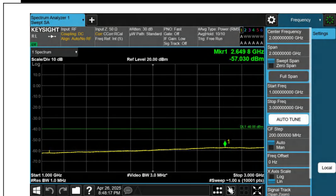
Band48-10MHz-QPSK-55990-1RB#49-1000~3000-PASS
