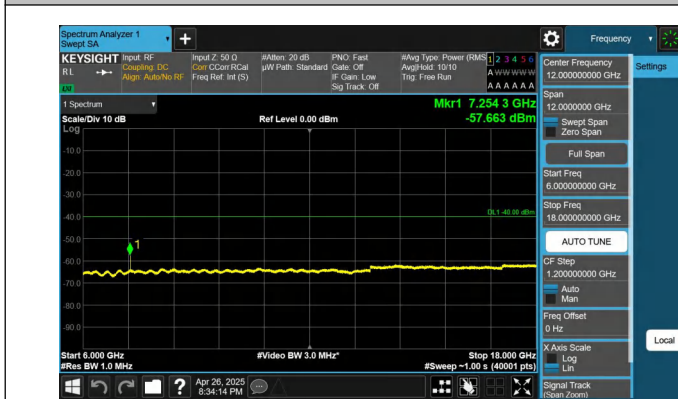
Band48-5MHz-QPSK-55990-1RB#24-6000~18000-PASS
