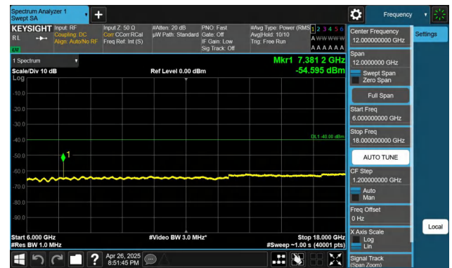
Band48-10MHz-QPSK-56690-1RB#0-6000~18000-PASS
