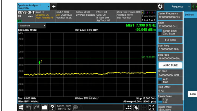
Band48-10MHz-QPSK-56690-1RB#49-6000~18000-PASS
