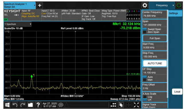
Band48-15MHz-QPSK-55315-1RB#74-0.009~0.15-PASS
