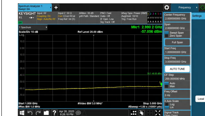
Band48-5MHz-QPSK-55265-1RB#24-1000~3000-PASS
