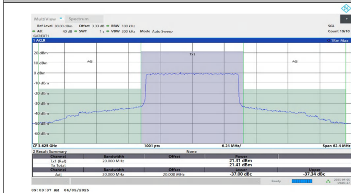
Band48-20MHz-16QAM-55990-100RB#0-PASS
