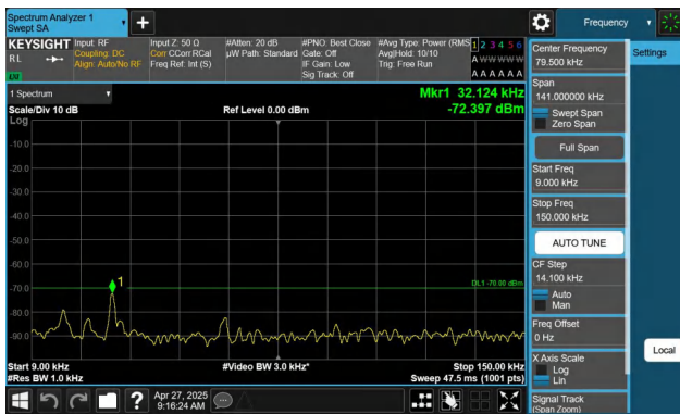
Band48-5MHz-QPSK-55990-1RB#0-0.009~0.15-PASS
