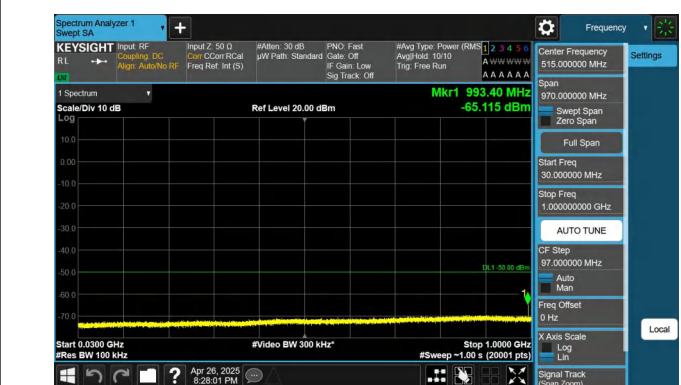
Band48-5MHz-QPSK-55265-1RB#24-30~1000-PASS
