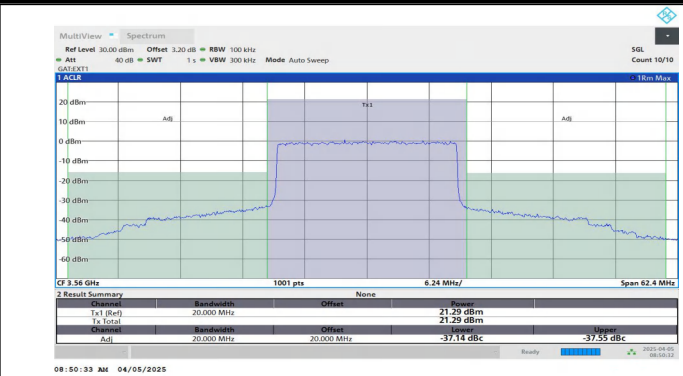
Band48-20MHz-16QAM-55340-100RB#0-PASS
