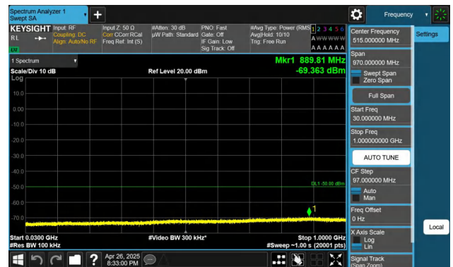
Band48-5MHz-QPSK-55990-1RB#24-30~1000-PASS
