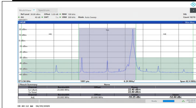
Band48-20MHz-16QAM-55340-1RB#99-PASS
