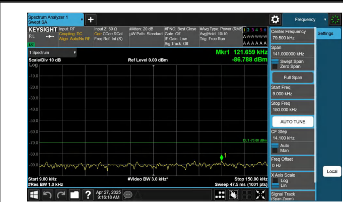
Band48-5MHz-QPSK-55265-1RB#24-0.009~0.15-PASS
