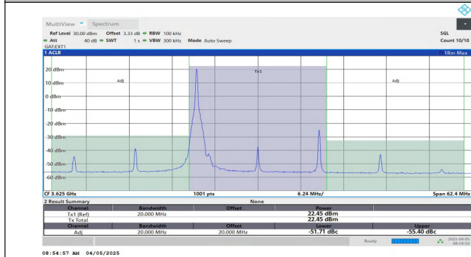
Band48-20MHz-16QAM-55990-1RB#0-PASS
