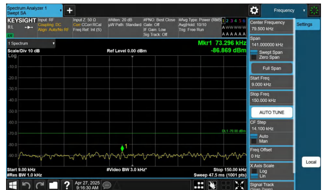
Band48-5MHz-QPSK-55990-1RB#24-0.009~0.15-PASS
