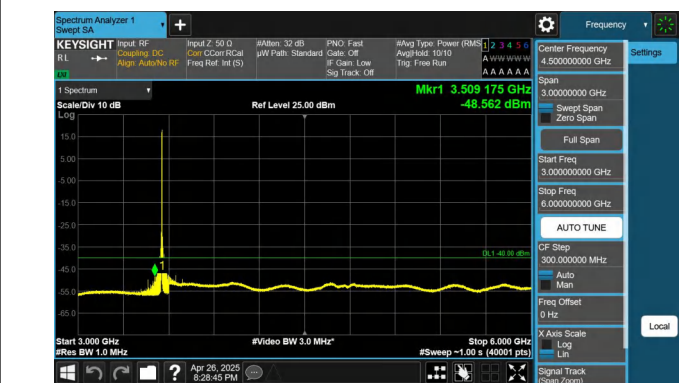
Band48-5MHz-QPSK-55265-1RB#24-3000~6000-PASS
