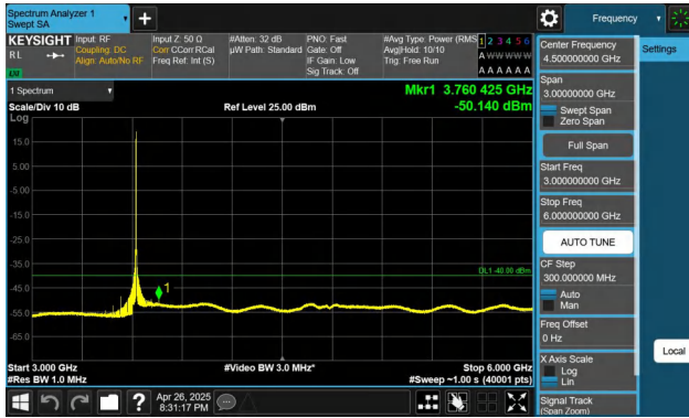
Band48-5MHz-QPSK-55990-1RB#0-3000~6000-PASS
