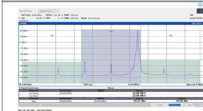
Band48-20MHz-16QAM-56640-1RB#0-PASS
