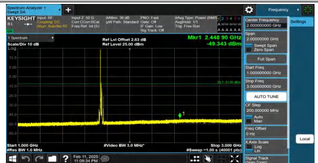
Band66-15MHz-QPSK-132322-1RB#0-1000~3000-PASS
