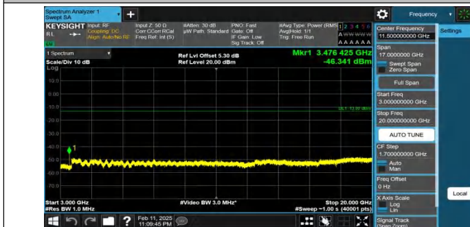
Band66-15MHz-QPSK-132322-1RB#0-3000~20000-PASS
