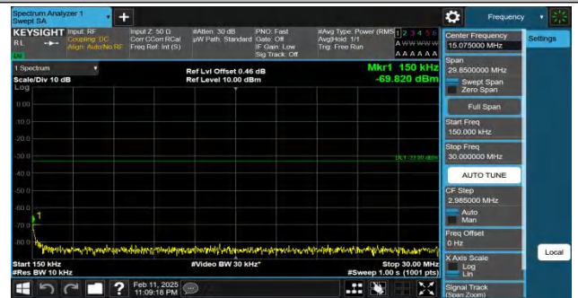
Band66-15MHz-QPSK-132322-1RB#0-0.15~30-PASS
