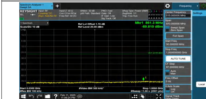
Band66-15MHz-QPSK-132322-1RB#0-0.30~1000-PASS
