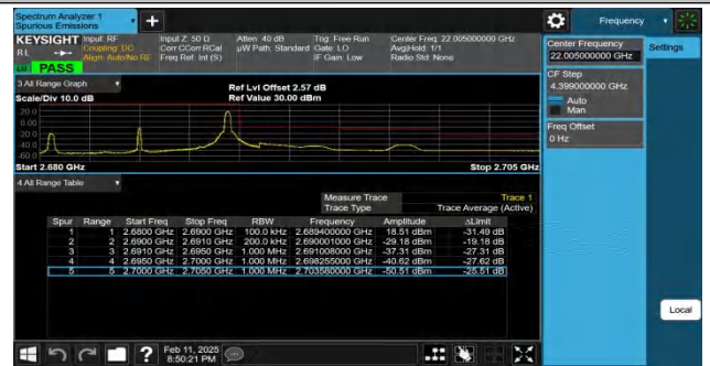
Band41-10MHz-QPSK-41540-1RB#49-PASS
