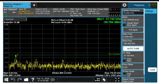
Band41-15MHz-QPSK-39725-1RB#74-0.009~0.15-PASS
