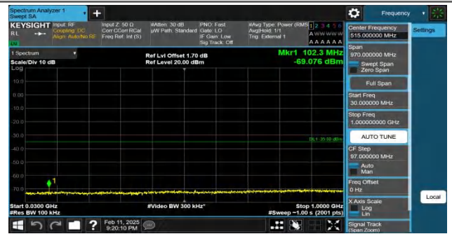
Band41-15MHz-QPSK-39725-1RB#74-30~1000-PASS
