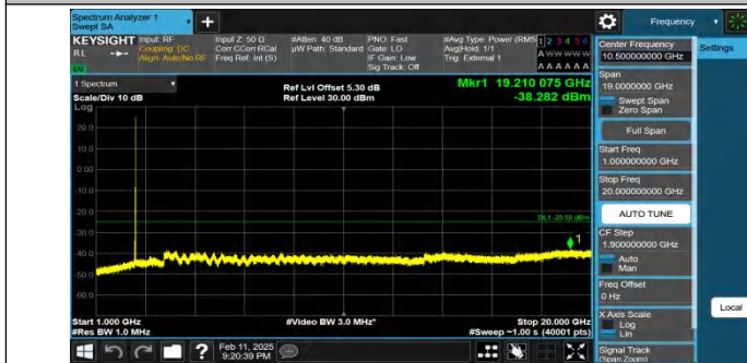
Band41-15MHz-QPSK-39725-1RB#74-1000~20000-PASS
