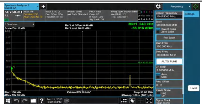
Band41-15MHz-QPSK-40620-1RB#0-0.15~30-PASS
