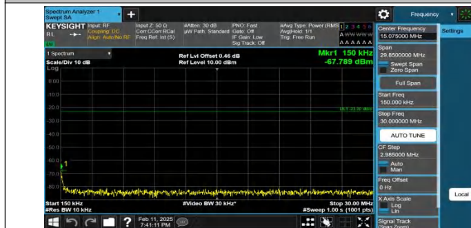
Band26(824-849)-3MHz-QPSK-26915-1RB#14-0.15~30-PASS
