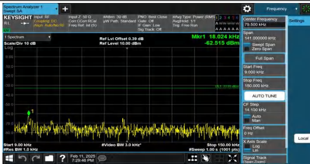
Band26(824-849)-1.4MHz-QPSK-26915-1RB#0-0.009~0.15-PASS
