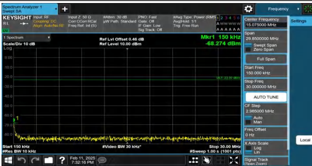
Band26(824-849)-1.4MHz-QPSK-27033-1RB#5-0.15~30-PASS
