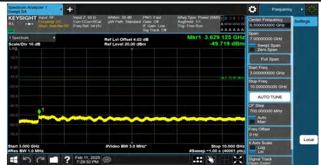
Band26(824-849)-1.4MHz-QPSK-26797-1RB#5-3000~10000-PASS S
