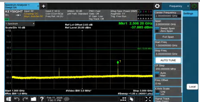
Band26(824-849)-1.4MHz-QPSK-26915-1RB#0-1000~3000-PASS
