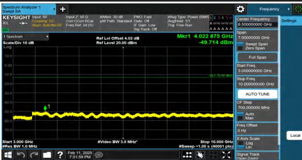
Band26(824-849)-1.4MHz-QPSK-27033-1RB#0-3000~10000-PAS
