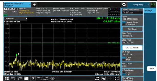
Band26(824-849)-1.4MHz-QPSK-27033-1RB#5-0.009~0.15-PASS
