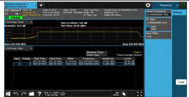
Band26(824-849)-5MHz-QPSK-26815-25RB#0-PASS
