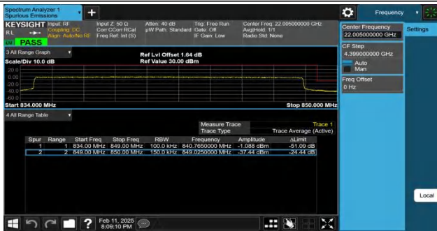
Band26(824-849)-15MHz-QPSK-26965-75RB#0-PASS
