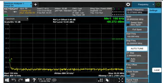
Band26(824-849)-1.4MHz-QPSK-26915-1RB#0-0.15~30-PASS
