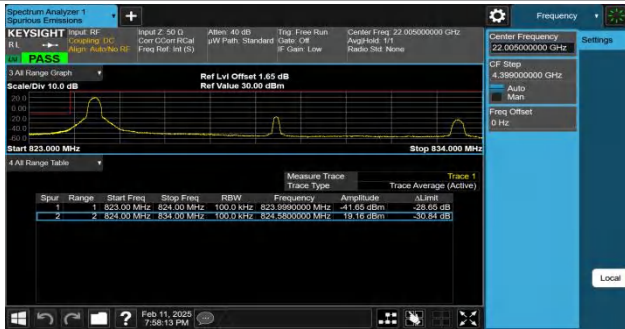
Band26(824-849)-10MHz-QPSK-26840-1RB#0-PASS
