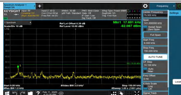
Band7-15MHz-QPSK-21100-1RB#74-0.009~0.15-PASS
