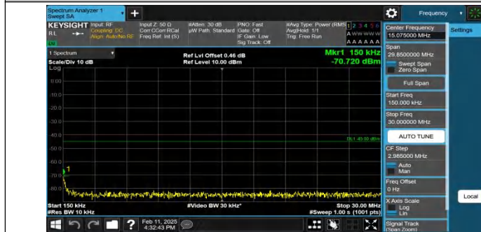
Band7-20MHz-QPSK-21100-1RB#99-0.15~30-PASS
