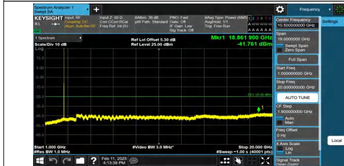
Band7-10MHz-QPSK-21400-1RB#49-1000~20000-PASS
