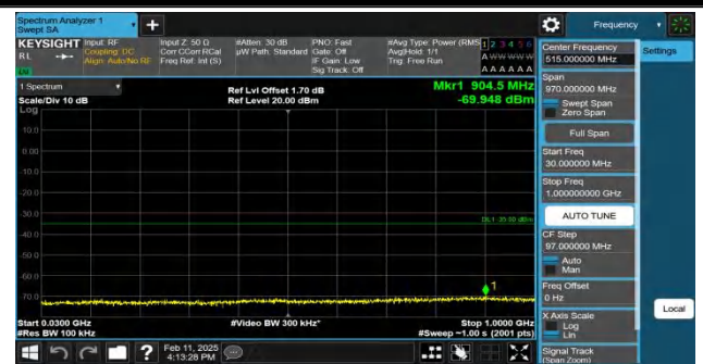
Band7-10MHz-QPSK-21400-1RB#49-30~1000-PASS
