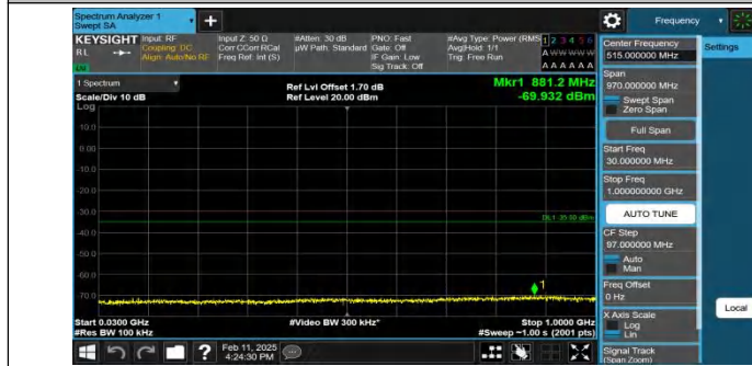
Band7-15MHz-QPSK-21375-1RB#0-30~1000-PASS
