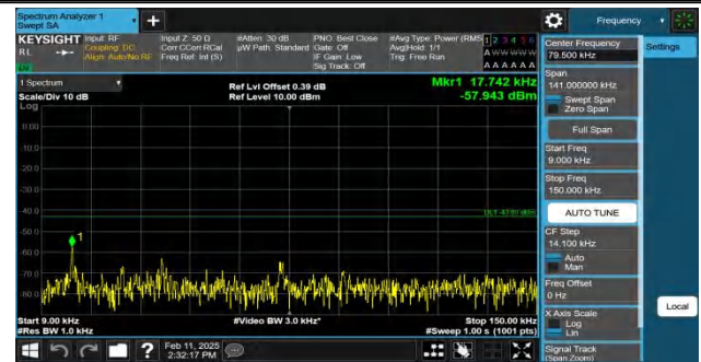
Band4-5MHz-QPSK-19975-1RB#24-0.009~0.15-PASS
