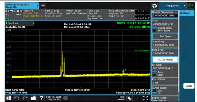
Band4-20MHz-QPSK-20175-1RB#0-1000~3000-PASS
