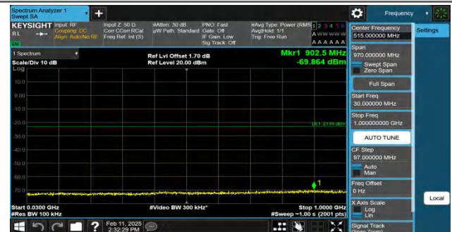
Band4-5MHz-QPSK-19975-1RB#24-30~1000-PASS
