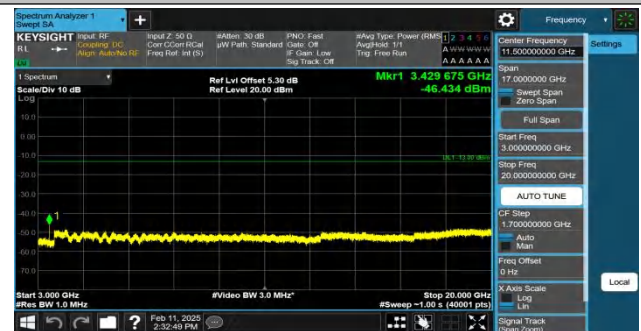
Band4-5MHz-QPSK-19975-1RB#24-3000~20000-PASS
