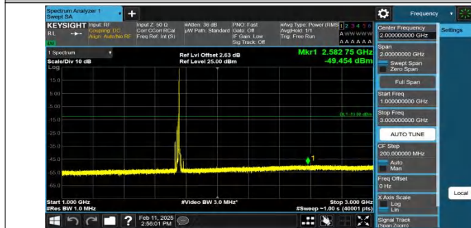
Band4-15MHz-QPSK-20325-1RB#74-1000~3000-PASS
