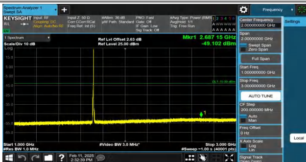
Band4-5MHz-QPSK-19975-1RB#24-1000~3000-PASS
