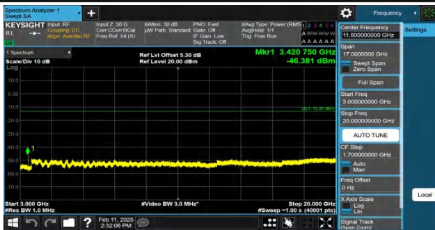
Band4-5MHz-QPSK-19975-1RB#0-3000~20000-PASS
