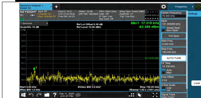
Band4-15MHz-QPSK-20025-1RB#0-0.009~0.15-PASS
