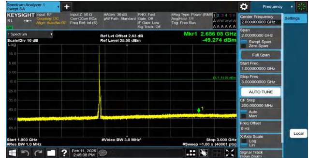
Band4-10MHz-QPSK-20350-1RB#0-1000~3000-PASS
