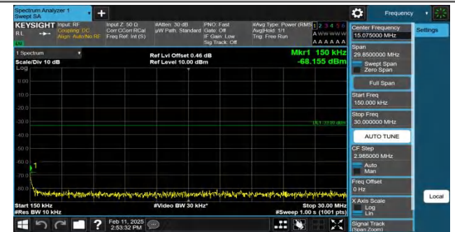
Band4-15MHz-QPSK-20175-1RB#0-0.15~30-PASS
