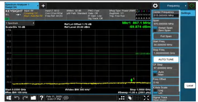
Band4-20MHz-QPSK-20175-1RB#99-30~1000-PASS
