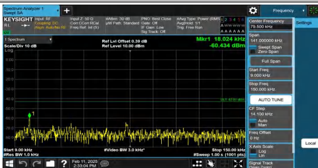
Band4-5MHz-QPSK-20175-1RB#0-0.009~0.15-PASS
