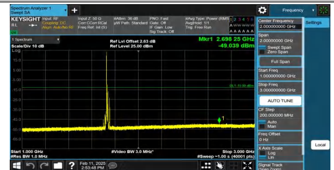
Band4-15MHz-QPSK-20175-1RB#0-1000~3000-PASS
