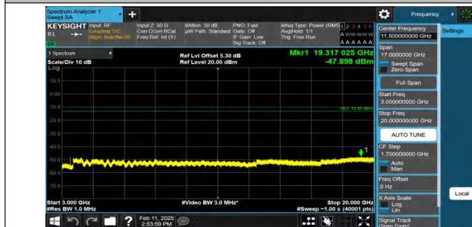
Band4-15MHz-QPSK-20175-1RB#0-3000~20000-PASS
