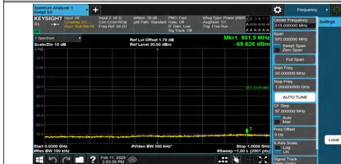
Band4-15MHz-QPSK-20175-1RB#0-30~1000-PASS
