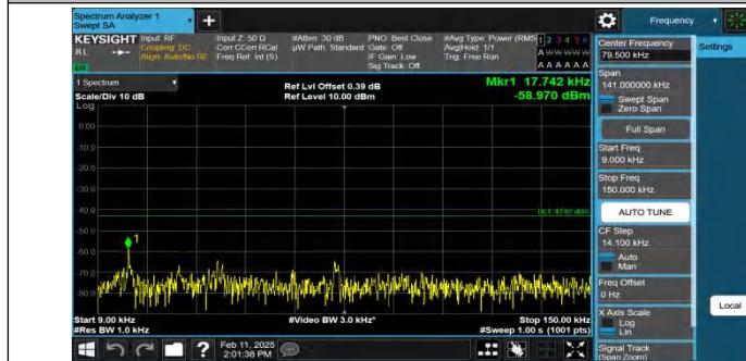
Band2-20MHz-QPSK-19100-1RB#0-0.009~0.15-PASS
