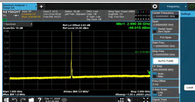
Band2-5MHz-QPSK-18900-1RB#24-1000~3000-PASS
