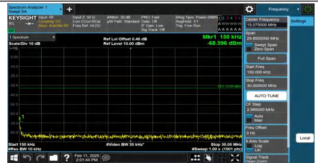
Band2-20MHz-QPSK-19100-1RB#0-0.15~30-PASS
