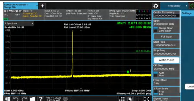
Band2-5MHz-QPSK-18900-1RB#0-1000~3000-PASS
