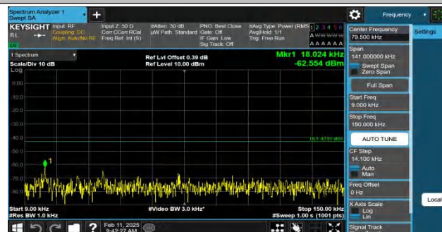
Band2-5MHz-QPSK-18900-1RB#24-0.009~0.15-PASS
