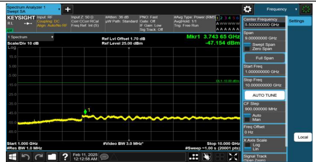
Band5-4182-5-1000~10000MHz-PASS
