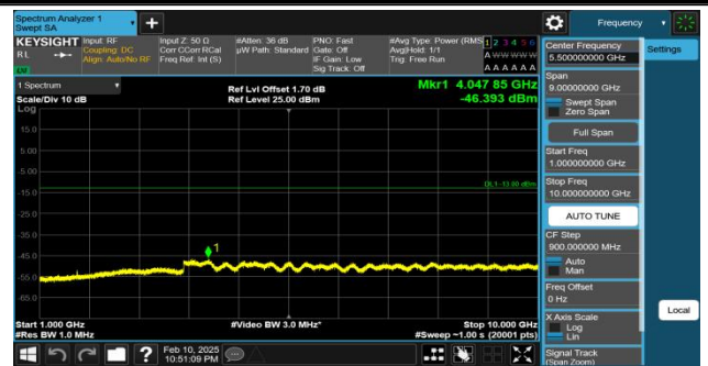
Band5-4182-1-1000~10000MHz-PASS
