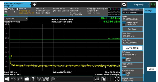
Band5-4233-5-0.15~30MHz-PASS
