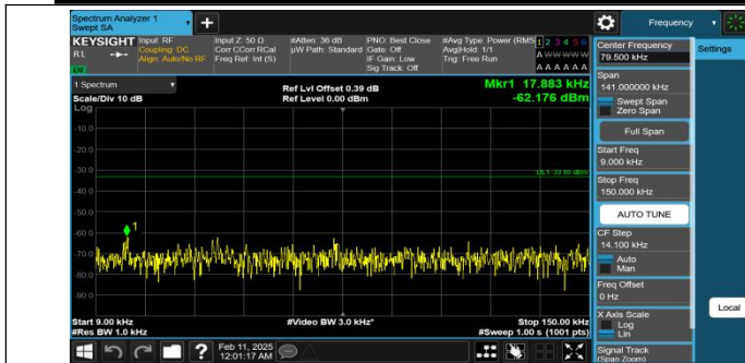
Band5-4132-1-0.009~0.15MHz-PASS
