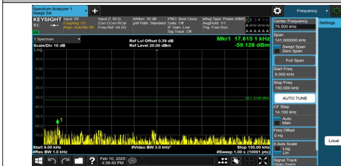
GPRS850-190-5-0.009~0.15MHz-PASS
