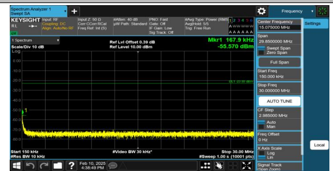
GPRS850-190-5-0.15~30MHz-PASS
