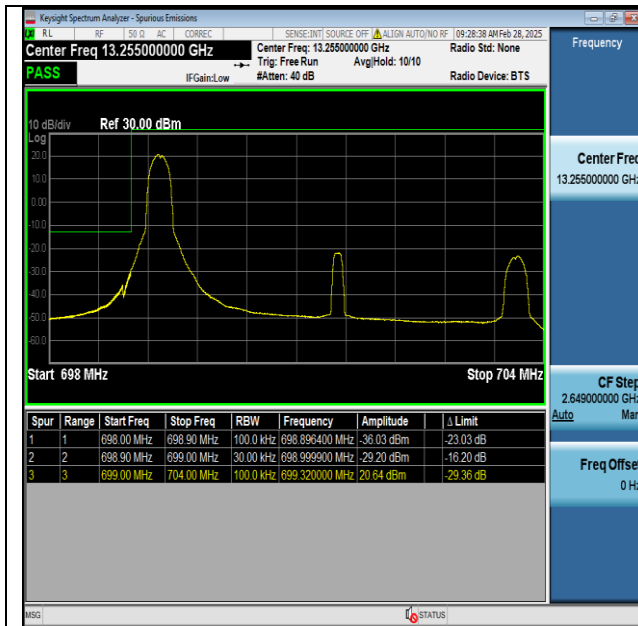
Band12-5MHz-QPSK-23035-1RB#0-PASS
