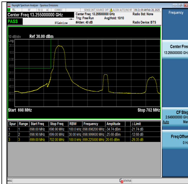
Band12-3MHz-QPSK-23025-1RB#0-PASS
