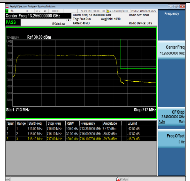
Band12-3MHz-QPSK-23165-15RB#0-PASS
