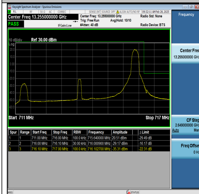
Band12-5MHz-QPSK-23155-1RB#24-PASS
