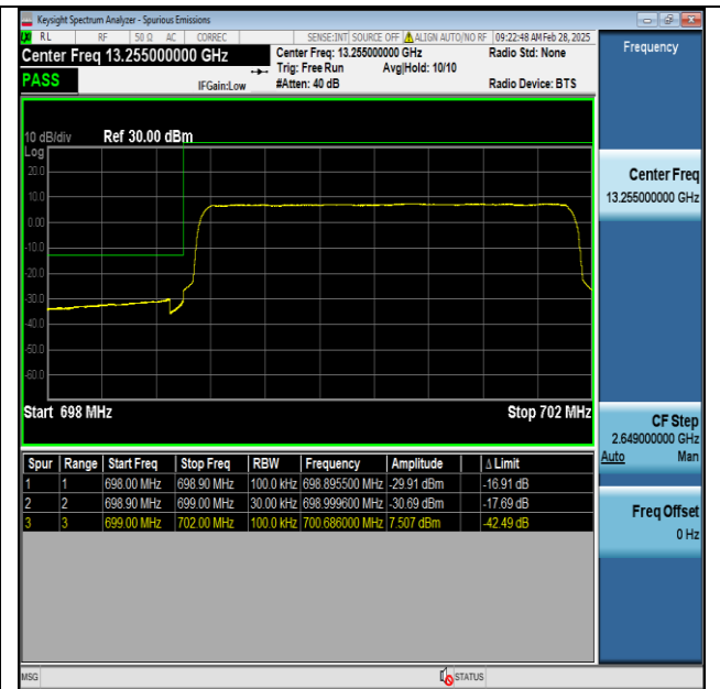
Band12-3MHz-QPSK-23025-15RB#0-PASS
