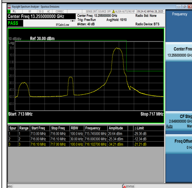
Band12-3MHz-QPSK-23165-1RB#14-PASS
