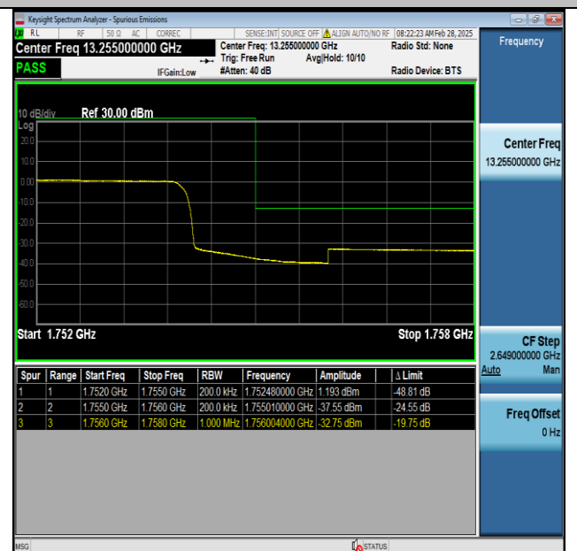
Band4-20MHz-QPSK-20300-100RB#0-PASS
