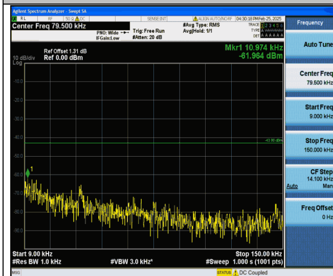
Band II-9538-0.009~0.15MHz-PASS
