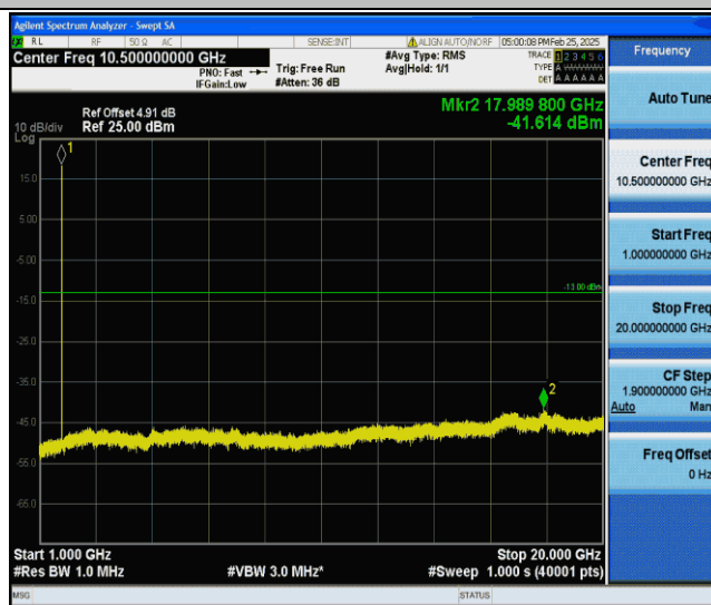
Band IV-1513-1000~20000MHz-PASS
