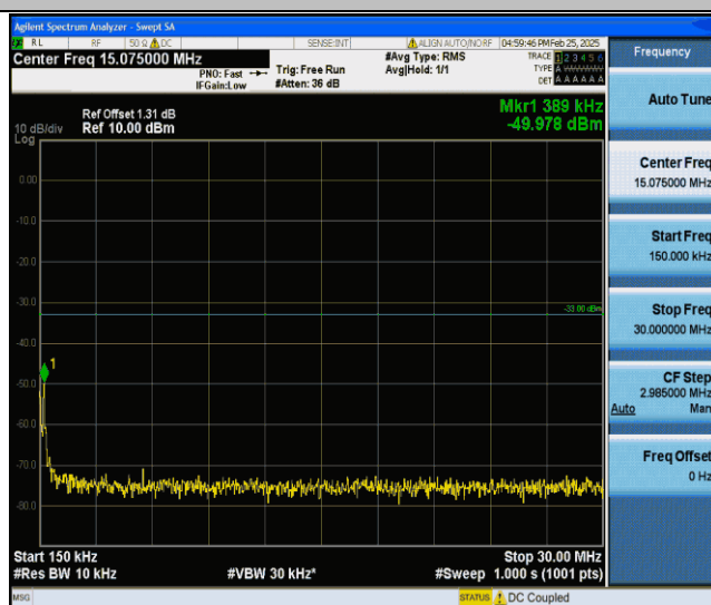
Band IV-1513-0.15~30MHz-PASS
