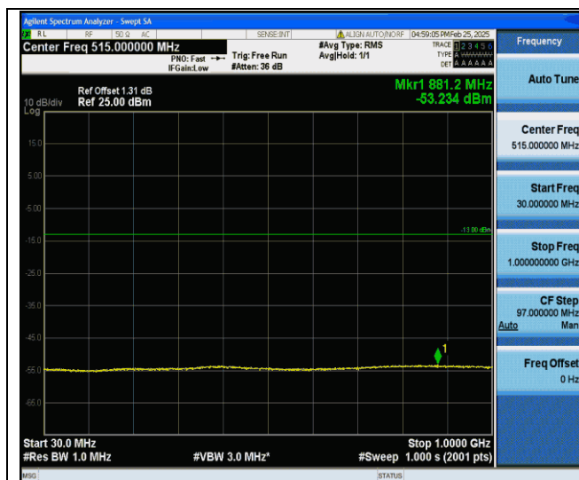
Band IV-1413-30~1000MHz-PASS
