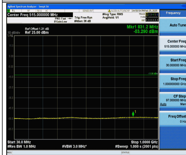
Band IV-1513-30~1000MHz-PASS
