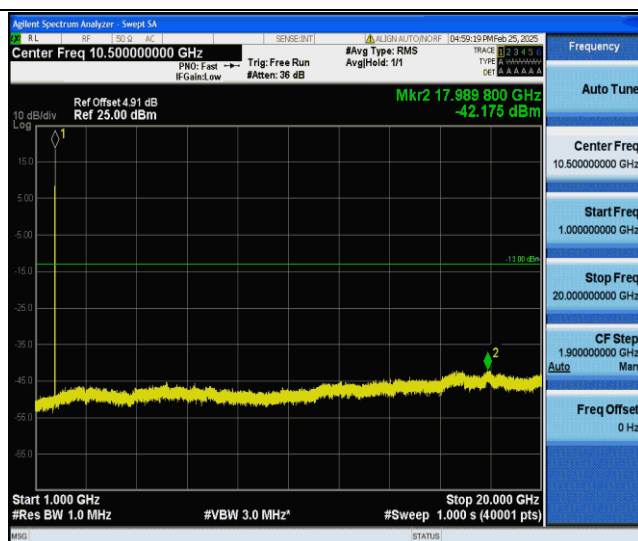
Band IV-1413-1000~20000MHz-PASS
