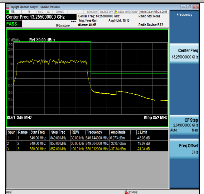
Band5-3MHz-QPSK-20635-15RB#0-PASS
