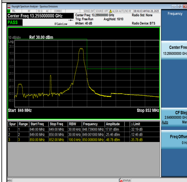
Band5-3MHz-QPSK-20635-1RB#14-PASS
