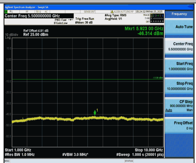
Band V-4132-1000~10000MHz-PASS
