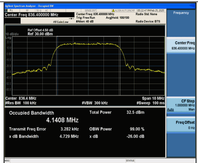
Band V-4182-PASS
