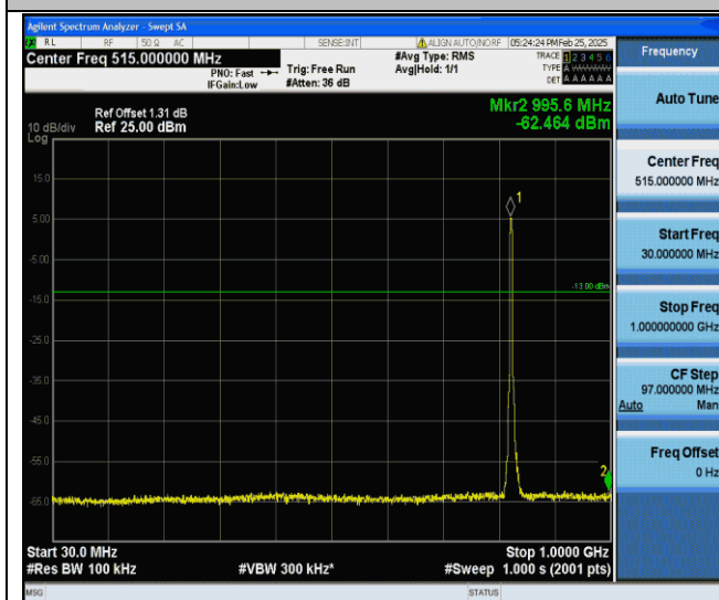
Band V-4132-30~1000MHz-PASS
