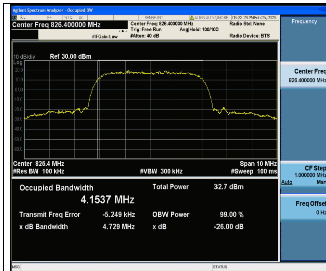
Band V-4132-PASS
