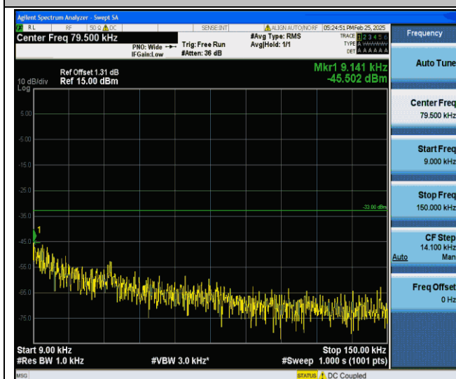
Band V-4182-0.009~0.15MHz-PASS
