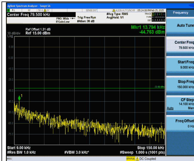
Band V-4132-0.009~0.15MHz-PASS
