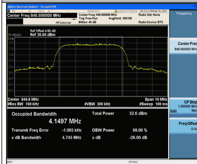
Band V-4233-PASS
