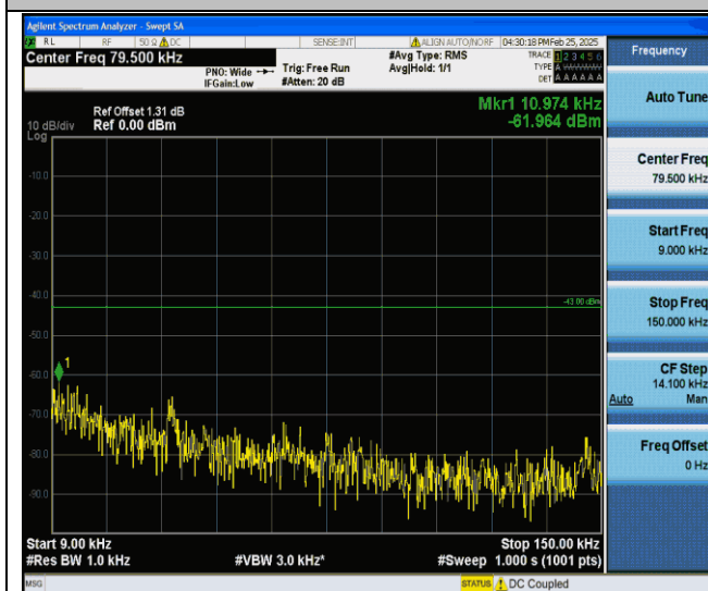
Band II-9538-0.009~0.15MHz-PASS
