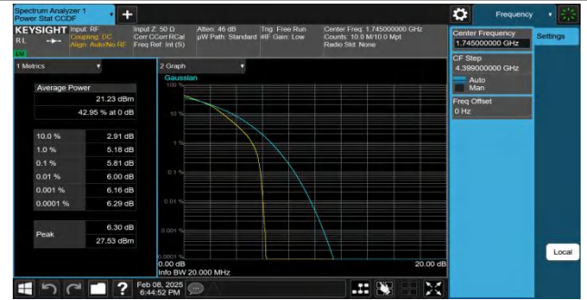
Band66-20MHz-16QAM-132322-27RB#0-PASS
