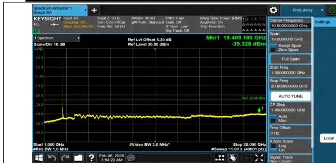
Band41-10MHz-QPSK-40620-1RB#49-1000~20000-PASS
