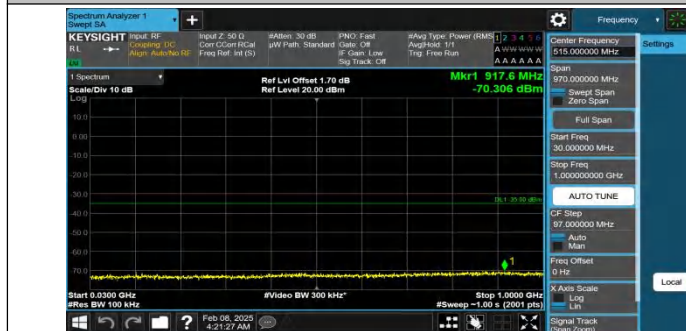
Band41-20MHz-QPSK-39750-1RB#0-30~1000-PASS
