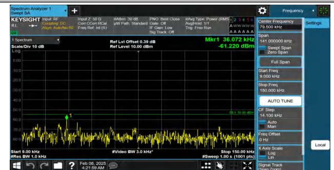
Band41-20MHz-QPSK-39750-1RB#99-0.009~0.15-PASS
