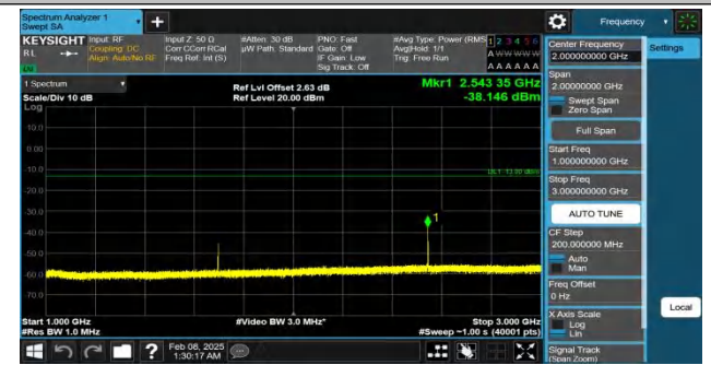
Band26(824-849)-1.4MHz-QPSK-27033-1RB#0-1000~3000-PASS
