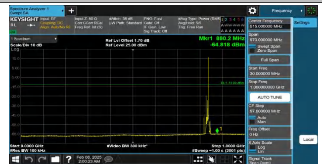
Band26(824-849)-10MHz-QPSK-26915-1RB#49-30~1000-PASS
