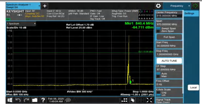
Band26(824-849)-5MHz-QPSK-26815-1RB#24-30~1000-PASS
