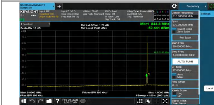
Band26(824-849)-1.4MHz-QPSK-27033-1RB#0-30~1000-PASS
