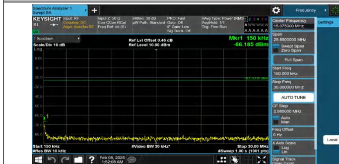
Band26(824-849)-5MHz-QPSK-27015-1RB#24-0.15~30-PASS
