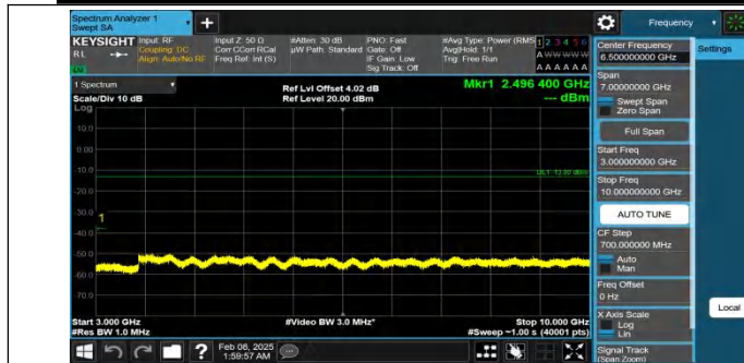
Band26(824-849)-10MHz-QPSK-26915-1RB#0-3000~10000-PAS
