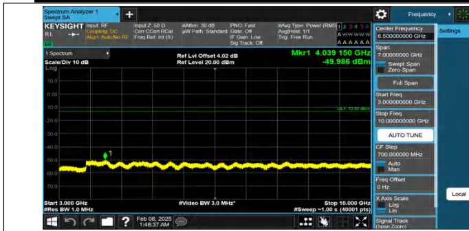
Band26(824-849)-5MHz-QPSK-26815-1RB#0-3000~10000-PASS
