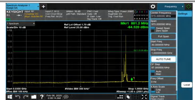
Band26(824-849)-15MHz-QPSK-26865-1RB#74-30~1000-PASS
