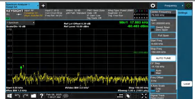
Band26(824-849)-3MHz-QPSK-26805-1RB#14-0.009~0.15-PASS
