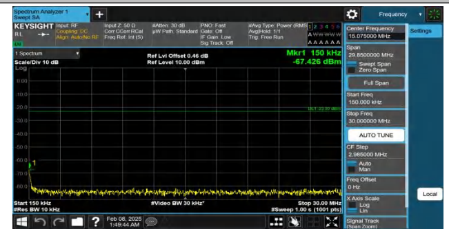
Band26(824-849)-5MHz-QPSK-26915-1RB#0-0.15~30-PASS
