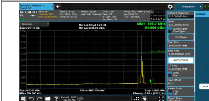
Band26(824-849)-10MHz-QPSK-26915-1RB#0-30~1000-PASS
