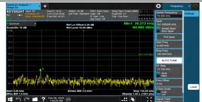
Band26(824-849)-3MHz-QPSK-26915-1RB#14-0.009~0.15-PASS
