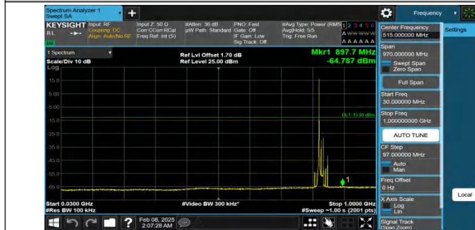
Band26(824-849)-15MHz-QPSK-26865-1RB#0-30~1000-PASS
