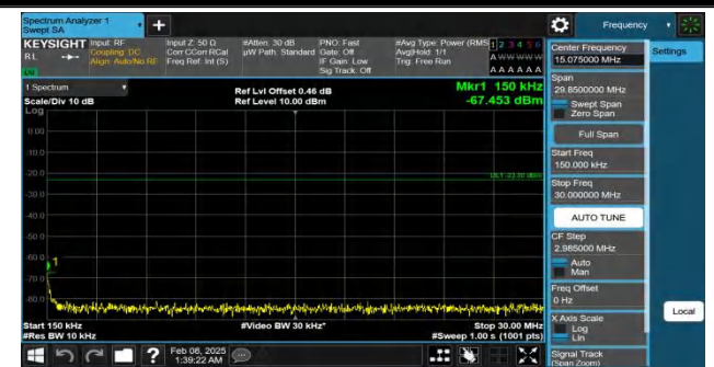
Band26(824-849)-3MHz-QPSK-26915-1RB#0-0.15~30-PASS
