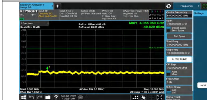
Band26(824-849)-3MHz-QPSK-26915-1RB#0-3000~10000-PASS
