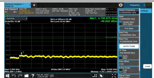
Band26(824-849)-10MHz-QPSK-26915-1RB#49-3000~10000-PAS
