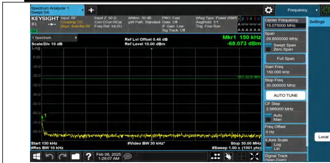
Band26(824-849)-1.4MHz-QPSK-26915-1RB#5-0.15~30-PASS
