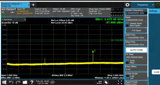
Band26(824-849)-1.4MHz-QPSK-26797-1RB#5-1000~3000-PASS
