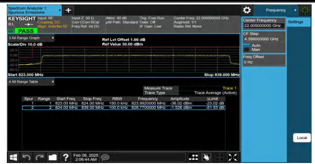
Band26(824-849)-15MHz-QPSK-26865-75RB#0-PASS
