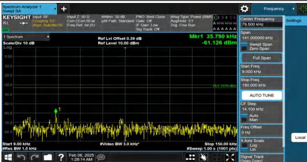
Band26(824-849)-1.4MHz-QPSK-26915-1RB#0-0.009~0.15-PASS
