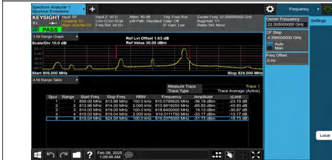
Band26(814-824)-5MHz-QPSK-26715-1RB#24-PASS
