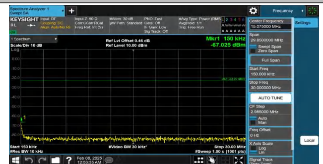
Band26(814-824)-1.4MHz-QPSK-26783-1RB#0-0.15~30-PASS
