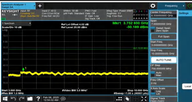
Band26(814-824)-1.4MHz-QPSK-26783-1RB#0-3000~10000-PAS S
