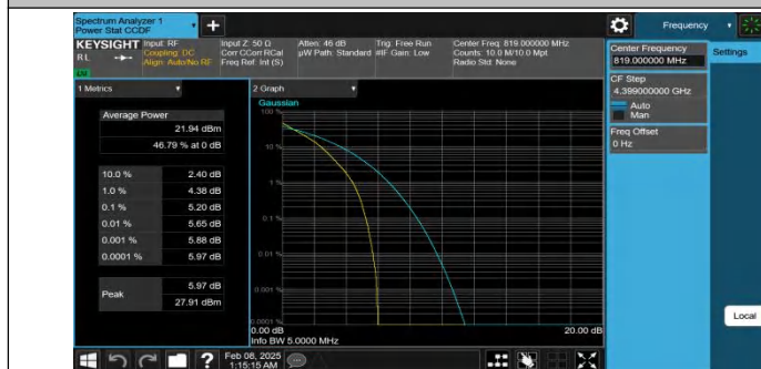
Band26(814-824)-5MHz-QPSK-26740-25RB#0-PASS
