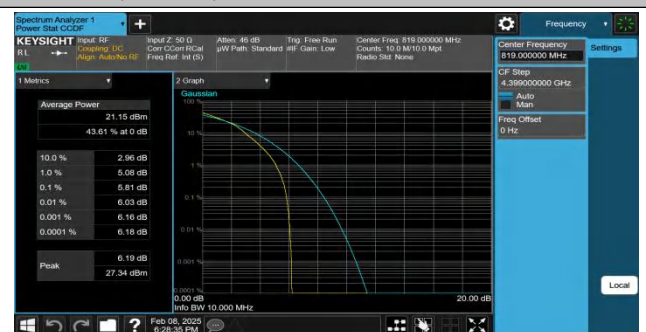
Band26(814-824)-10MHz-16QAM-26740-27RB#0-PASS
