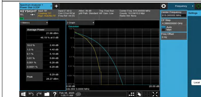
Band26(814-824)-3MHz-QPSK-26740-15RB#0-PASS
