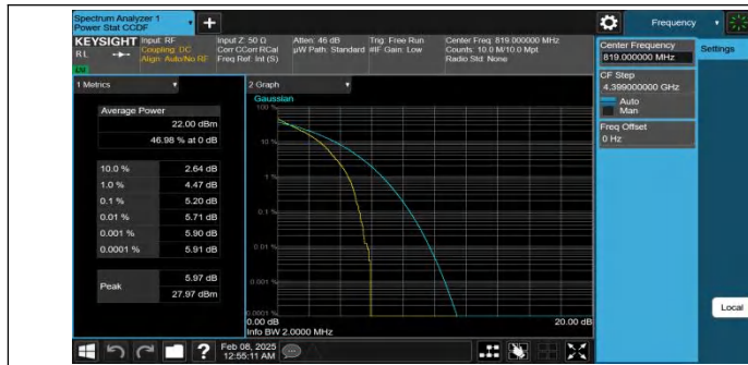
Band26(814-824)-1.4MHz-QPSK-26740-6RB#0-PASS
