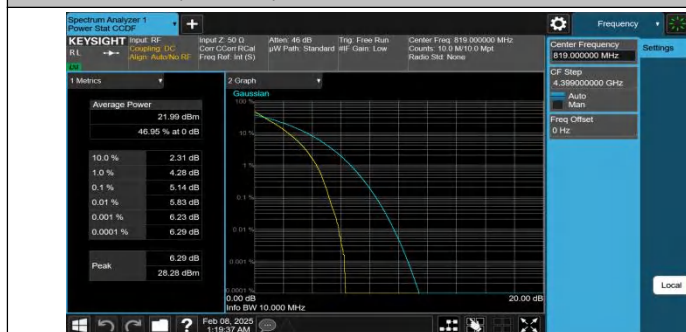
Band26(814-824)-10MHz-QPSK-26740-50RB#0-PASS
