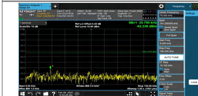
Band26(814-824)-1.4MHz-QPSK-26783-1RB#0-0.009~0.15-PASS
