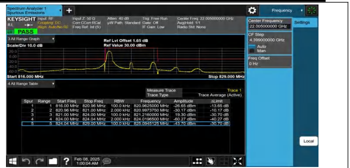
Band26(814-824)-3MHz-QPSK-26775-1RB#0-PASS
