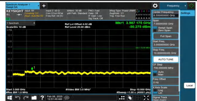
Band26(814-824)-1.4MHz-QPSK-26697-1RB#5-3000~10000-PASS S
