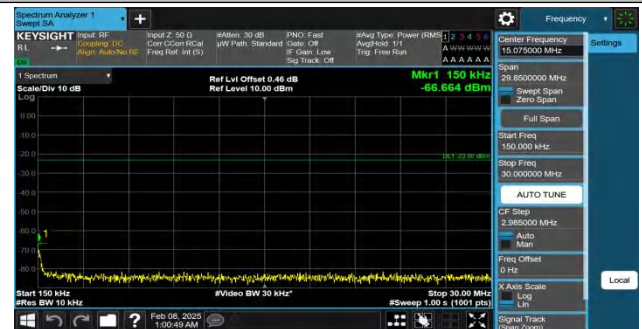
Band26(814-824)-3MHz-QPSK-26705-1RB#0-0.15~30-PASS
