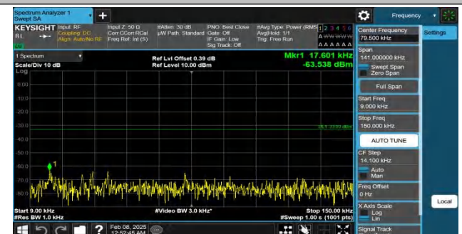
Band26(814-824)-1.4MHz-QPSK-26740-1RB#5-0.009~0.15-PASS
