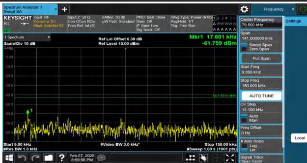
Band4-15MHz-QPSK-20025-1RB#0-0.009~0.15-PASS
