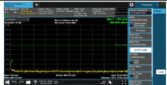
Band4-15MHz-QPSK-20025-1RB#0-0.15~30-PASS
