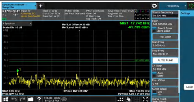
Band4-5MHz-QPSK-20175-1RB#0-0.009~0.15-PASS
