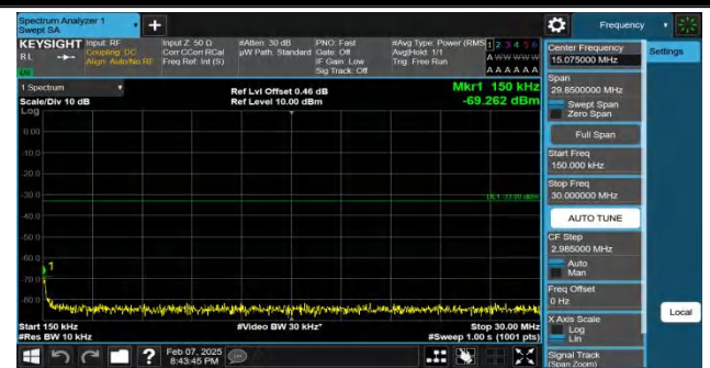
Band4-5MHz-QPSK-20375-1RB#0-0.15~30-PASS
