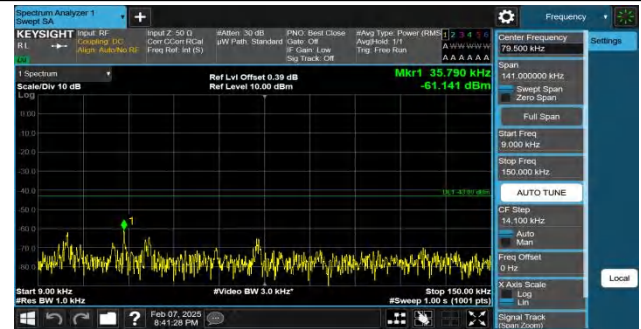
Band4-5MHz-QPSK-19975-1RB#24-0.009~0.15-PASS
