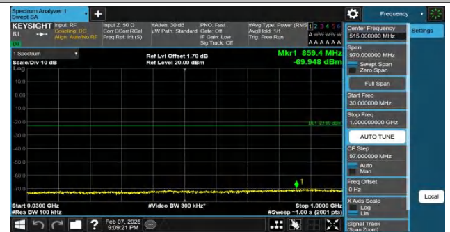
Band4-20MHz-QPSK-20050-1RB#99-30~1000-PASS
