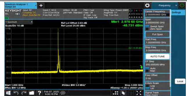
Band4-15MHz-QPSK-20025-1RB#0-1000~3000-PASS
