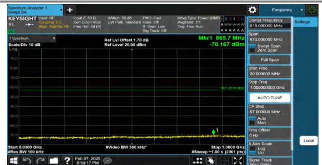
Band4-10MHz-QPSK-20350-1RB#49-30~1000-PASS
