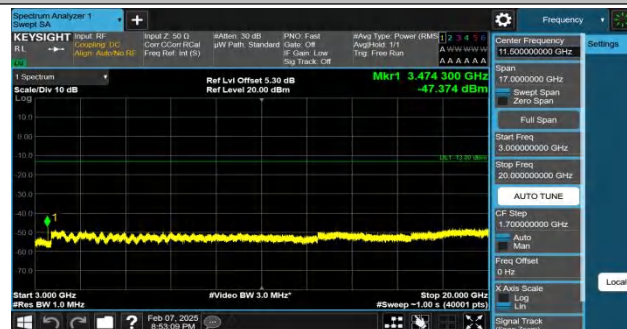
Band4-10MHz-QPSK-20175-1RB#49-3000~20000-PASS
