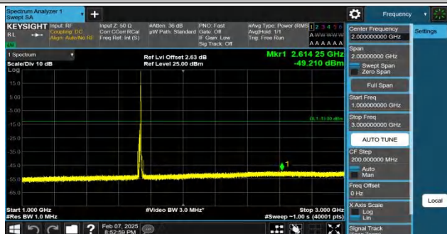
Band4-10MHz-QPSK-20175-1RB#49-1000~3000-PASS
