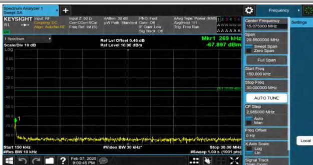
Band4-15MHz-QPSK-20025-1RB#74-0.15~30-PASS
