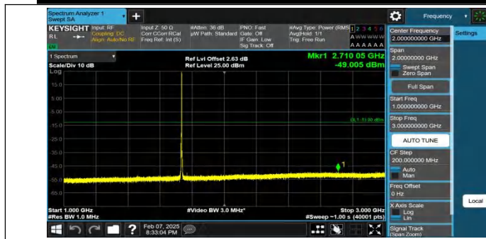
Band4-3MHz-QPSK-20175-1RB#14-1000~3000-PASS
