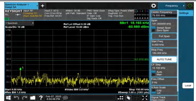
Band4-10MHz-QPSK-20350-1RB#49-0.009~0.15-PASS
