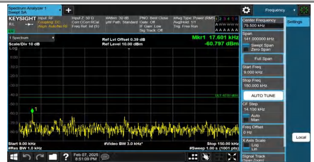
Band4-10MHz-QPSK-20000-1RB#49-0.009~0.15-PASS
