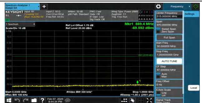
Band4-5MHz-QPSK-20375-1RB#24-30~1000-PASS
