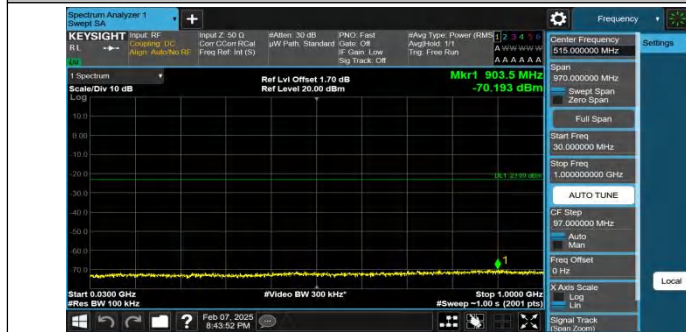
Band4-5MHz-QPSK-20375-1RB#0-30~1000-PASS
