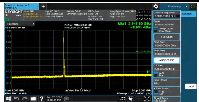
Band4-10MHz-QPSK-20350-1RB#0-1000~3000-PASS
