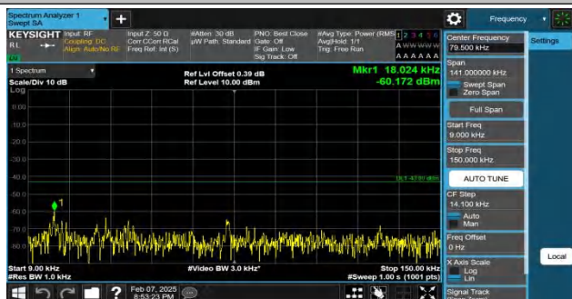
Band4-10MHz-QPSK-20350-1RB#0-0.009~0.15-PASS
