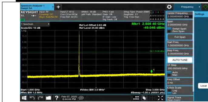
Band4-5MHz-QPSK-20375-1RB#24-1000~3000-PASS
