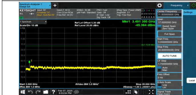
Band4-10MHz-QPSK-20350-1RB#0-3000~20000-PASS
