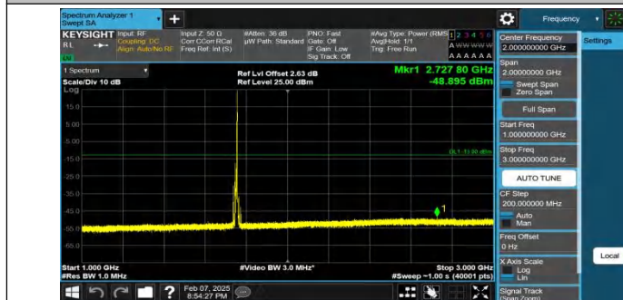
Band4-10MHz-QPSK-20350-1RB#49-1000~3000-PASS
