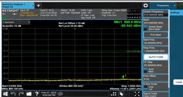
Band4-15MHz-QPSK-20025-1RB#0-30~1000-PASS
