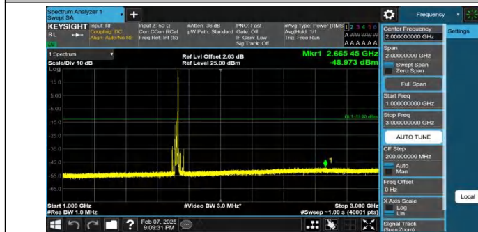
Band4-20MHz-QPSK-20050-1RB#99-1000~3000-PASS
