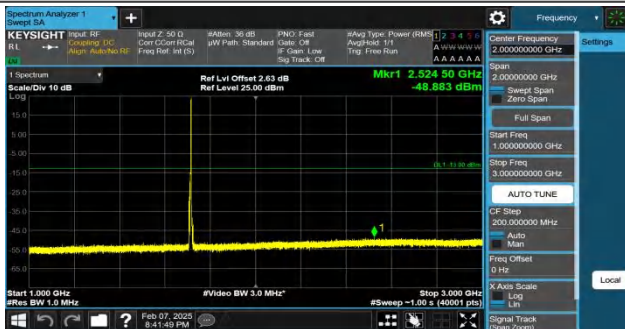
Band4-5MHz-QPSK-19975-1RB#24-1000~3000-PASS
