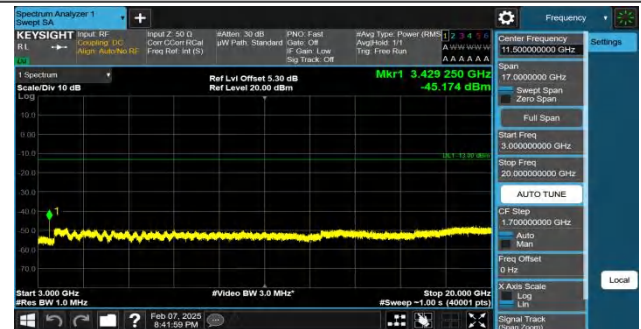
Band4-5MHz-QPSK-19975-1RB#24-3000~20000-PASS
