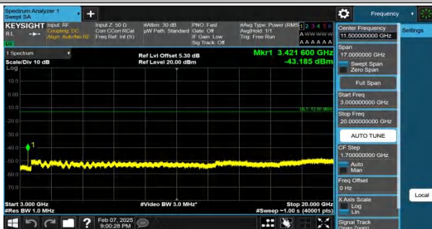
Band4-15MHz-QPSK-20025-1RB#0-3000~20000-PASS
