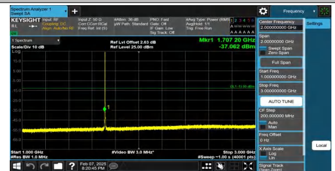
Band4-1.4MHz-QPSK-19957-1RB#0-1000~3000-PASS
