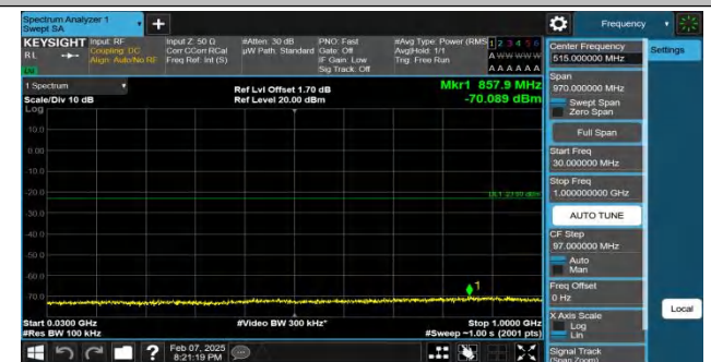
Band4-1.4MHz-QPSK-19957-1RB#5-30~1000-PASS
