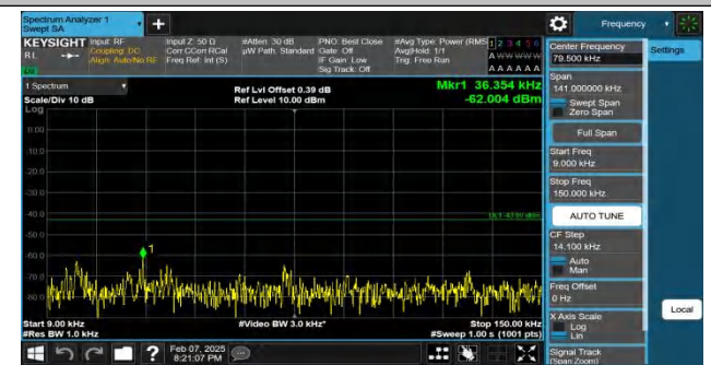
Band4-1.4MHz-QPSK-19957-1RB#5-0.009~0.15-PASS
