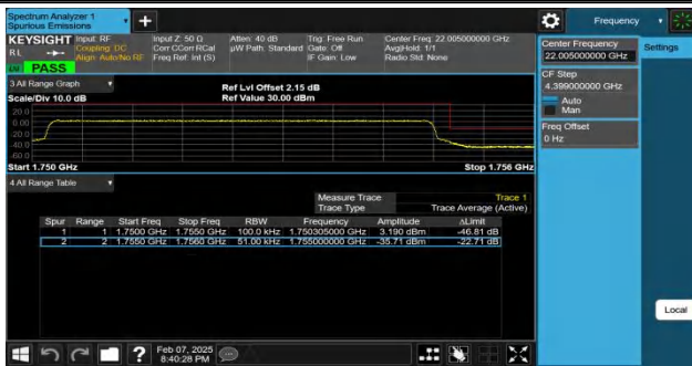
Band4-5MHz-QPSK-20375-25RB#0-PASS
