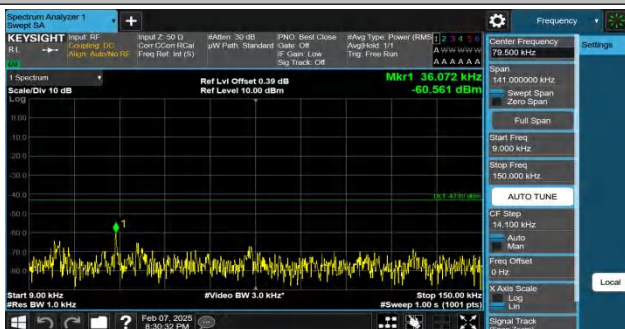
Band4-3MHz-QPSK-19965-1RB#0-0.009~0.15-PASS
