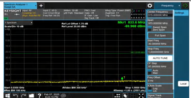
Band4-1.4MHz-QPSK-20393-1RB#5-30~1000-PASS
