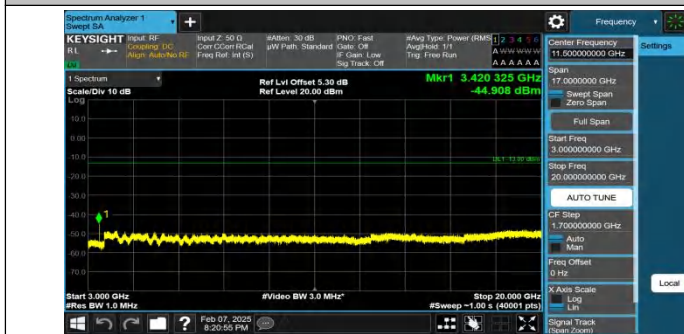
Band4-1.4MHz-QPSK-19957-1RB#0-3000~20000-PASS
