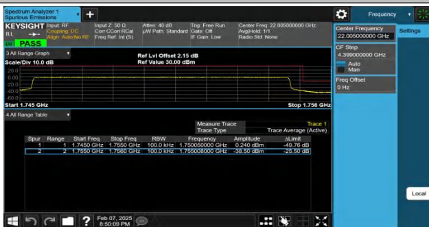
Band4-10MHz-QPSK-20350-50RB#0-PASS
