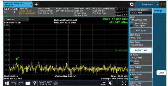
Band4-1.4MHz-QPSK-20393-1RB#5-0.009~0.15-PASS
