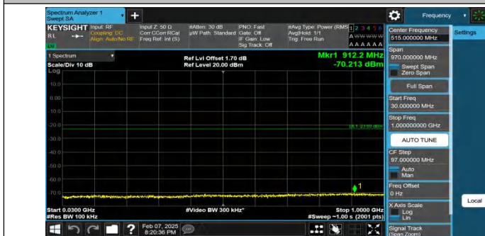
Band4-1.4MHz-QPSK-19957-1RB#0-30~1000-PASS
