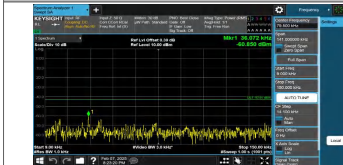
Band4-1.4MHz-QPSK-20393-1RB#0-0.009~0.15-PASS
