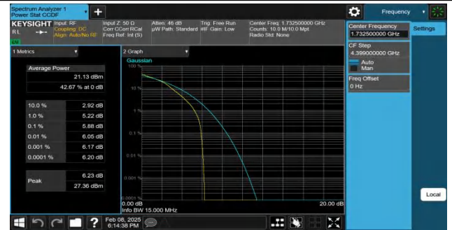
Band4-15MHz-16QAM-20175-27RB#0-PASS
