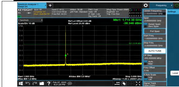
Band4-1.4MHz-QPSK-19957-1RB#5-1000~3000-PASS
