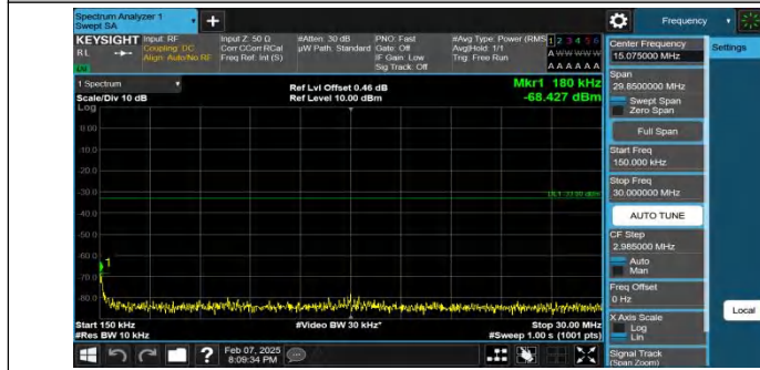
Band2-20MHz-QPSK-18900-1RB#99-0.15~30-PASS
