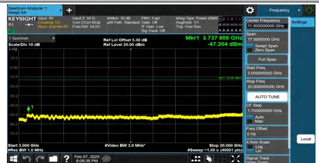
Band2-20MHz-QPSK-18700-1RB#99-3000~20000-PASS
