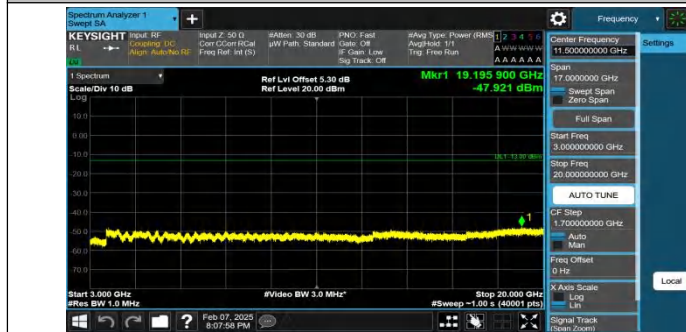
Band2-20MHz-QPSK-18700-1RB#0-3000~20000-PASS
