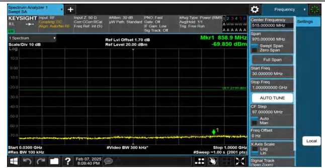
Band2-20MHz-QPSK-18900-1RB#99-30~1000-PASS
