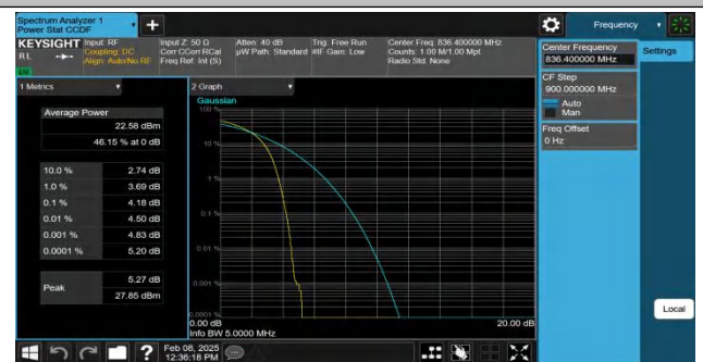
Band5-4182-5-PASS
