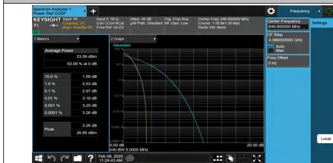
Band5-4233-PASS
