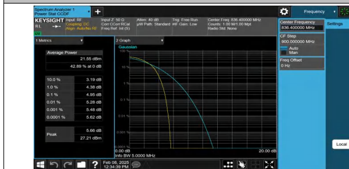
Band5-4182-4-PASS
