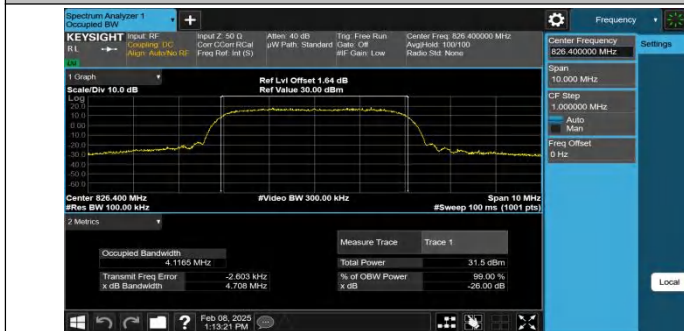
Band5-4132-5-PASS
