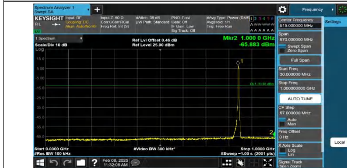
Band5-4233-30~1000MHz-PASS
