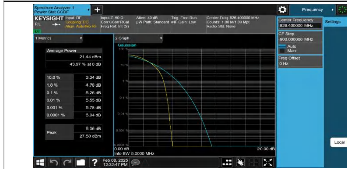
Band5-4132-3-PASS
