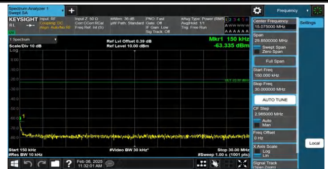
Band5-4233-0.15~30MHz-PASS
