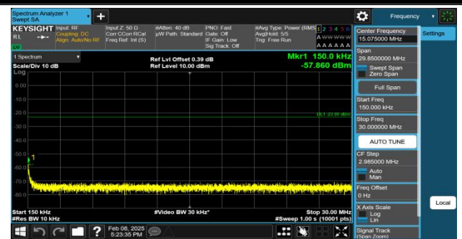
EGPRS850-190-8-0.15~30MHz-PASS
