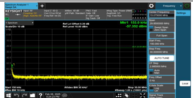
EGPRS850-251-8-0.15~30MHz-PASS
