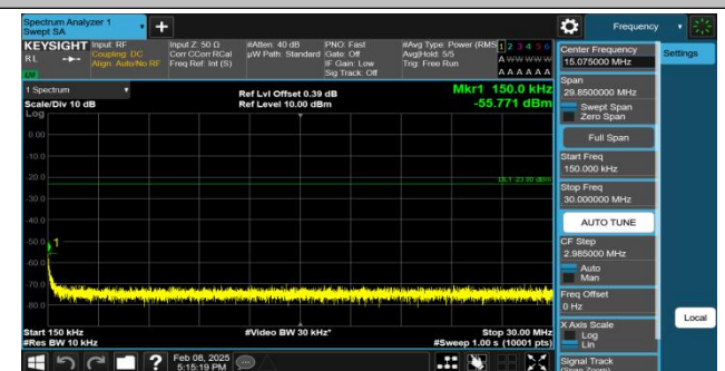
GPRS850-190-5-0.15~30MHz-PASS
