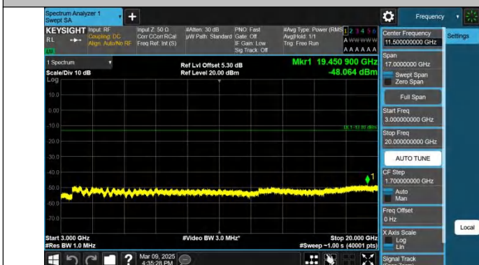
Band2-10MHz-QPSK-18650-1RB#0-3000~20000-PASS
