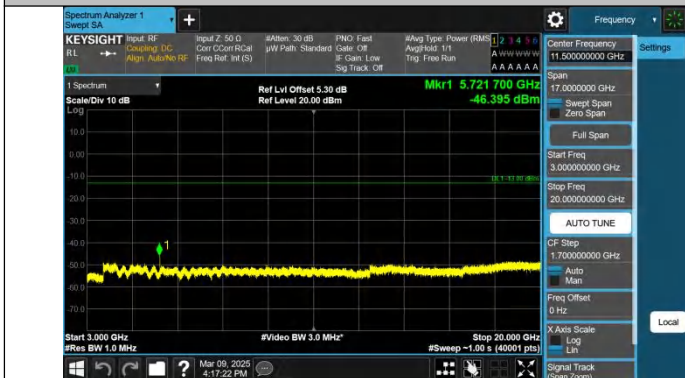
Band2-3MHz-QPSK-19185-1RB#0-3000~20000-PASS
