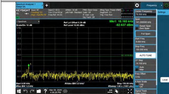
Band2-10MHz-QPSK-18900-1RB#0-0.009~0.15-PASS
