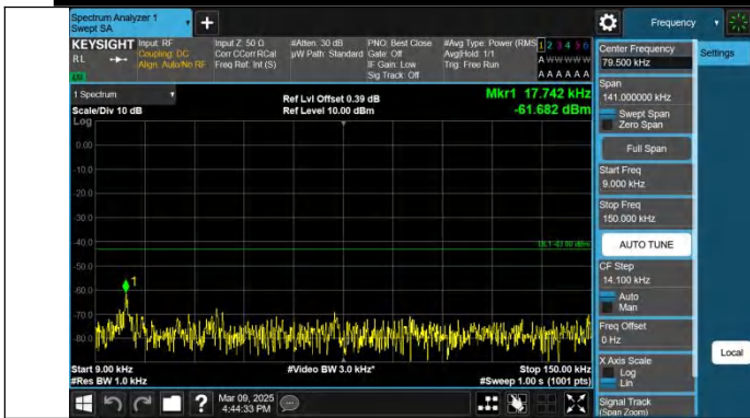
Band2-15MHz-QPSK-18675-1RB#0-0.09~0.15-PASS
