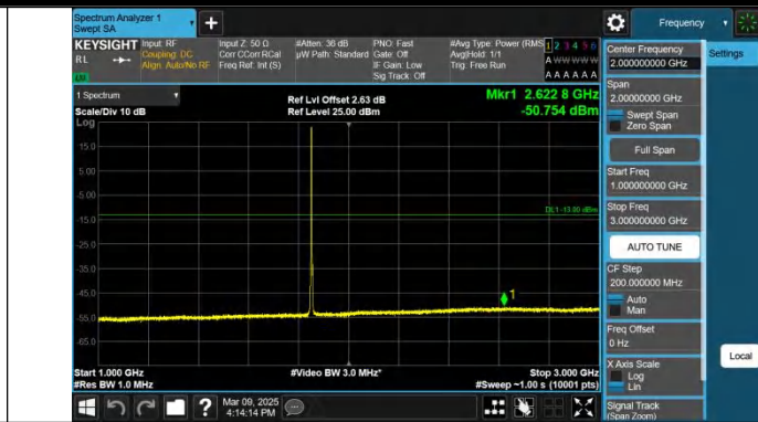
Band2-3MHz-QPSK-18615-1RB#0-1000~3000-PASS
