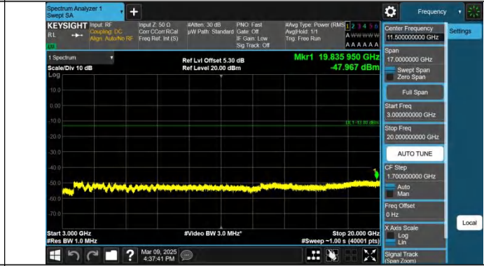
Band2-10MHz-QPSK-18900-1RB#49.3000~20000-PASS
