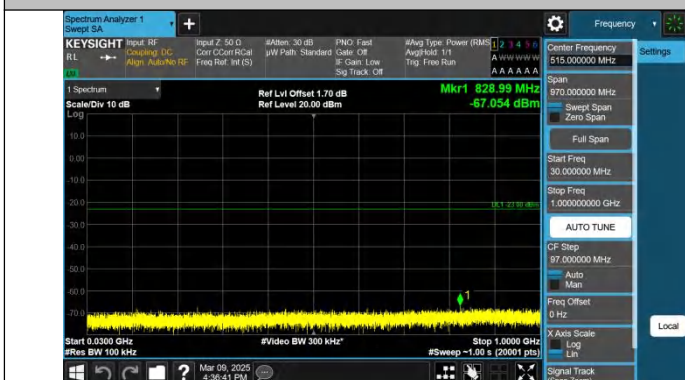
Band2-10MHz-QPSK-18900-1RB#0-30~1000-PASS
