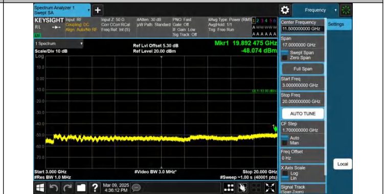
Band2-10MHz-QPSK-18650-1RB#49-3000~20000-PASS
