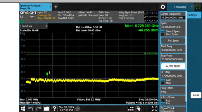
Band2-1.4MHz-QPSK-19193-1RB#5-3000~20000-PASS
