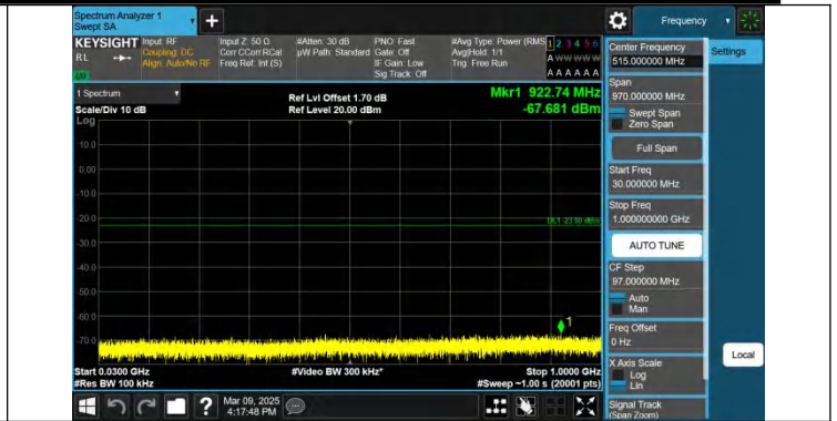
Band2-3MHz-QPSK-19185-1RB#14-30~1000-PASS
