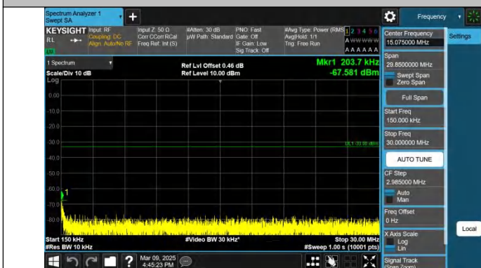
Band2-15MHz-QPSK-18675-1RB#74-0.15~30-PASS
