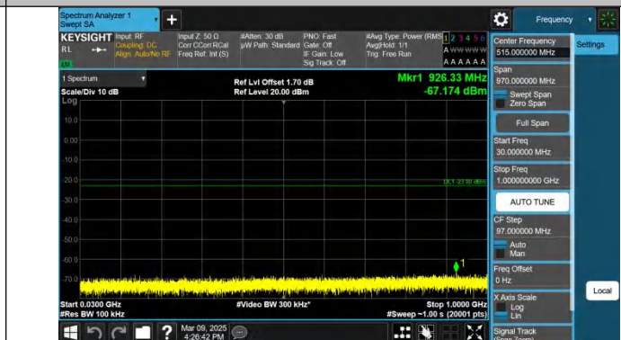
Band2-5MHz-QPSK-18900-1RB#24-30~1000-PASS
