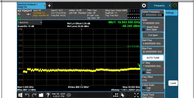
Band2-5MHz-QPSK-18625-1RB#24-3000~20000-PASS
