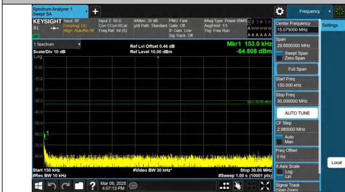
Band2-1.4MHz-QPSK-19193-1RB#5-0.15~30-PASS
