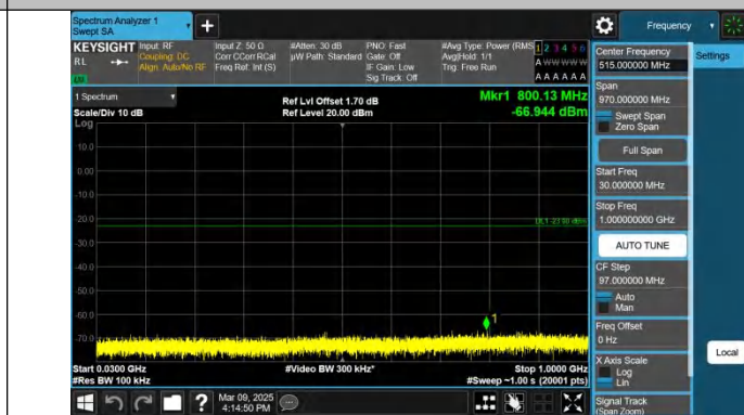
Band2-3MHz-QPSK-18615-1RB#14-30~1000-PASS
