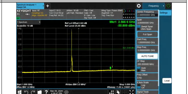
Band2-10MHz-QPSK-18900-1RB#0-1000~3000-PASS
