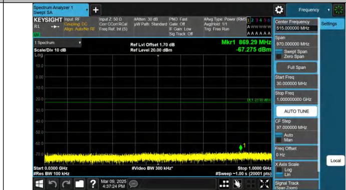
Band2-10MHz-QPSK-18900-1RB#49.30~1000-PASS
