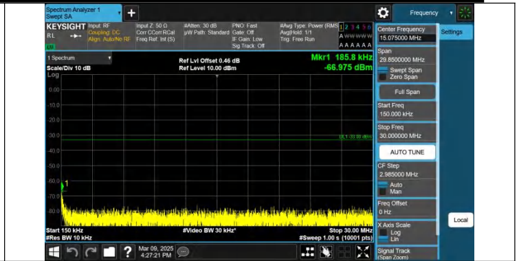
Band2-5MHz-QPSK-19175-1RB#0-0.15~30-PASS
