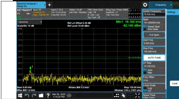
Band2-3MHz-QPSK-18900-1RB#0-0.009~0.15-PASS
