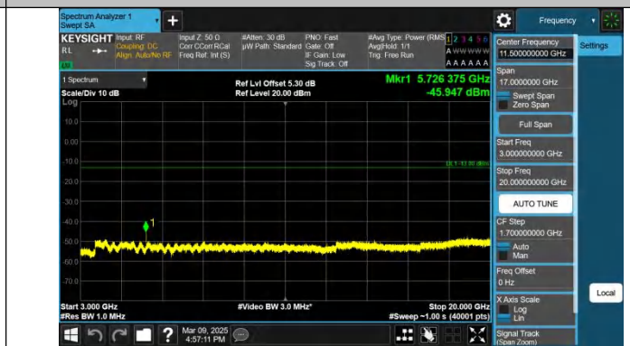
Band2-20MHz-QPSK-19100-1RB#99-3000~20000-PASS
