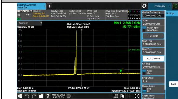
Band2-15MHz-QPSK-19125-1RB#74.1000~3000-PASS
