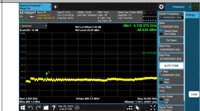
Band2-15MHz-QPSK-19125-1RB#74.3000~20000-PASS
