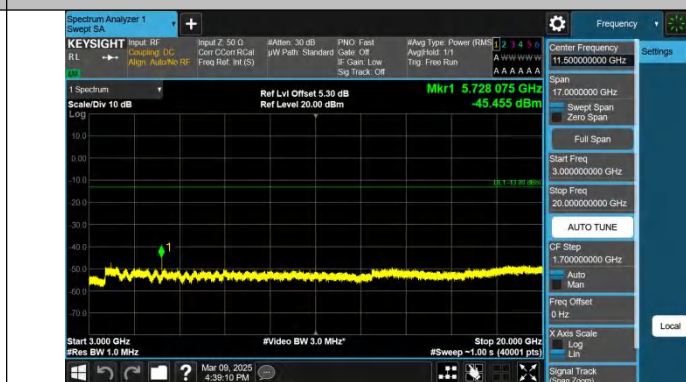
Band2-10MHz-QPSK-19150-1RB#49.3000~20000-PASS
