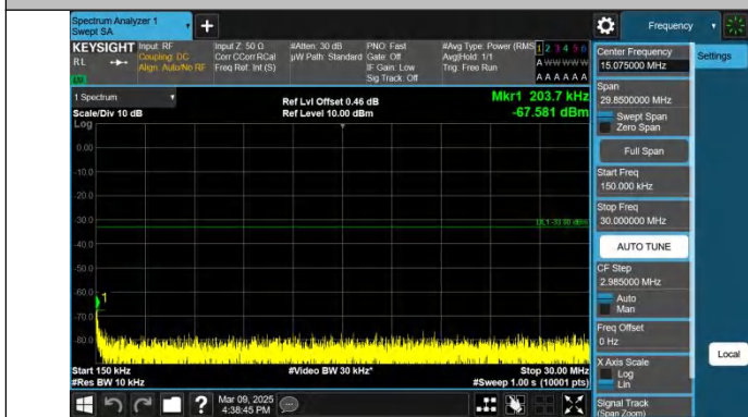
Band2-10MHz-QPSK-19150-1RB#49.0.15~30-PASS
