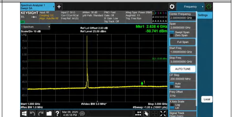
Band2-10MHz-QPSK-18650-1RB#0-1000~3000-PASS
