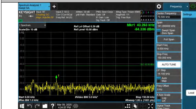
Band2-10MHz-QPSK-18650-1RB#0-0.009~0.15-PASS
