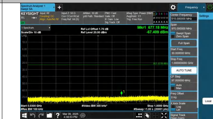
Band2-10MHz-QPSK-19150-1RB#49.30~1000-PASS
