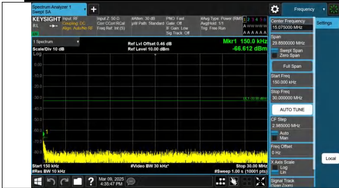
Band2-10MHz-QPSK-18650-1RB#49-0.15~30-PASS
