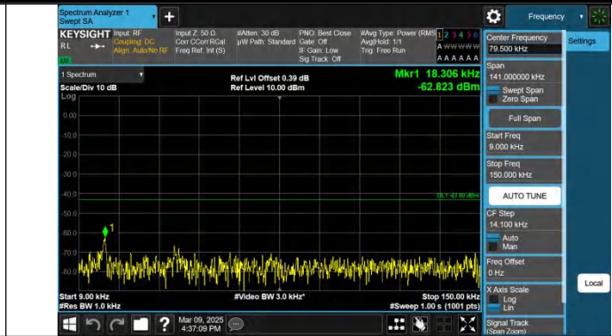
Band2-10MHz-QPSK-18900-1RB#49.0.009~0.15-PASS
