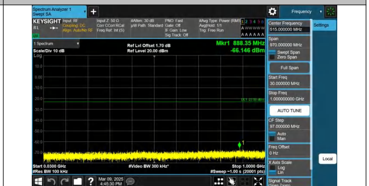
Band2-15MHz-QPSK-18675-1RB#74-30~1000-PASS
