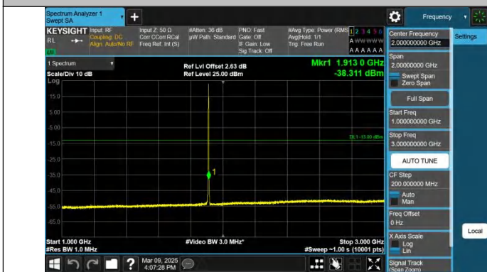
Band2-1.4MHz-QPSK-19193-1RB#5-1000~3000-PASS
