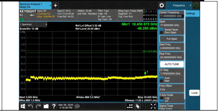
Band2-3MHz-QPSK-18900-1RB#14-3000~20000-PASS
