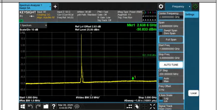
Band2-15MHz-QPSK-18675-1RB#0-1000~3000-PASS
