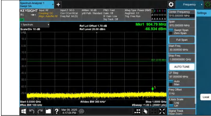
Band2-3MHz-QPSK-19185-1RB#0-30~1000-PASS
