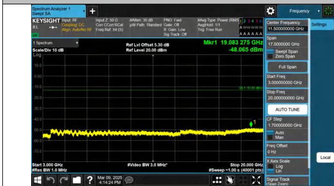
Band2-3MHz-QPSK-18615-1RB#0-3000~20000-PASS
