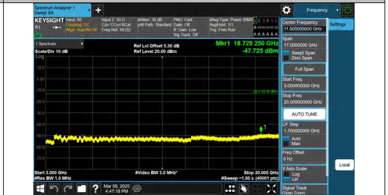
Band2-15MHz-QPSK-18900-1RB#74-3000~20000-PASS
