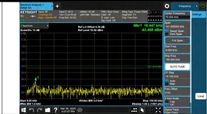
Band2-1.4MHz-QPSK-19193-1RB#5-0.009~0.15-PASS
