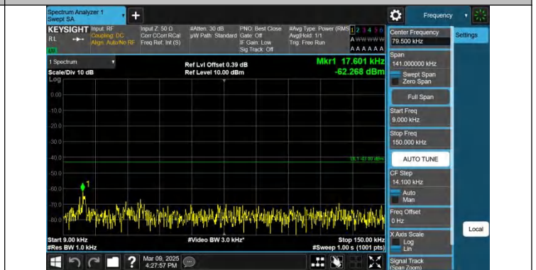
Band2-5MHz-QPSK-19175-1RB#24-0.009~0.15-PASS
