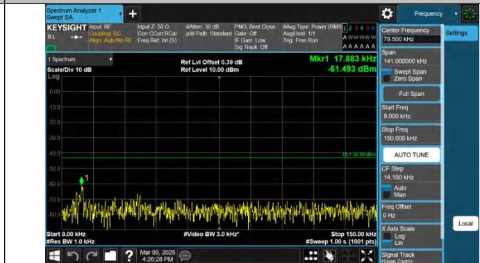
Band2-5MHz-QPSK-18900-1RB#24-0.009~0.15-PASS
