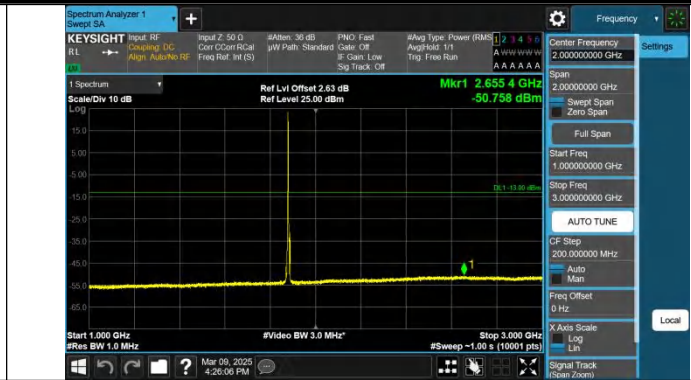
Band2-5MHz-QPSK-18900-1RB#0-1000~3000-PASS
