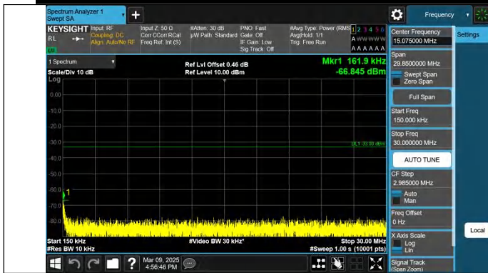
Band2-20MHz-QPSK-19100-1RB#99-0.15~30-PASS
