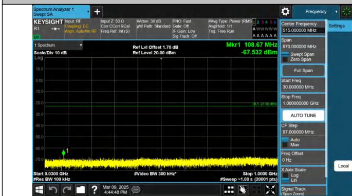
Band2-15MHz-QPSK-18675-1RB#0-30~1000-PASS
