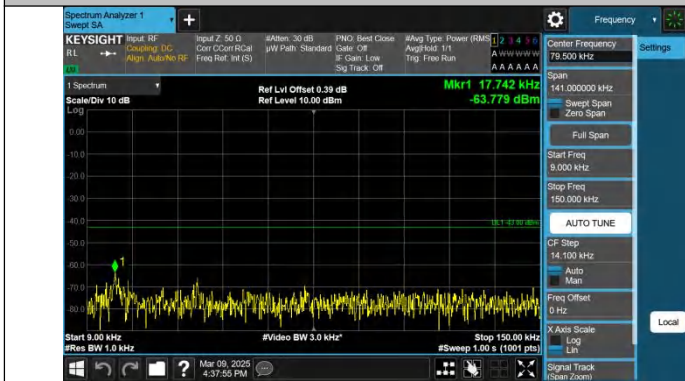
Band2-10MHz-QPSK-18900-1RB#49.0.009~0.15-PASS
