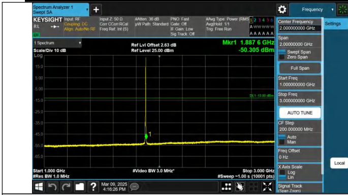
Band2-3MHz-QPSK-18900-1RB#14-1000~3000-PASS
