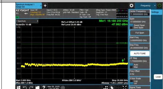
Band2-20MHz-QPSK-18700-1RB#99.3000~20000-PASS
