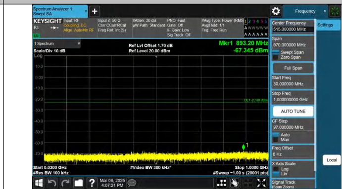
Band2-1.4MHz-QPSK-19193-1RB#5-30~1000-PASS
