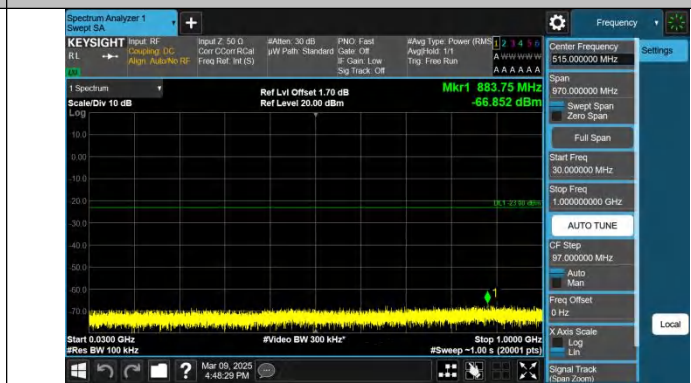
Band2-15MHz-QPSK-19125-1RB#74.30~1000-PASS
