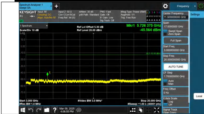
Band2-1.4MHz-QPSK-19193-1RB#0-3000~20000-PASS
