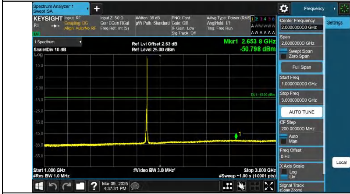
Band2-10MHz-QPSK-18900-1RB#49.1000~3000-PASS
