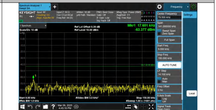
Band2-15MHz-QPSK-18675-1RB#74-0.09~0.15-PASS
