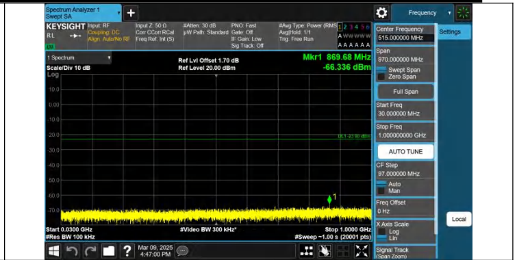
Band2-15MHz-QPSK-18900-1RB#74-30~1000-PASS
