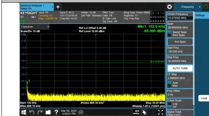
Band2-15MHz-QPSK-19125-1RB#74.0.15~30-PASS
