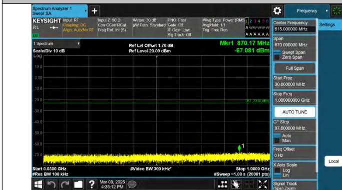
Band2-10MHz-QPSK-18650-1RB#0-30~1000-PASS
