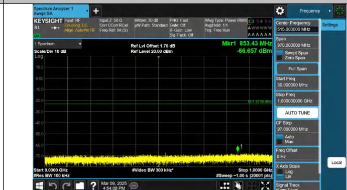
Band2-20MHz-QPSK-18700-1RB#99.30~1000-PASS
