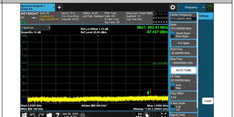
Band2-3MHz-QPSK-18900-1RB#14-30~1000-PASS
