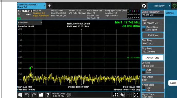
Band2-3MHz-QPSK-18615-1RB#14-0.009~0.15-PASS
