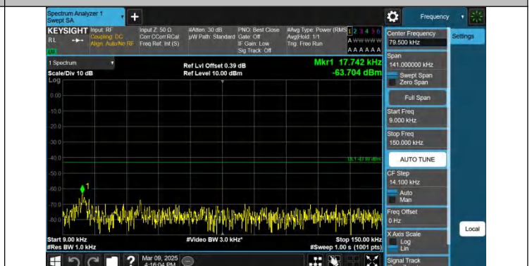
Band2-3MHz-QPSK-18900-1RB#14-0.009~0.15-PASS
