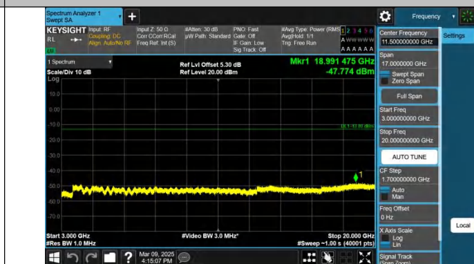
Band2-3MHz-QPSK-18615-1RB#14-3000~20000-PASS
