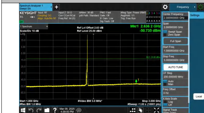
Band2-10MHz-QPSK-19150-1RB#49.1000~3000-PASS
