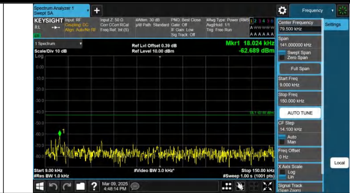
Band2-15MHz-QPSK-19125-1RB#74.0.009~0.15-PASS
