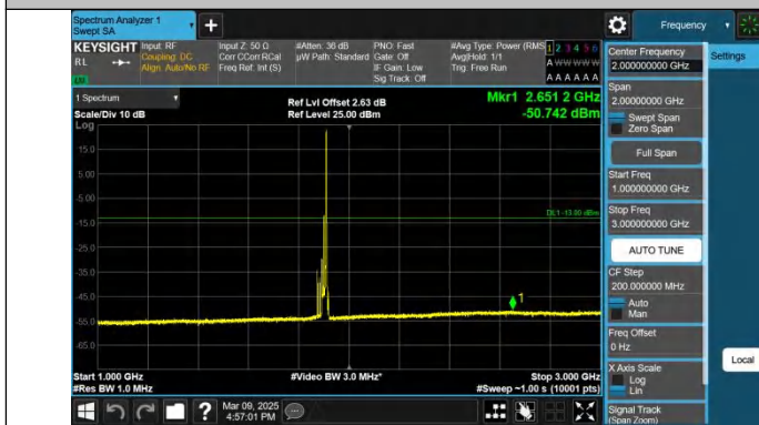
Band2-20MHz-QPSK-19100-1RB#99-1000~3000-PASS
