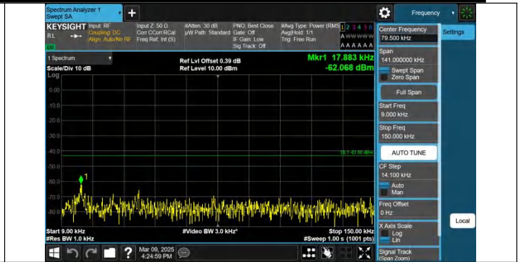
Band2-5MHz-QPSK-18625-1RB#24-0.009~0.15-PASS
