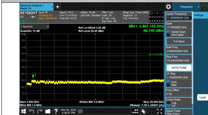
Band2-10MHz-QPSK-19150-1RB#0-3000~20000-PASS
