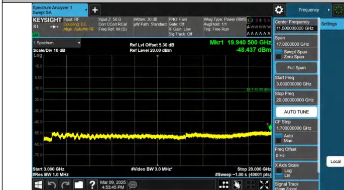
Band2-20MHz-QPSK-18700-1RB#0-3000~20000-PASS
