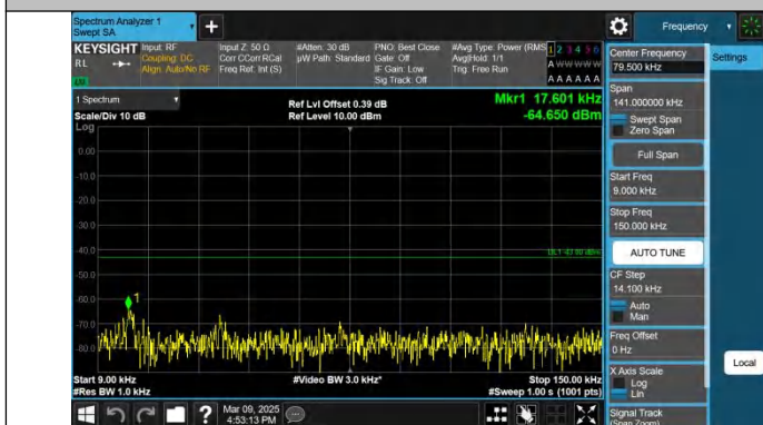
Band2-20MHz-QPSK-18700-1RB#0-0.009~0.15-PASS
