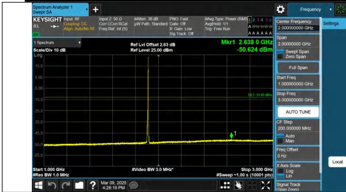
Band2-5MHz-QPSK-19175-1RB#24-1000~3000-PASS
