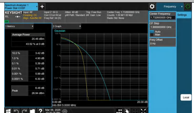
Band4-1413-3-PASS
