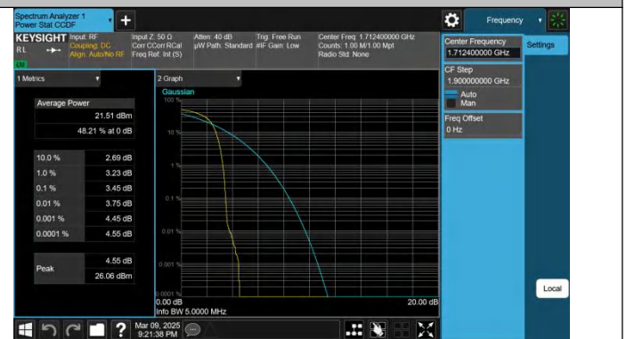
Band4-1312-2-PASS
