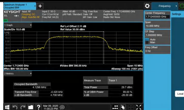
Band4-1312-4-PASS
