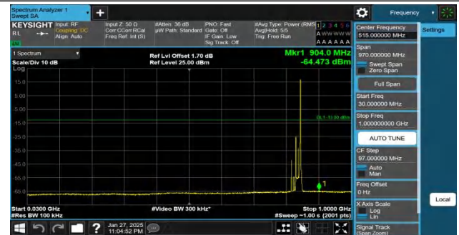
Band26(824-849)-15MHz-QPSK-26965-1RB#74-30~1000-PASS
