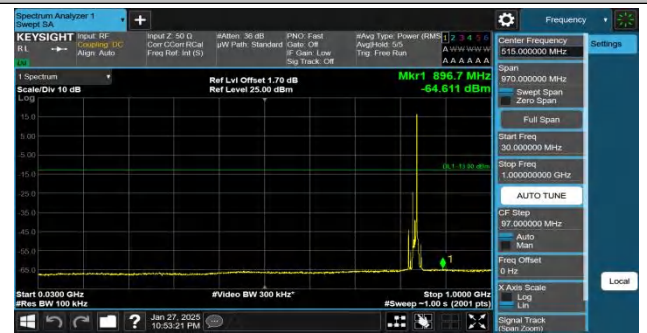
Band26(824-849)-10MHz-QPSK-26915-1RB#49-30~1000-PASS
