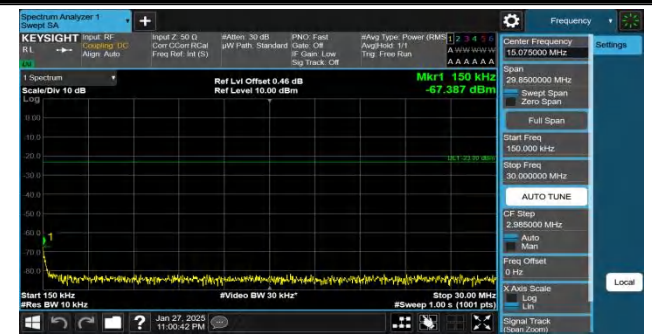
Band26(824-849)-15MHz-QPSK-26865-1RB#0-0.15~30-PASS
