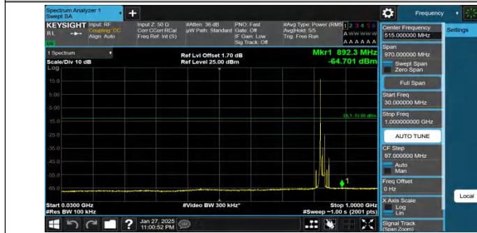
Band26(824-849)-15MHz-QPSK-26865-1RB#0-30~1000-PASS
