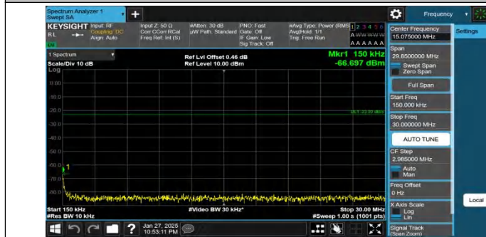
Band26(824-849)-10MHz-QPSK-26915-1RB#49-0.15~30-PASS
