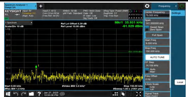
Band26(824-849)-10MHz-QPSK-26915-1RB#49-0.009~0.15-PASS
