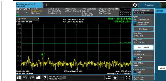
Band26(824-849)-15MHz-QPSK-26865-1RB#0-0.009~0.15-PASS
