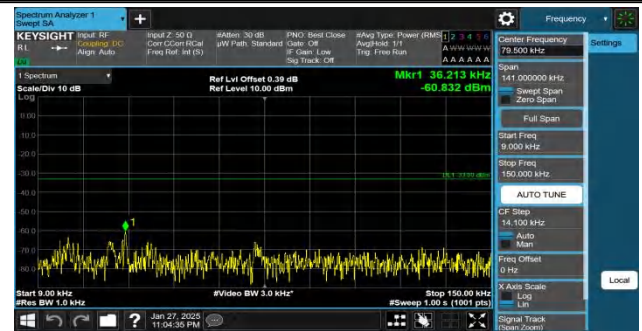
Band26(824-849)-15MHz-QPSK-26965-1RB#74-0.009~0.15-PASS
