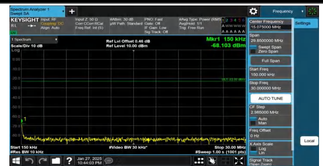
Band26(824-849)-5MHz-QPSK-27015-1RB#0-0.15~30-PASS
