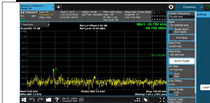
Band26(824-849)-5MHz-QPSK-27015-1RB#0-0.009~0.15-PASS
