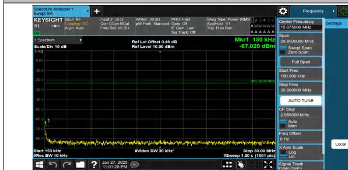
Band26(824-849)-15MHz-QPSK-26865-1RB#74-0.15~30-PASS
