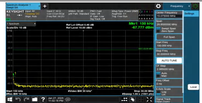
Band26(824-849)-15MHz-QPSK-26915-1RB#0-0.15~30-PASS
