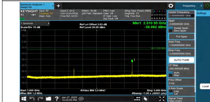
Band26(824-849)-1.4MHz-QPSK-26915-1RB#5-1000~3000-PASS
