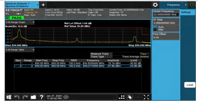
Band26(824-849)-15MHz-QPSK-26965-1RB#0-PASS
