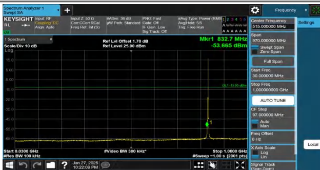
Band26(824-849)-1.4MHz-QPSK-26915-1RB#0-30~1000-PASS
