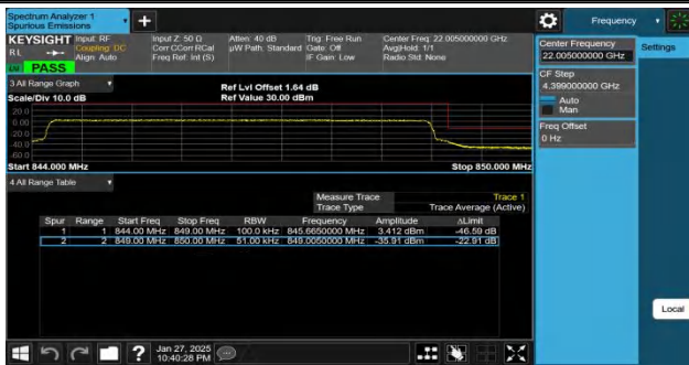
Band26(824-849)-5MHz-QPSK-27015-25RB#0-PASS
