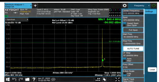
Band26(824-849)-1.4MHz-QPSK-26915-1RB#5-30~1000-PASS
