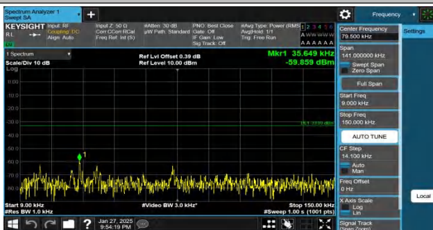
Band26(814-824)-3MHz-QPSK-26705-1RB#0-0.009~0.15-PASS
