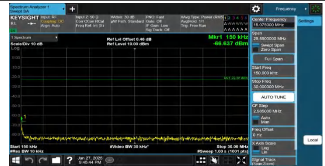
Band26(814-824)-1.4MHz-QPSK-26740-1RB#0-0.15~30-PASS
