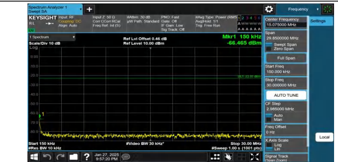
Band26(814-824)-3MHz-QPSK-26775-1RB#0-0.15~30-PASS
