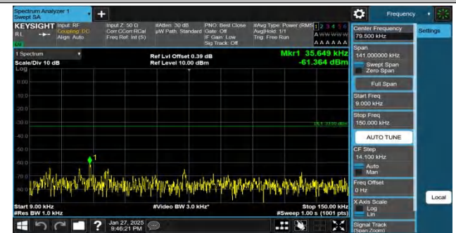
Band26(814-824)-1.4MHz-QPSK-26740-1RB#5-0.009~0.15-PASS
