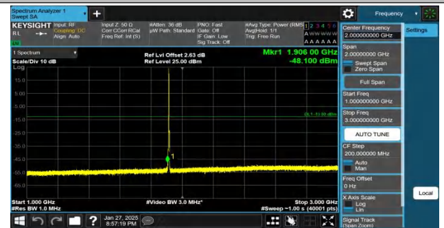
Band25-3MHz-QPSK-26675-1RB#0-1000~3000-PASS
