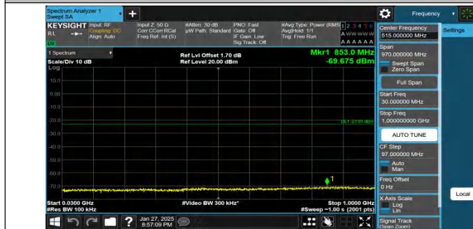
Band25-3MHz-QPSK-26675-1RB#0-0.30~1000-PASS
