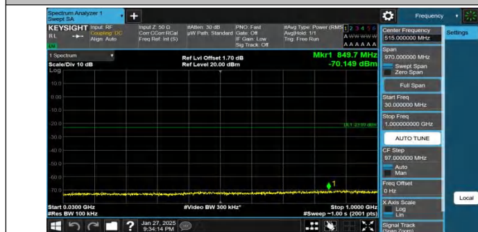
Band25-20MHz-QPSK-26590-1RB#0-30~1000-PASS
