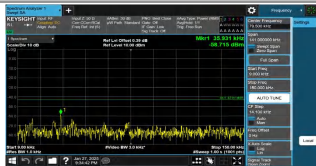
Band25-20MHz-QPSK-26590-1RB#99-0.009~0.15-PASS
