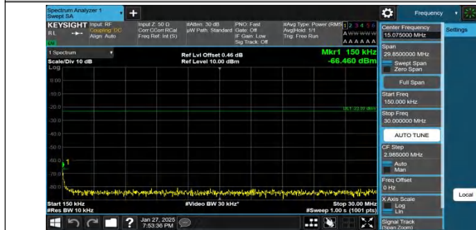
Band12-1.4MHz-QPSK-23173-1RB#5-0.15~30-PASS
