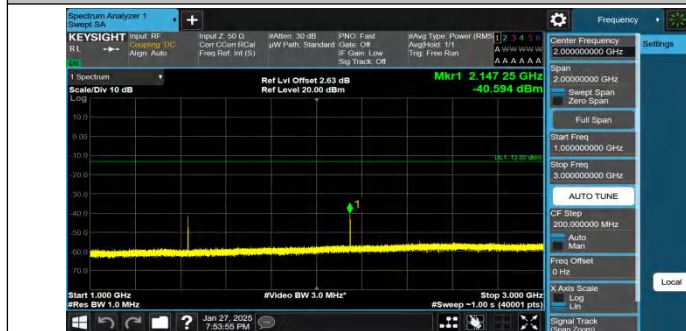
Band12-1.4MHz-QPSK-23173-1RB#5-1000~3000-PASS
