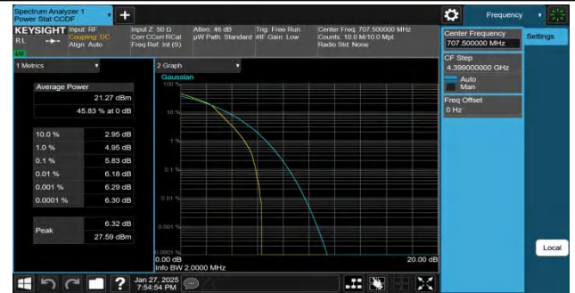
Band12-1.4MHz-16QAM-23095-6RB#0-PASS
