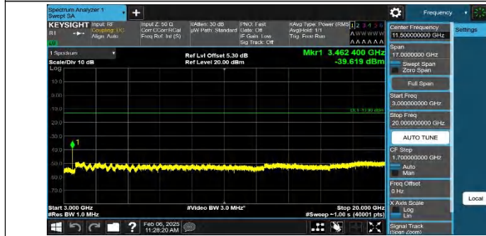
Band4-3MHz-QPSK-20175-1RB#0-3000~20000-PASS
