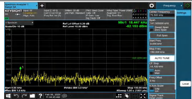
Band4-20MHz-QPSK-20050-1RB#99-0.009~0.15-PASS
