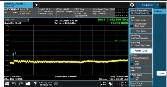
Band4-20MHz-QPSK-20175-1RB#99-3000~20000-PASS
