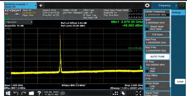
Band4-10MHz-QPSK-20350-1RB#0-1000~3000-PASS
