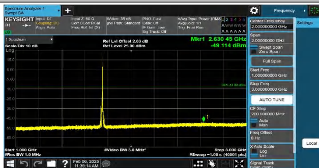
Band4-10MHz-QPSK-20350-1RB#49-1000~3000-PASS
