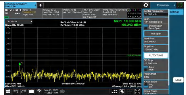
Band4-3MHz-QPSK-20175-1RB#14-0.009~0.15-PASS
