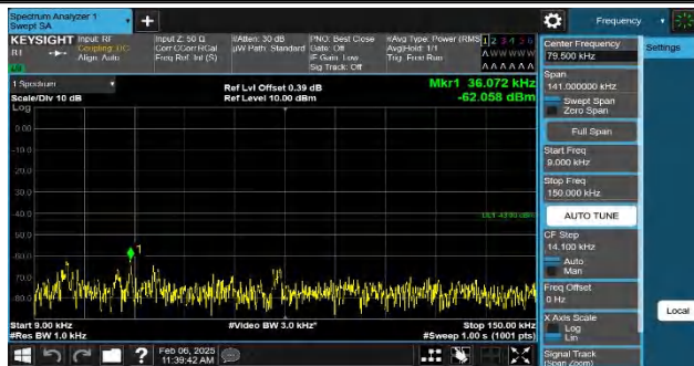
Band4-15MHz-QPSK-20025-1RB#0-0.009~0.15-PASS
