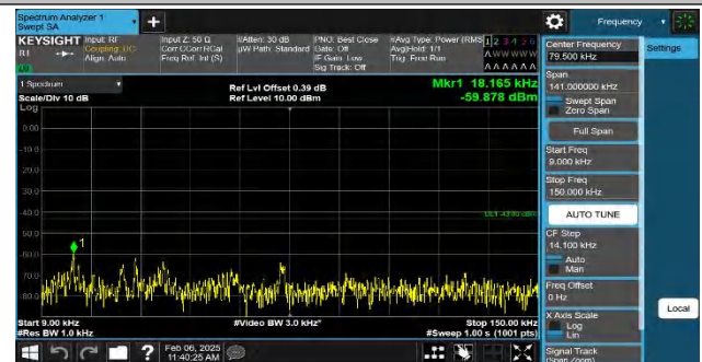
Band4-15MHz-QPSK-20025-1RB#74-0.009~0.15-PASS
