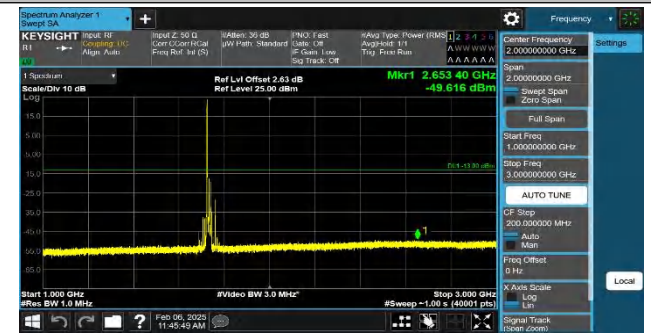
Band4-20MHz-QPSK-20175-1RB#0-1000~3000-PASS
