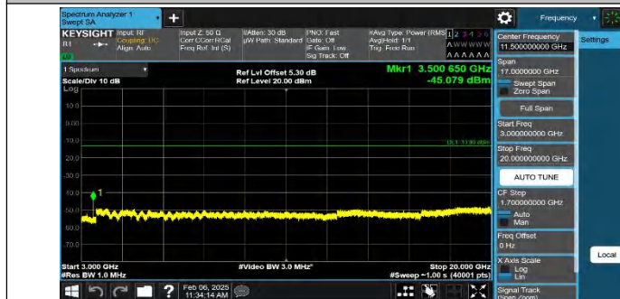
Band4-5MHz-QPSK-20375-1RB#0-3000~20000-PASS
