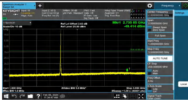
Band4-5MHz-QPSK-20375-1RB#24-1000~3000-PASS
