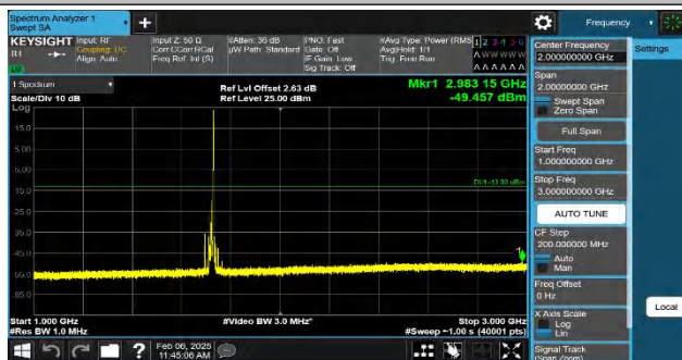
Band4-20MHz-QPSK-20050-1RB#99-1000~3000-PASS
