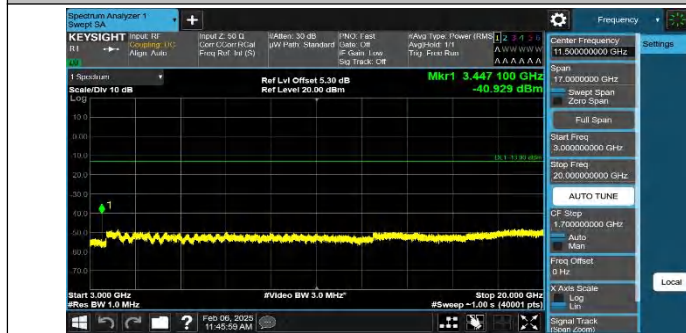
Band4-20MHz-QPSK-20175-1RB#0-3000~20000-PASS
