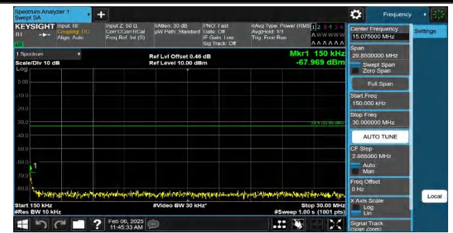
Band4-20MHz-QPSK-20175-1RB#0-0.15~30-PASS
