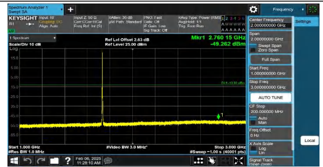
Band4-3MHz-QPSK-20175-1RB#0-1000~3000-PASS
