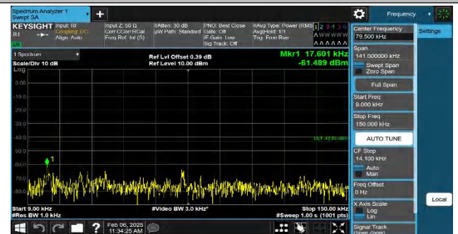
Band4-5MHz-QPSK-20375-1RB#24-0.009~0.15-PASS
