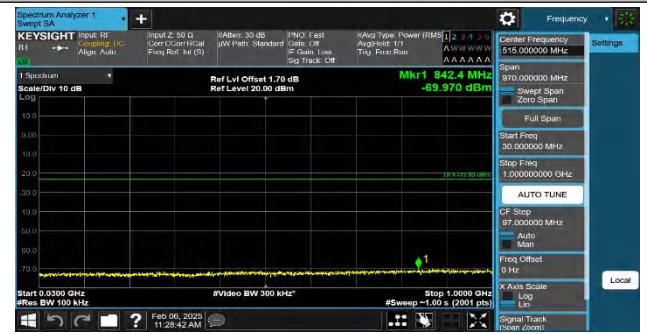
Band4-3MHz-QPSK-20175-1RB#14-30~1000-PASS
