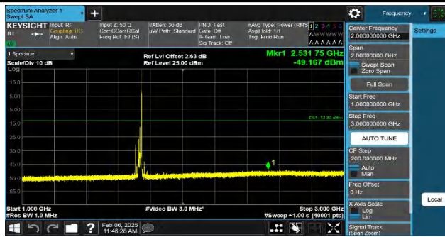
Band4-20MHz-QPSK-20175-1RB#99-1000~3000-PASS
