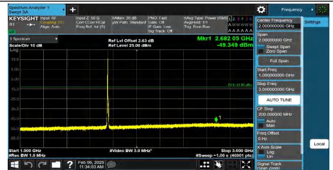
Band4-5MHz-QPSK-20375-1RB#0-1000~3000-PASS
