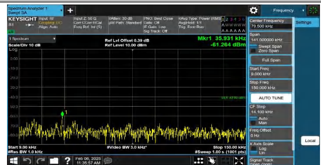
Band4-10MHz-QPSK-20000-1RB#49-0.009~0.15-PASS
