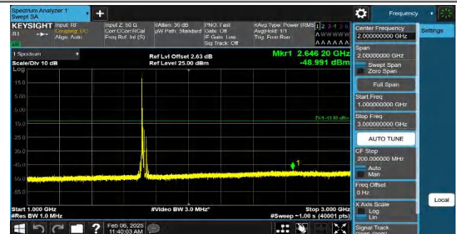
Band4-15MHz-QPSK-20025-1RB#0-1000~3000-PASS
