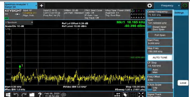
Band4-10MHz-QPSK-20350-1RB#49-0.009~0.15-PASS
