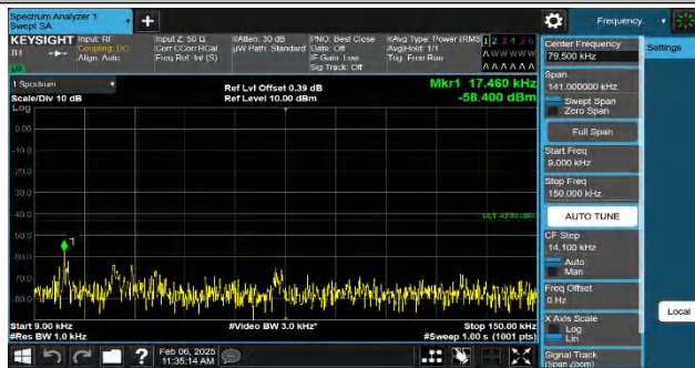
Band4-10MHz-QPSK-20000-1RB#0-0.009~0.15-PASS
