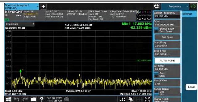
Band4-20MHz-QPSK-20300-1RB#99-0.009~0.15-PASS
