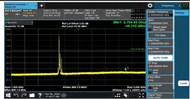
Band4-20MHz-QPSK-20050-1RB#0-1000~3000-PASS
