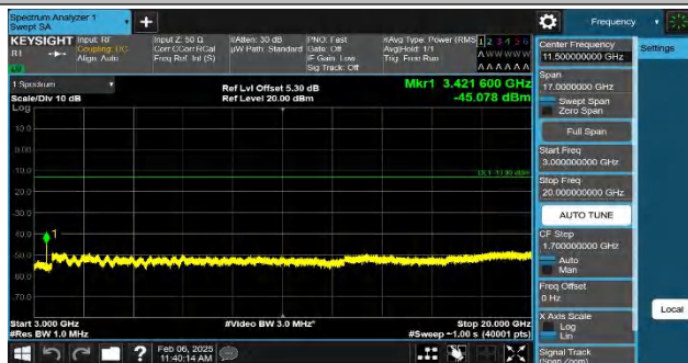
Band4-15MHz-QPSK-20025-1RB#0-3000~20000-PASS
