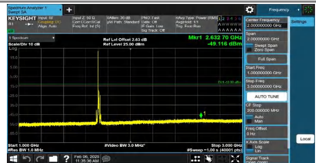
Band4-10MHz-QPSK-20000-1RB#0-1000~3000-PASS
