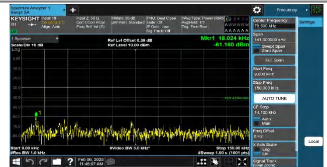
Band4-20MHz-QPSK-20175-1RB#99-0.009~0.15-PASS
