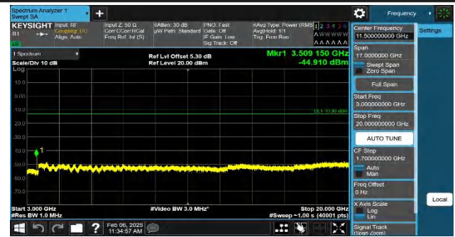
Band4-5MHz-QPSK-20375-1RB#24-3000~20000-PASS
