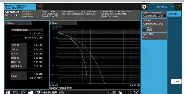
Band4-10MHz-16QAM-20175-50RB#0-PASS
