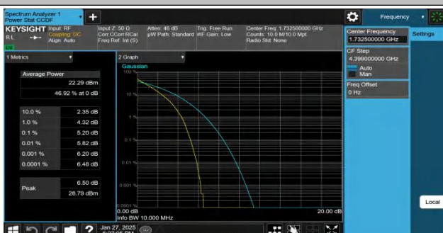
Band4-10MHz-QPSK-20175-50RB#0-PASS
