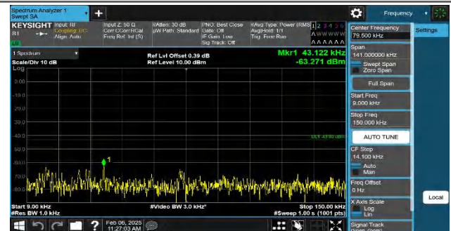
Band4-3MHz-QPSK-19965-1RB#14-0.009~0.15-PASS
