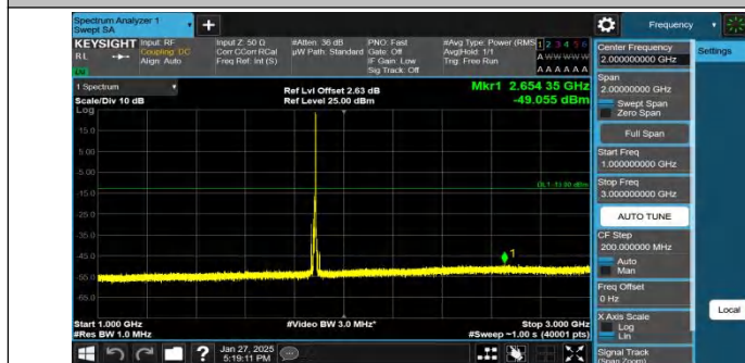
Band2-10MHz-QPSK-18900-1RB#49-1000~3000-PASS
