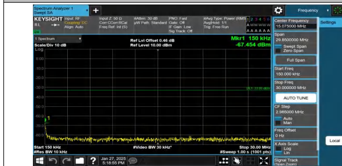
Band2-10MHz-QPSK-18900-1RB#49-0.15~30-PASS
