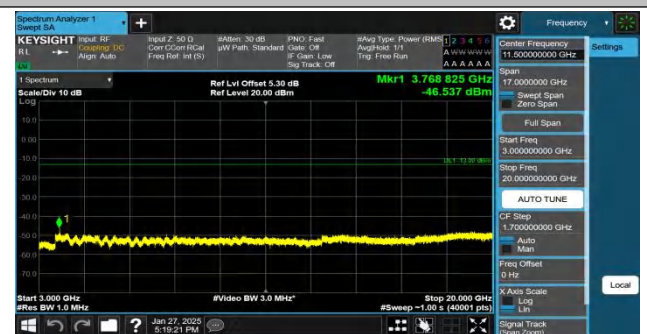
Band2-10MHz-QPSK-18900-1RB#49-3000~20000-PASS
