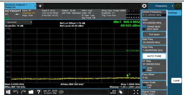
Band2-10MHz-QPSK-18900-1RB#49-30~1000-PASS
