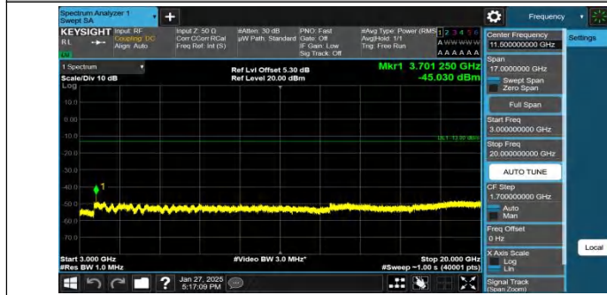
Band2-10MHz-QPSK-18650-1RB#0-3000~20000-PASS
