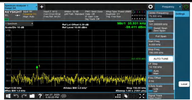
Band2-15MHz-QPSK-19125-1RB#74-0.009~0.15-PASS
