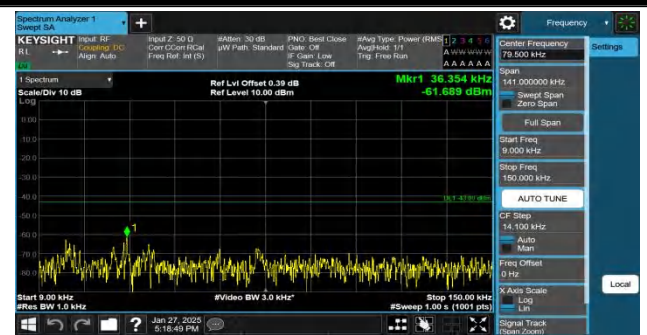
Band2-10MHz-QPSK-18900-1RB#49-0.009~0.15-PASS
