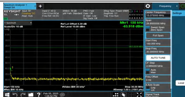
Band5-4182-1-0.15~30MHz-PASS
