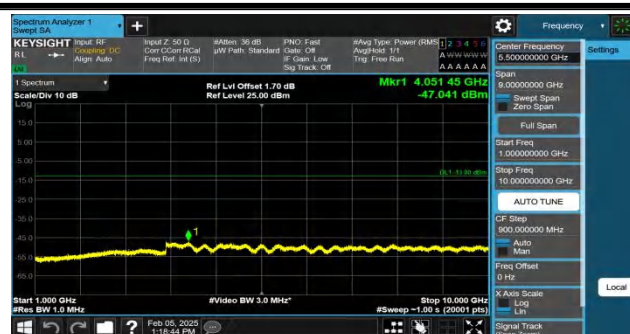
Band5-4132-5-1000~10000MHz-PASS
