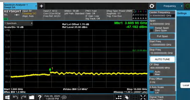
Band5-4182-1-1000~10000MHz-PASS
