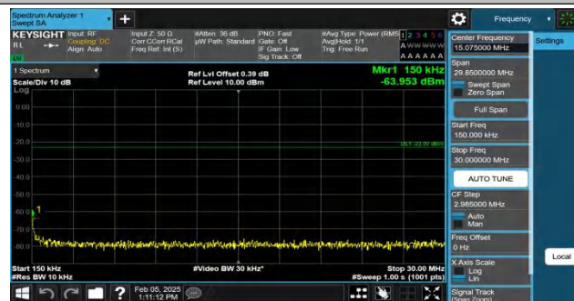
Band5-4182-2-0.15~30MHz-PASS
