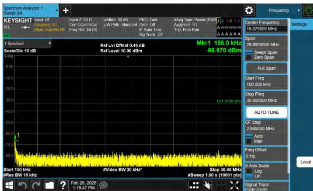
Band66-1.4MHz-QPSK-132665-1RB#5-0.15~30-PASS
