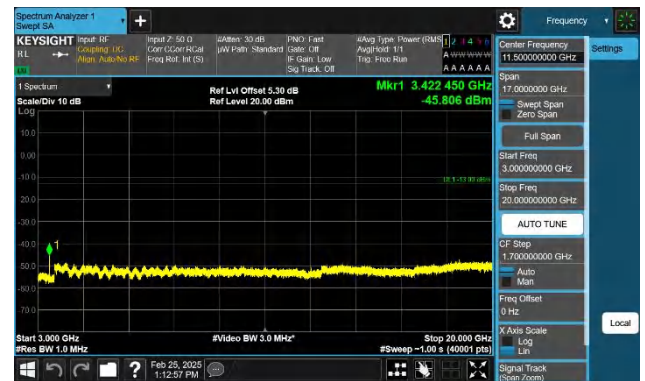
Band66-1.4MHz-QPSK-131979-1RB#5-3000~20000-PASS
