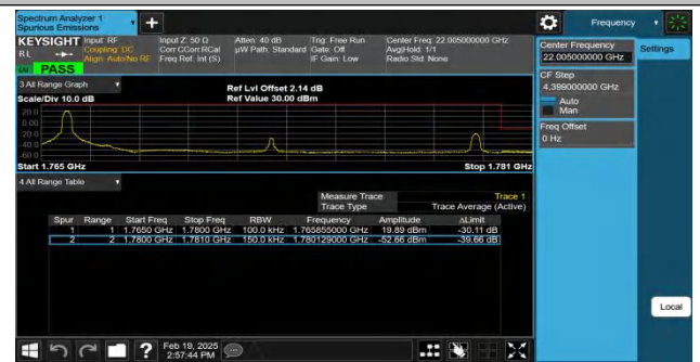
Band66-15MHz-QPSK-132597-1RB#0-PASS
