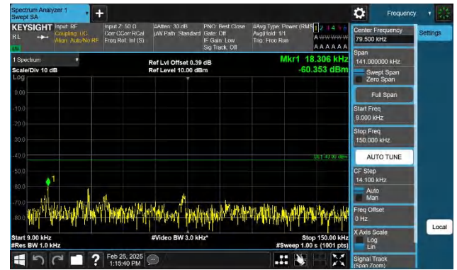
Band66-1.4MHz-QPSK-132665-1RB#5-0.009~0.15-PASS
