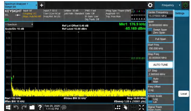
Band66-1.4MHz-QPSK-131979-1RB#0-0.15~30-PASS
