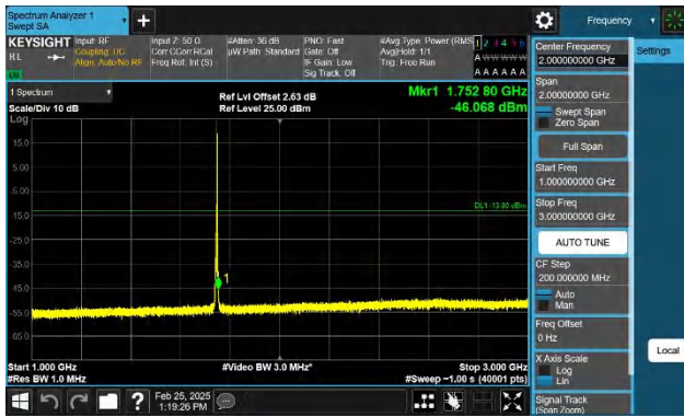
Band66-3MHz-QPSK-132322-1RB#14-1000~3000-PASS
