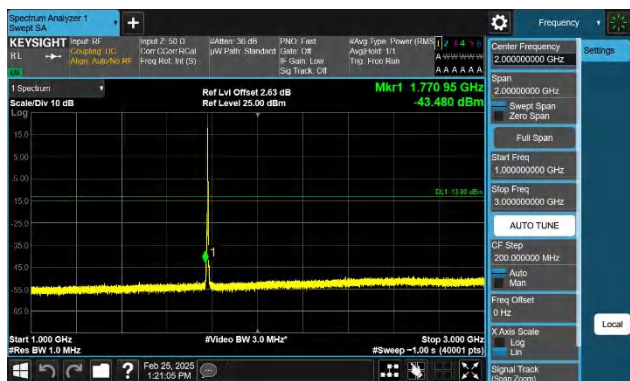
Band66-3MHz-QPSK-132657-1RB#14-1000~3000-PASS
