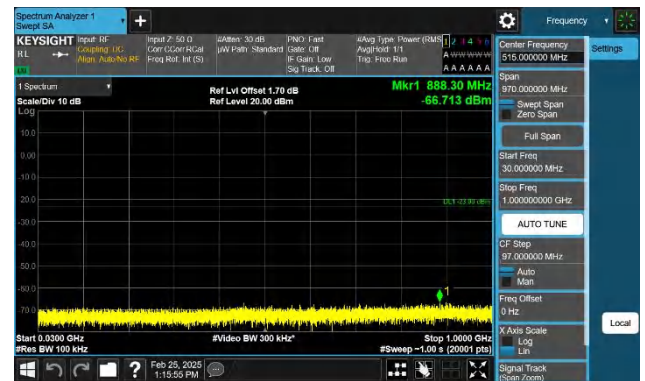
Band66-1.4MHz-QPSK-132665-1RB#5-30~1000-PASS
