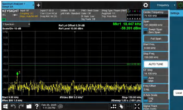
Band66-1.4MHz-QPSK-131979-1RB#0-0.009~0.15-PASS
