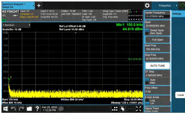
Band66-1.4MHz-QPSK-131979-1RB#5-0.15~30-PASS
