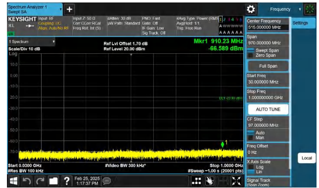
Band66-3MHz-QPSK-131987-1RB#14-30~1000-PASS
