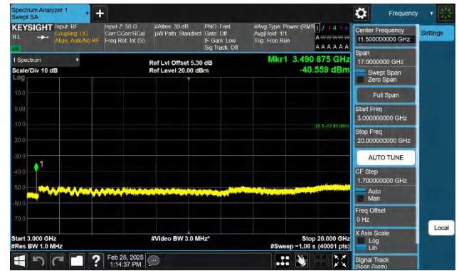
Band66-1.4MHz-QPSK-132322-1RB#5-3000~20000-PASS
