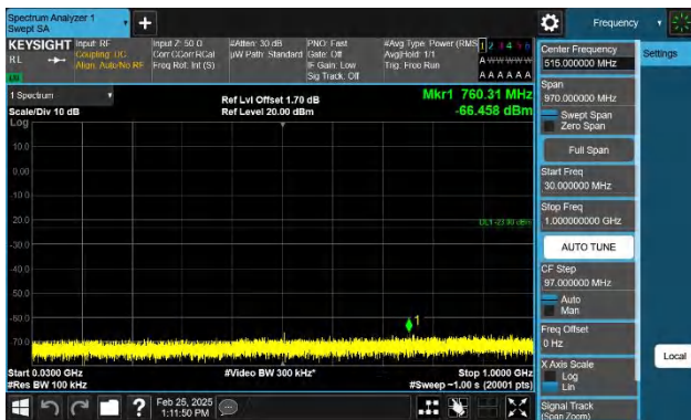
Band66-1.4MHz-QPSK-131979-1RB#0-30~1000-PASS
