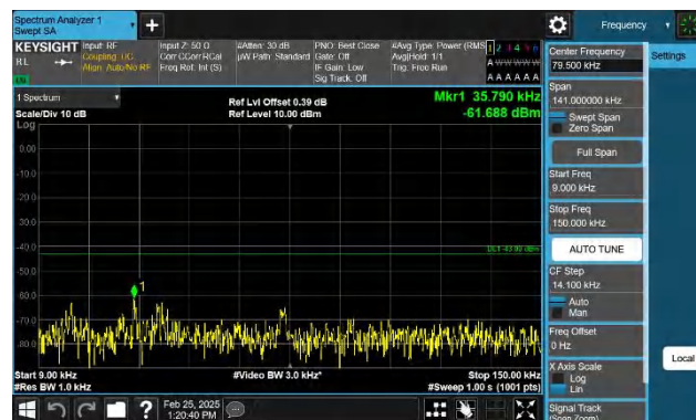
Band66-3MHz-QPSK-132657-1RB#14-0.009~0.15-PASS
