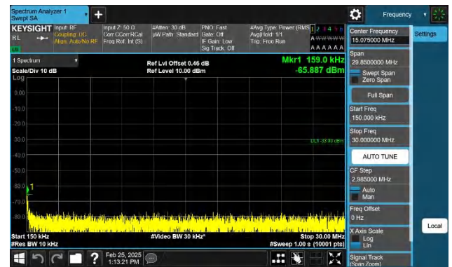
Band66-1.4MHz-QPSK-132322-1RB#0-0.15~30-PASS
