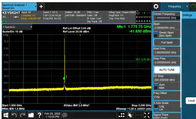
Band66-1.4MHz-QPSK-132665-1RB#5-1000~3000-PASS
