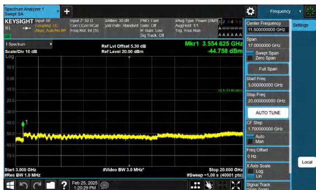
Band66-3MHz-QPSK-132657-1RB#0-3000~20000-PASS
