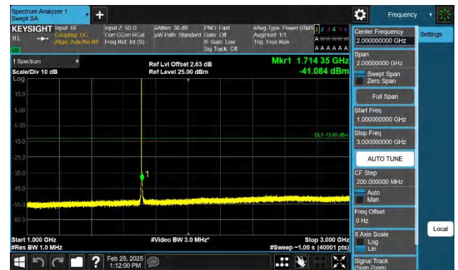
Band66-1.4MHz-QPSK-131979-1RB#0-1000~3000-PASS
