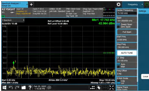
Band66-3MHz-QPSK-131987-1RB#0-0.009~0.15-PASS
