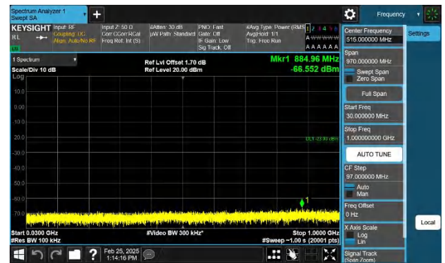
Band66-1.4MHz-QPSK-132322-1RB#5-30~1000-PASS
