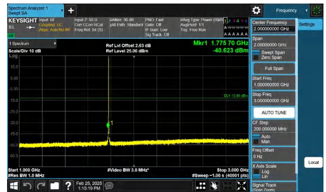
Band66-1.4MHz-QPSK-132665-1RB#0-1000~3000-PASS
