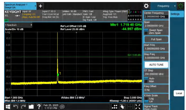
Band66-3MHz-QPSK-131987-1RB#0-1000~3000-PASS
