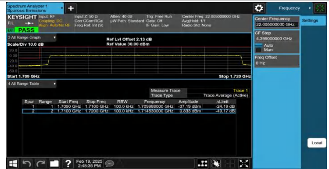
Band66-10MHz-QPSK-132022-50RB#0-PASS
