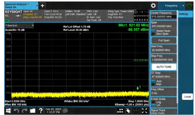
Band66-1.4MHz-QPSK-131979-1RB#5-30~1000-PASS
