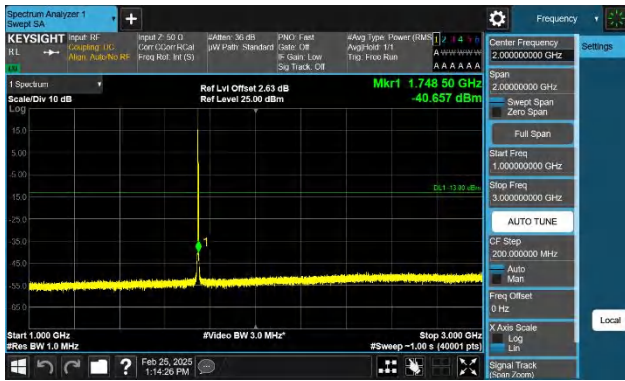
Band66-1.4MHz-QPSK-132322-1RB#5-1000~3000-PASS
