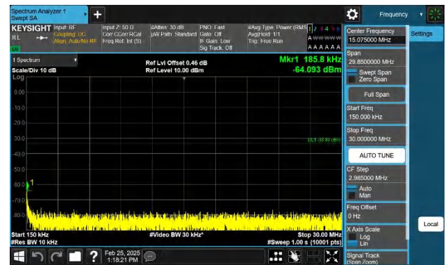
Band66-3MHz-QPSK-132322-1RB#0-0.15~30-PASS
