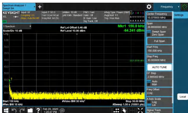
Band66-3MHz-QPSK-132657-1RB#14-0.15~30-PASS
