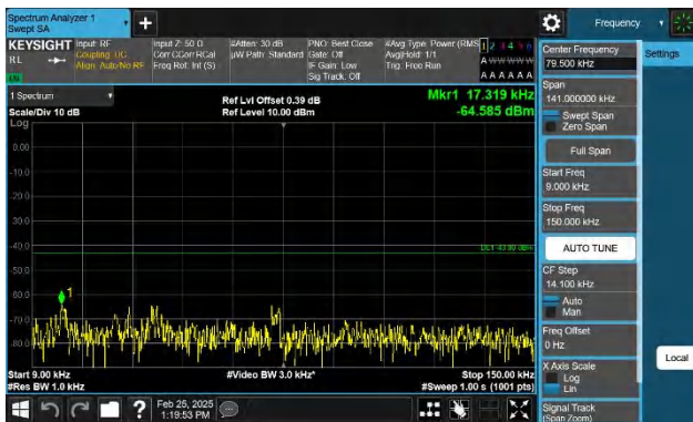
Band66-3MHz-QPSK-132657-1RB#0-0.009~0.15-PASS
