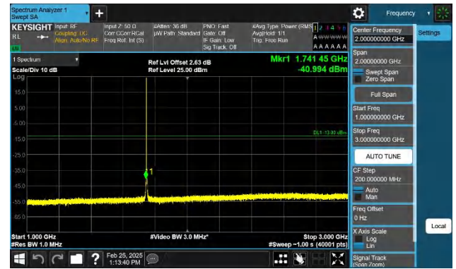
Band66-1.4MHz-QPSK-132322-1RB#0-1000~3000-PASS
