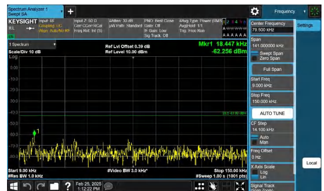
Band66-1.4MHz-QPSK-131979-1RB#5-0.009~0.15-PASS
