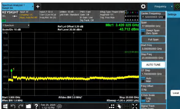
Band66-1.4MHz-QPSK-131979-1RB#0-3000~20000-PASS
