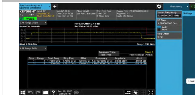
Band66-15MHz-QPSK-132597-75RB#0-PASS
