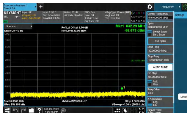
Band66-3MHz-QPSK-132657-1RB#14-30~1000-PASS
