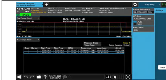
Band66-20MHz-QPSK-132572-100RB#0-PASS
