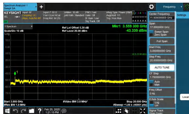
Band66-3MHz-QPSK-132657-1RB#14-3000~20000-PASS
