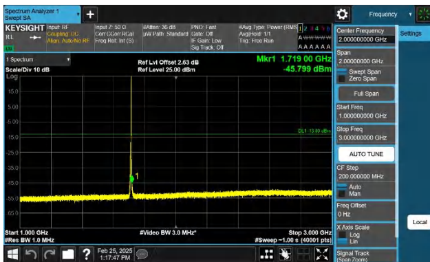
Band66-3MHz-QPSK-131987-1RB#14-1000~3000-PASS
