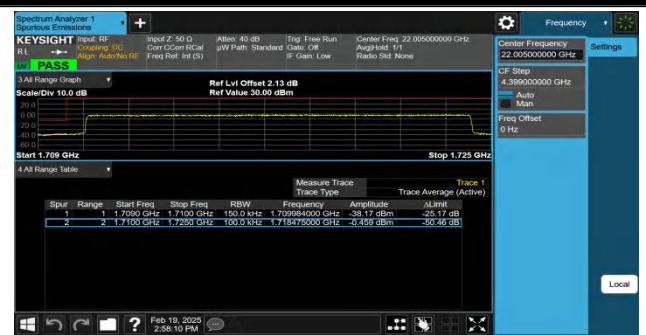
Band66-15MHz-QPSK-132047-75RB#0-PASS
