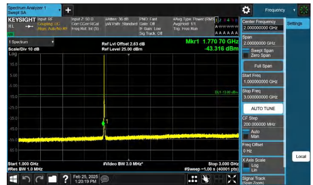
Band66-3MHz-QPSK-132657-1RB#0-1000~3000-PASS
