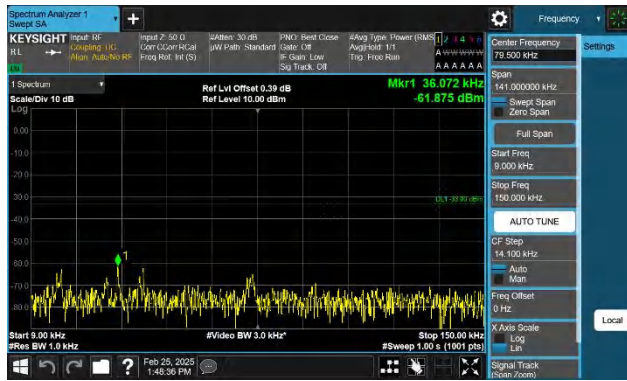
Band14-5MHz-QPSK-23355-1RB#24-0.009~0.15-PASS
