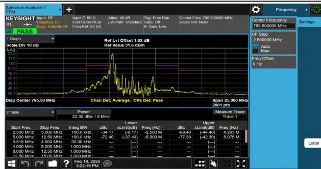
NTNV-Band14-5MHz-QPSK-23355-1RB#0-2.50-5.00-PASS
