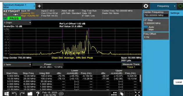
NTNV-Band14-10MHz-QPSK-23330-1RB#49-10.00-25.00-PASS
