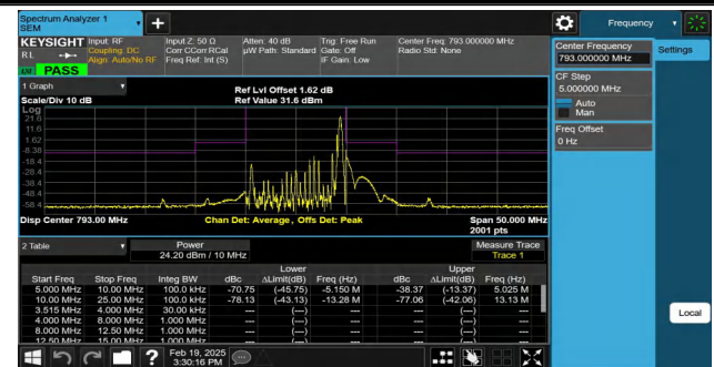
NTNV-Band14-10MHz-QPSK-23330-1RB#49-5.00-10.00-PASS
