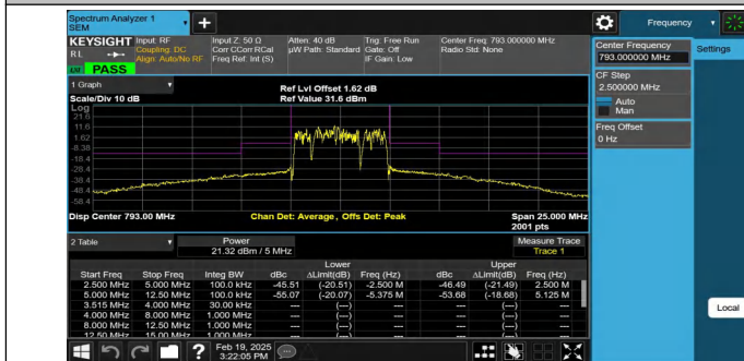
NTNV-Band14-5MHz-16QAM-23330-25RB#0--2.50-2.50-PASS
