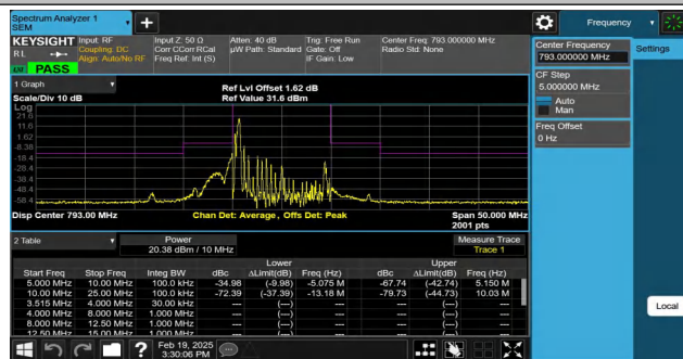
NTNV-Band14-10MHz-16QAM-23330-1RB#0-10.00-25.00-PASS
