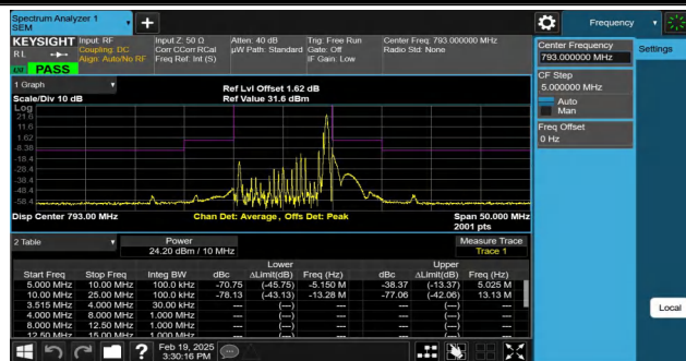
NTNV-Band14-10MHz-QPSK-23330-1RB#49--10.00--5.00-PASS
