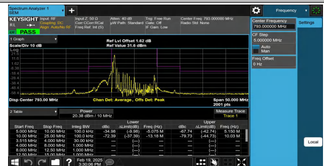
NTNV-Band14-10MHz-16QAM-23330-1RB#0--25.00--10.00-PASS
