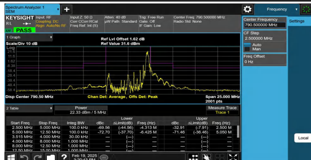
NTNV-Band14-5MHz-QPSK-23305-1RB#24--12.50--5.00-PASS
