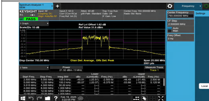
NTNV-Band14-5MHz-16QAM-23330-25RB#0--12.50--5.00-PASS
