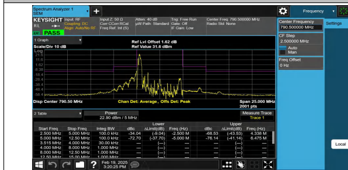
NTNV-Band14-5MHz-QPSK-23305-1RB#0-2.50-5.00-PASS
