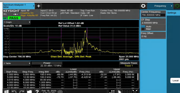
NTNV-Band14-5MHz-QPSK-23305-1RB#24--2.50-2.50-PASS
