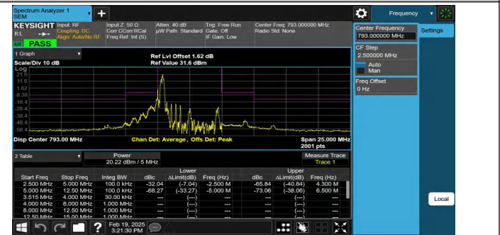
NTNV-Band14-5MHz-16QAM-23330-1RB#0-5.00-12.50-PASS
