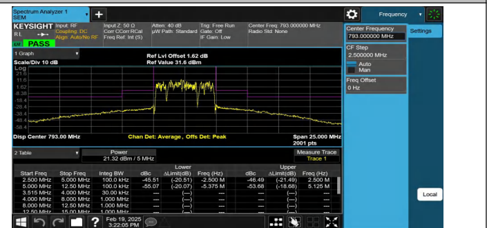
NTNV-Band14-5MHz-16QAM-23330-25RB#0-5.00-12.50-PASS
