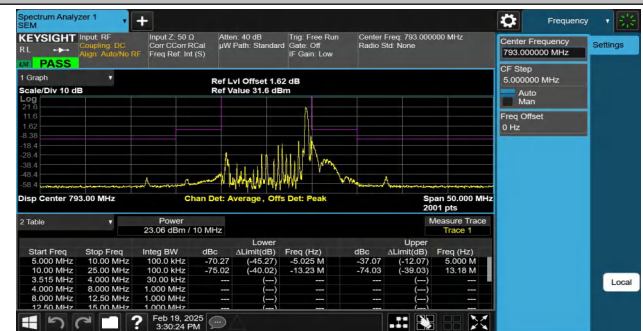
NTNV-Band14-10MHz-16QAM-23330-1RB#49--25.00--10.00-PAS
