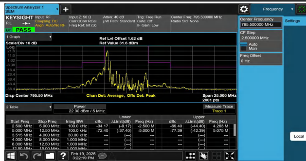
NTNV-Band14-5MHz-QPSK-23355-1RB#0--12.50--5.00-PASS
