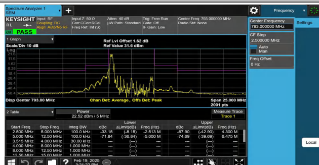
NTNV-Band14-5MHz-QPSK-23330-1RB#0-2.50-5.00-PASS
