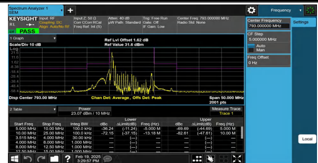
NTNV-Band14-10MHz-QPSK-23330-1RB#0--5.00-5.00-PASS
