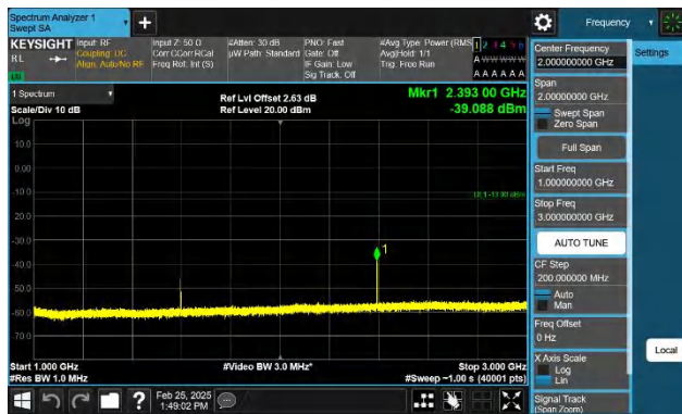
Band14-5MHz-QPSK-23355-1RB#24-1000~3000-PASS
