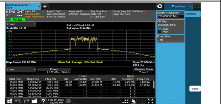
NTNV-Band14-5MHz-16QAM-23330-25RB#0--5.00--2.50-PASS
