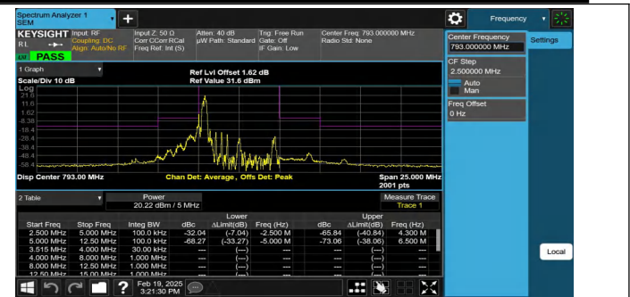
NTNV-Band14-5MHz-16QAM-23330-1RB#0--5.00--2.50-PASS
