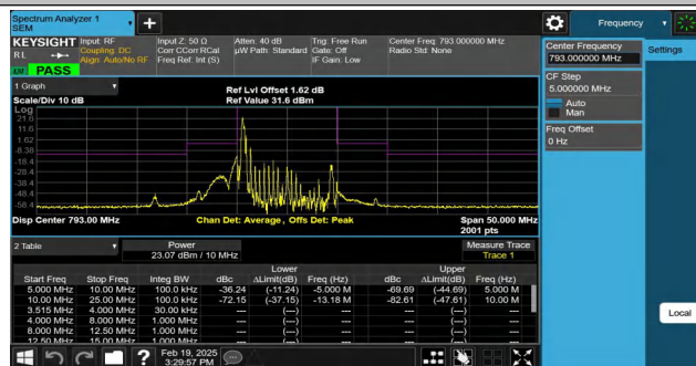
NTNV-Band14-10MHz-QPSK-23330-1RB#0-5.00-10.00-PASS
