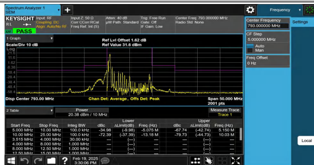
NTNV-Band14-10MHz-16QAM-23330-1RB#0--10.00--5.00-PASS
