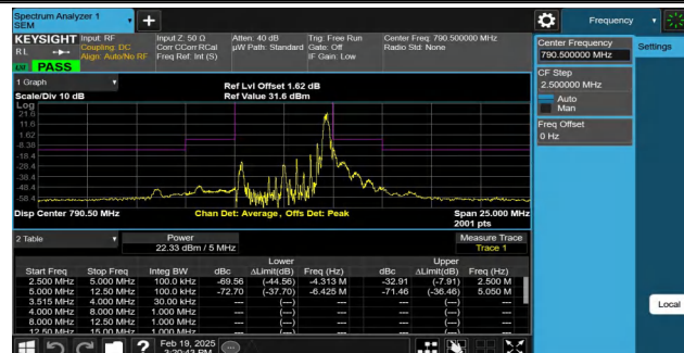
NTNV-Band14-5MHz-QPSK-23305-1RB#24--5.00--2.50-PASS
