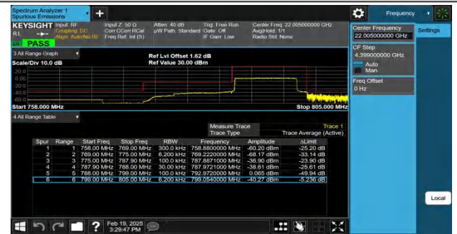
Band14-10MHz-QPSK-23330-50RB#0-PASS
