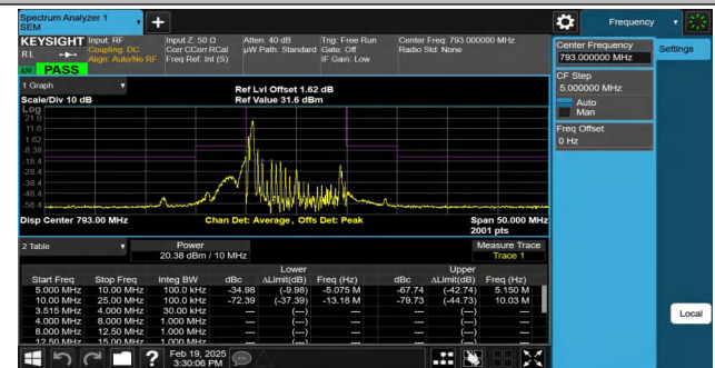
NTNV-Band14-10MHz-16QAM-23330-1RB#0-5.00-10.00-PASS
