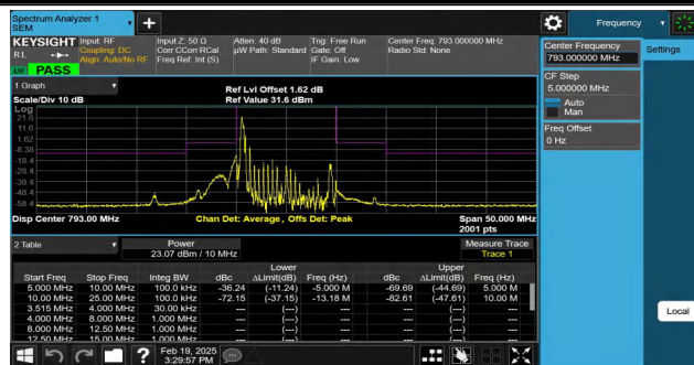
NTNV-Band14-10MHz-QPSK-23330-1RB#0--10.00--5.00-PASS
