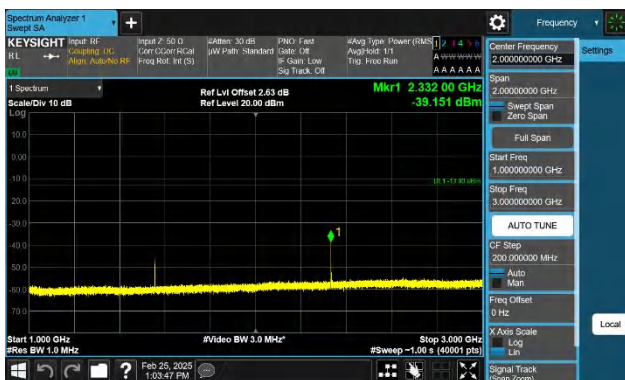
Band13-5MHz-QPSK-23205-1RB#0-1000~3000-PASS
