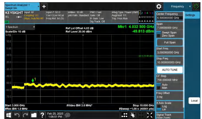
Band13-5MHz-QPSK-23230-1RB#24-3000~10000-PASS
