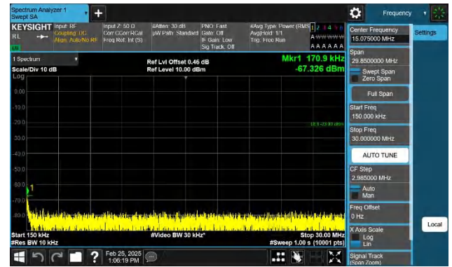
Band13-5MHz-QPSK-23230-1RB#24-0.15~30-PASS
