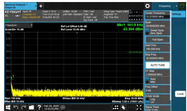
Band12-5MHz-QPSK-23095-1RB#0-0.15~30-PASS
