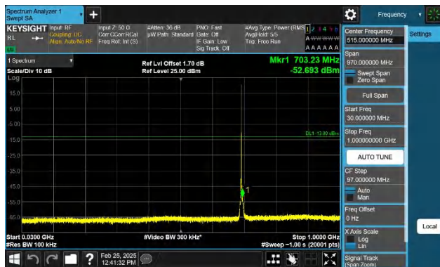
Band12-1.4MHz-QPSK-23017-1RB#0-30~1000-PASS
