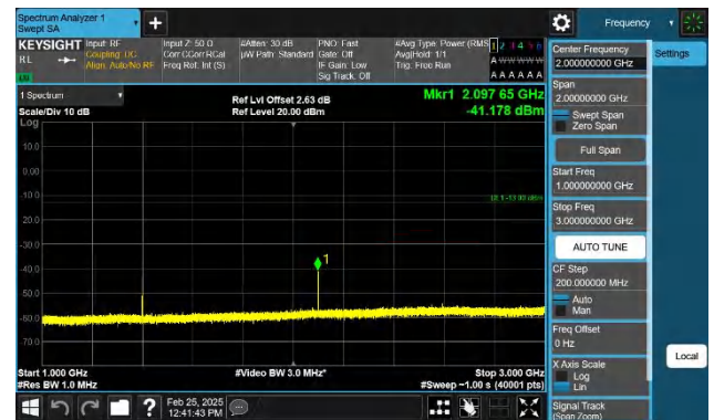
Band12-1.4MHz-QPSK-23017-1RB#0-1000~3000-PASS
