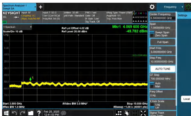
Band12-1.4MHz-QPSK-23017-1RB#0-3000~10000-PASS
