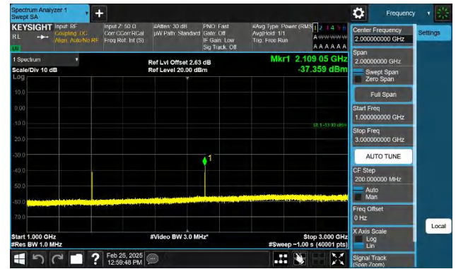
Band12-10MHz-QPSK-23095-1RB#0-1000~3000-PASS
