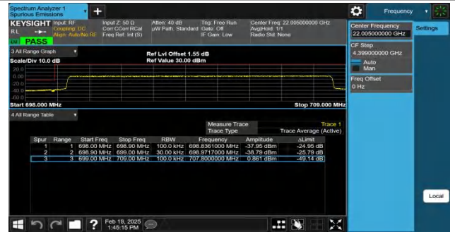
Band12-10MHz-QPSK-23060-50RB#0-PASS
