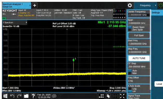
Band12-5MHz-QPSK-23035-1RB#24-1000~3000-PASS
