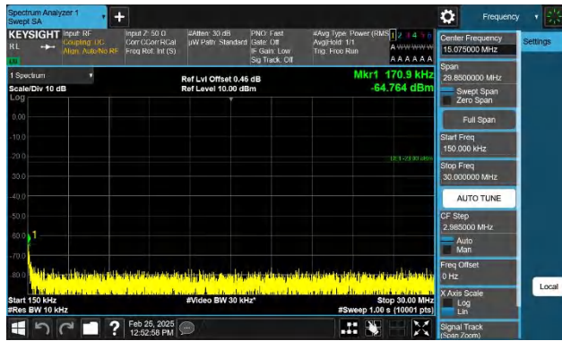
Band12-5MHz-QPSK-23035-1RB#24-0.15~30-PASS
