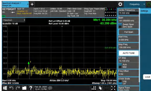
Band12-1.4MHz-QPSK-23017-1RB#0-0.009~0.15-PASS
