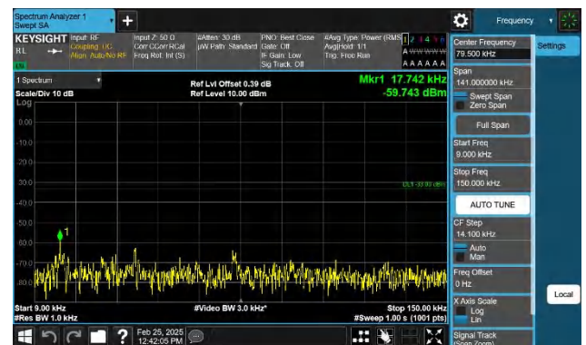
Band12-1.4MHz-QPSK-23017-1RB#5-0.009~0.15-PASS
