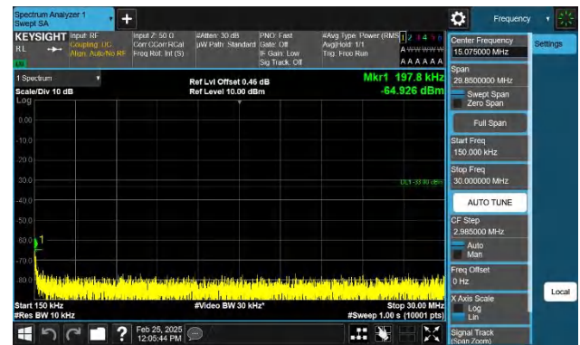
Band4-10MHz-QPSK-20175-1RB#0-0.15~30-PASS
