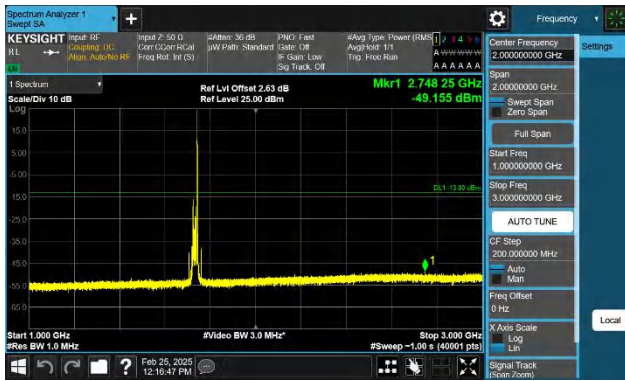
Band4-20MHz-QPSK-20175-1RB#99-1000~3000-PASS
