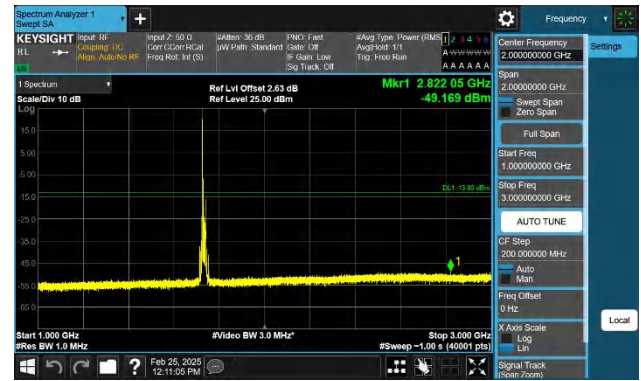
Band4-15MHz-QPSK-20175-1RB#0-1000~3000-PASS
