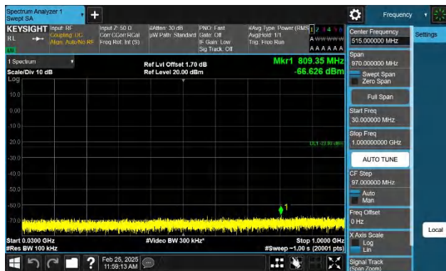
Band4-5MHz-QPSK-19975-1RB#0-30~1000-PASS
