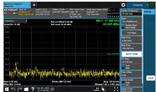
Band4-15MHz-QPSK-20175-1RB#74-0.009~0.15-PASS
