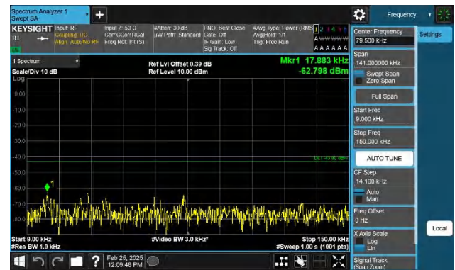
Band4-15MHz-QPSK-20025-1RB#74-0.009~0.15-PASS
