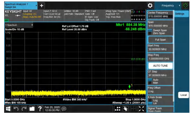
Band4-5MHz-QPSK-19975-1RB#24-30~1000-PASS
