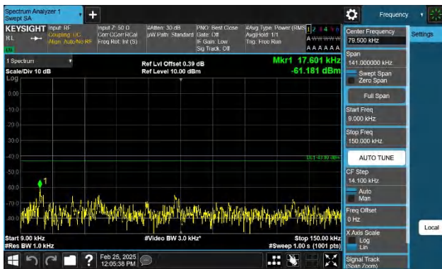
Band4-10MHz-QPSK-20175-1RB#0-0.009~0.15-PASS
