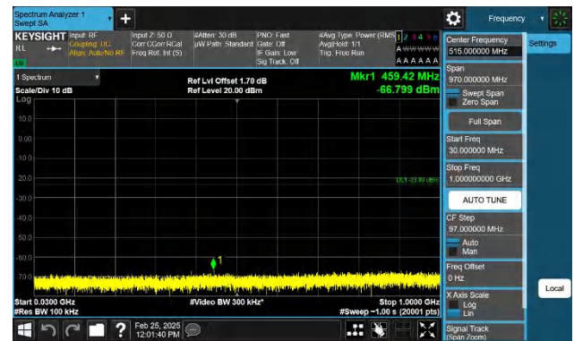
Band4-5MHz-QPSK-20175-1RB#24-30~1000-PASS
