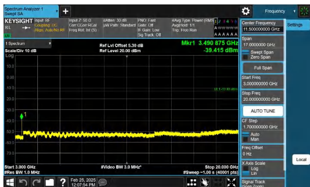
Band4-10MHz-QPSK-20350-1RB#0-3000~20000-PASS
