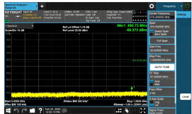
Band4-5MHz-QPSK-20375-1RB#24-30~1000-PASS
