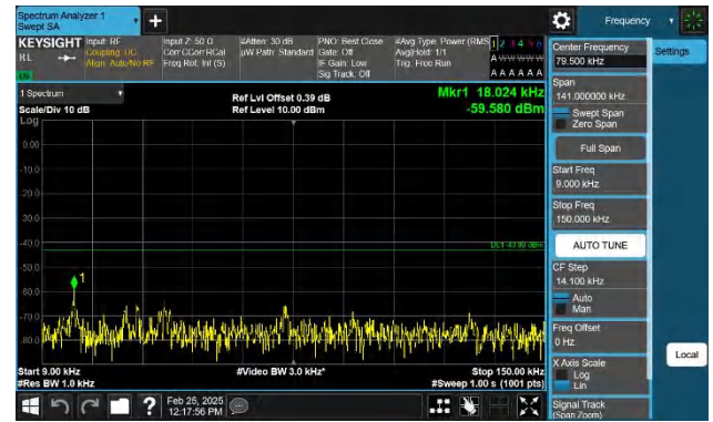
Band4-20MHz-QPSK-20300-1RB#99-0.009~0.15-PASS
