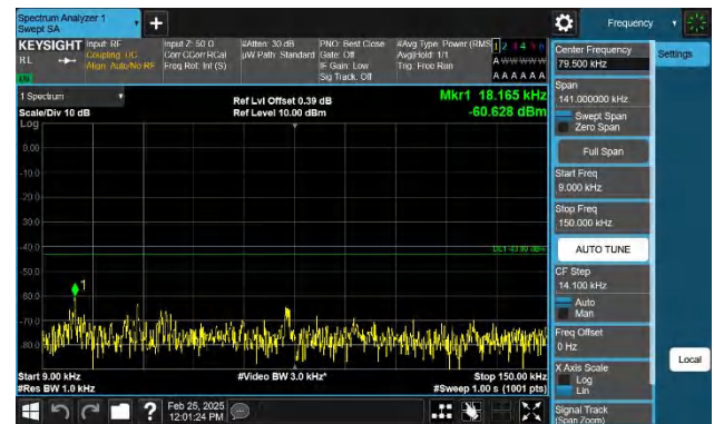
Band4-5MHz-QPSK-20175-1RB#24-0.009~0.15-PASS
