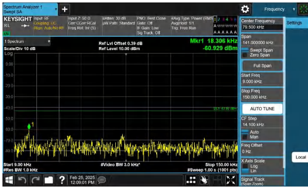
Band4-15MHz-QPSK-20025-1RB#0-0.009~0.15-PASS
