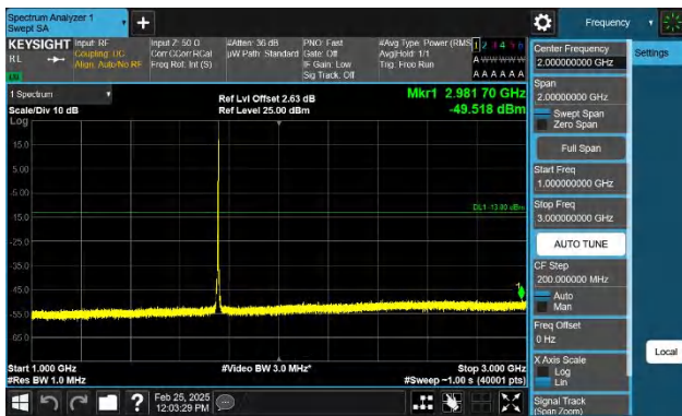
Band4-5MHz-QPSK-20375-1RB#24-1000~3000-PASS
