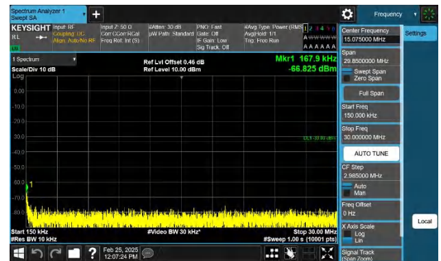
Band4-10MHz-QPSK-20350-1RB#0-0.15~30-PASS
