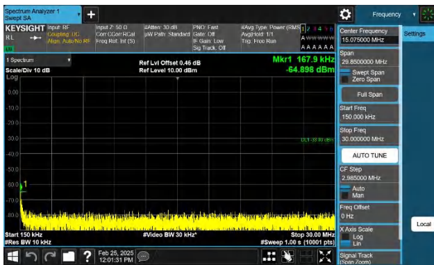
Band4-5MHz-QPSK-20175-1RB#24-0.15~30-PASS
