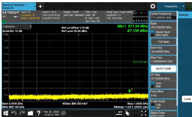
Band4-5MHz-QPSK-20375-1RB#0-30~1000-PASS
