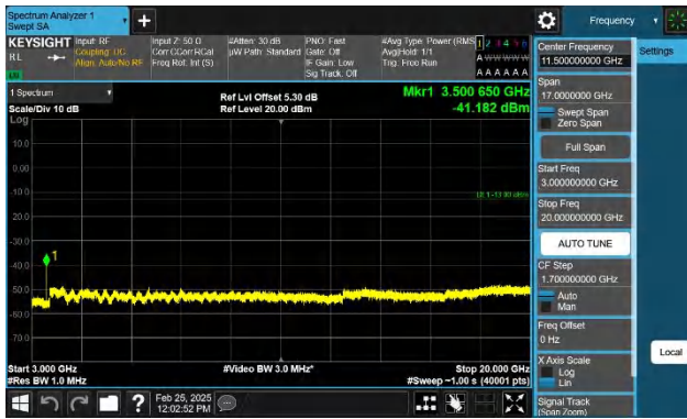
Band4-5MHz-QPSK-20375-1RB#0-3000~20000-PASS
