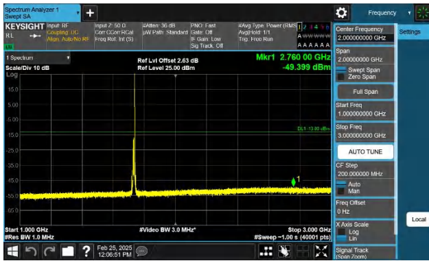
Band4-10MHz-QPSK-20175-1RB#49-1000~3000-PASS
