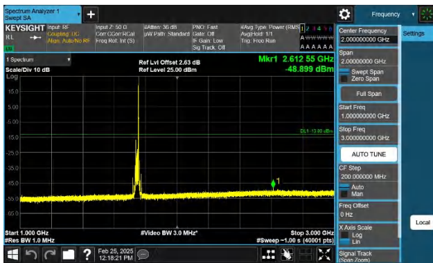
Band4-20MHz-QPSK-20300-1RB#99-1000~3000-PASS
