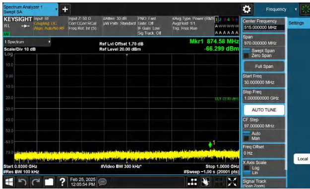
Band4-10MHz-QPSK-20175-1RB#0-30~1000-PASS
