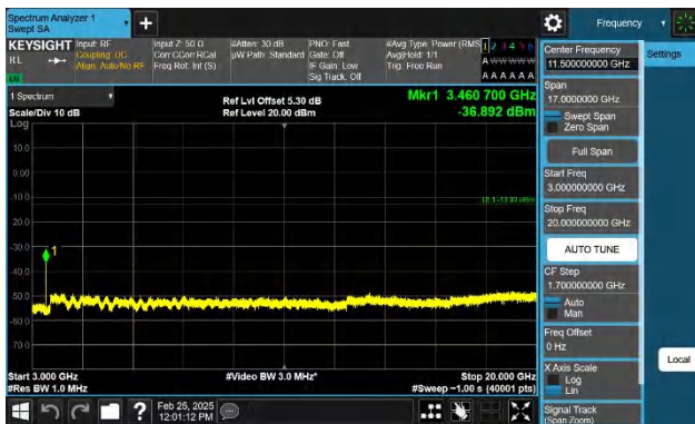
Band4-5MHz-QPSK-20175-1RB#0-3000~20000-PASS
