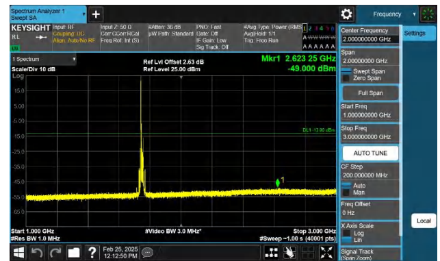
Band4-15MHz-QPSK-20325-1RB#0-1000~3000-PASS
