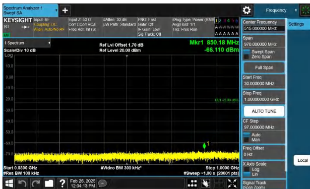
Band4-10MHz-QPSK-20000-1RB#0-30~1000-PASS
