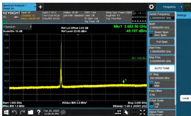
Band4-10MHz-QPSK-20350-1RB#49-1000~3000-PASS
