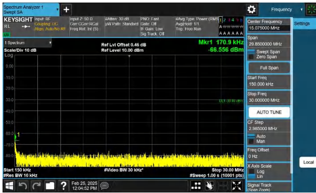
Band4-10MHz-QPSK-20000-1RB#49-0.15~30-PASS
