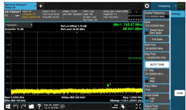
Band4-15MHz-QPSK-20175-1RB#74-30~1000-PASS
