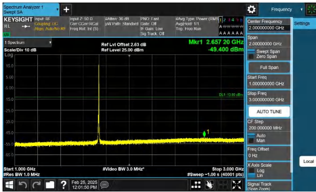
Band4-5MHz-QPSK-20175-1RB#24-1000~3000-PASS
