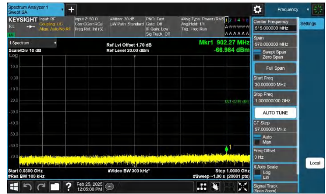
Band4-10MHz-QPSK-20000-1RB#49-30~1000-PASS
