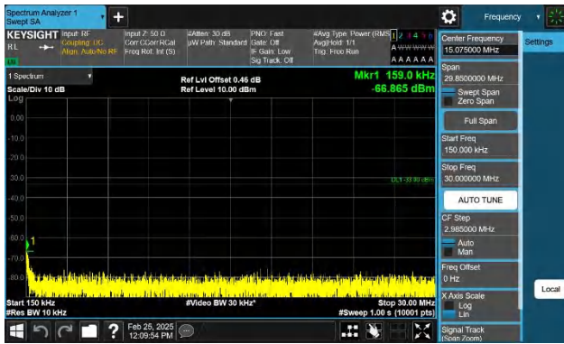
Band4-15MHz-QPSK-20025-1RB#74-0.15~30-PASS
