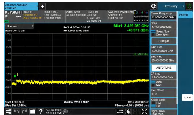
Band4-5MHz-QPSK-19975-1RB#24-3000~20000-PASS
