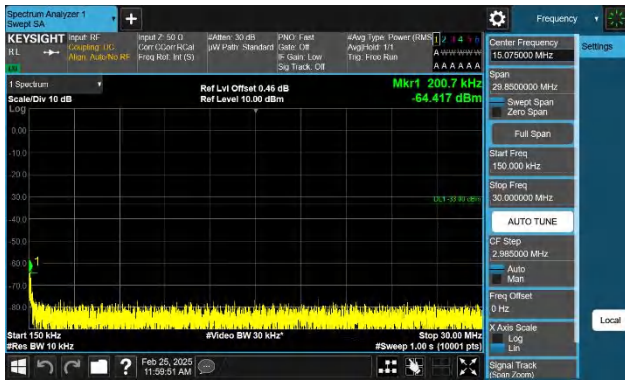
Band4-5MHz-QPSK-19975-1RB#24-0.15~30-PASS
