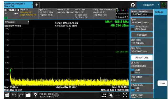
Band4-10MHz-QPSK-20000-1RB#0-0.15~30-PASS
