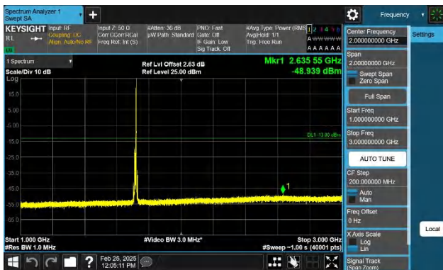
Band4-10MHz-QPSK-20000-1RB#49-1000~3000-PASS
