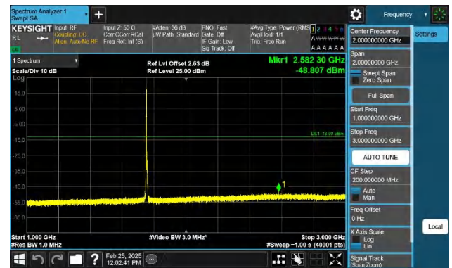
Band4-5MHz-QPSK-20375-1RB#0-1000~3000-PASS
