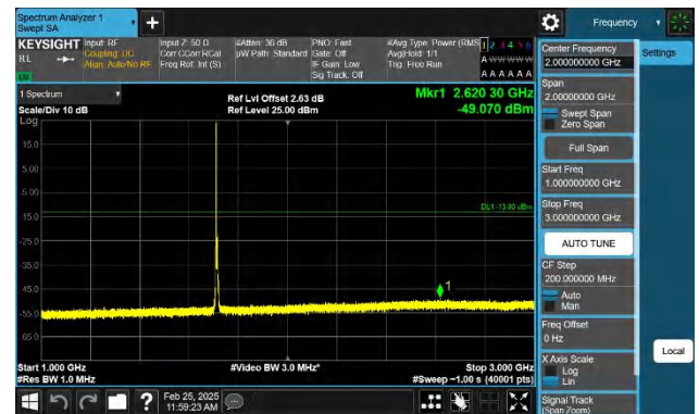
Band4-5MHz-QPSK-19975-1RB#0-1000~3000-PASS
