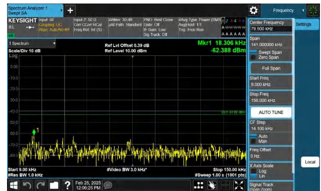
Band4-10MHz-QPSK-20175-1RB#49-0.009~0.15-PASS
