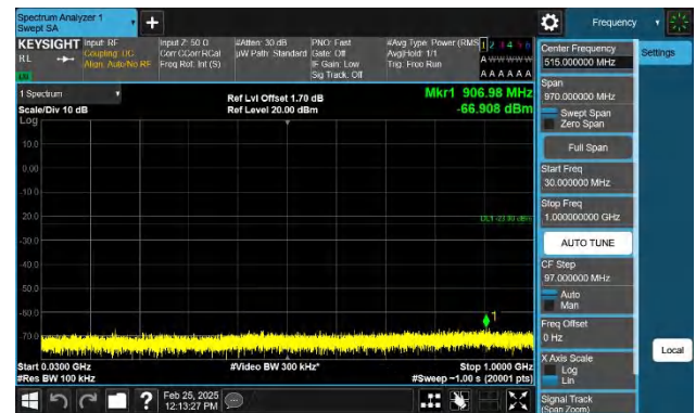
Band4-15MHz-QPSK-20325-1RB#74-30~1000-PASS
