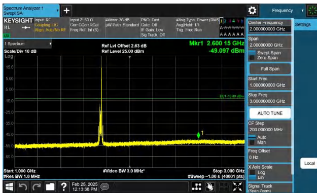
Band4-15MHz-QPSK-20325-1RB#74-1000~3000-PASS
