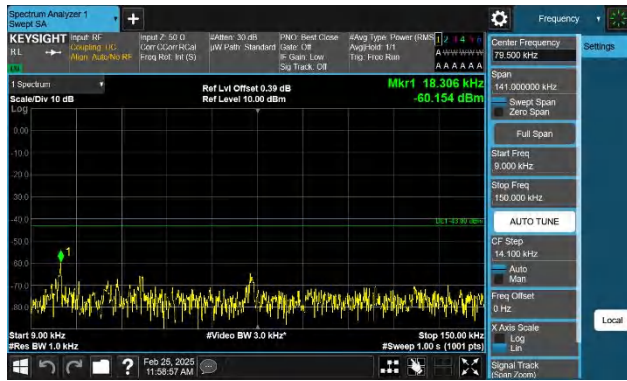
Band4-5MHz-QPSK-19975-1RB#0-0.009~0.15-PASS
