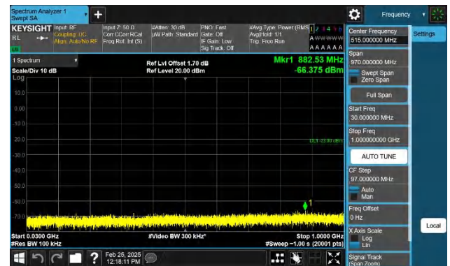
Band4-20MHz-QPSK-20300-1RB#99-30~1000-PASS
