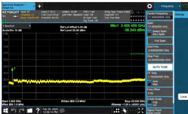
Band4-10MHz-QPSK-20175-1RB#0-3000~20000-PASS
