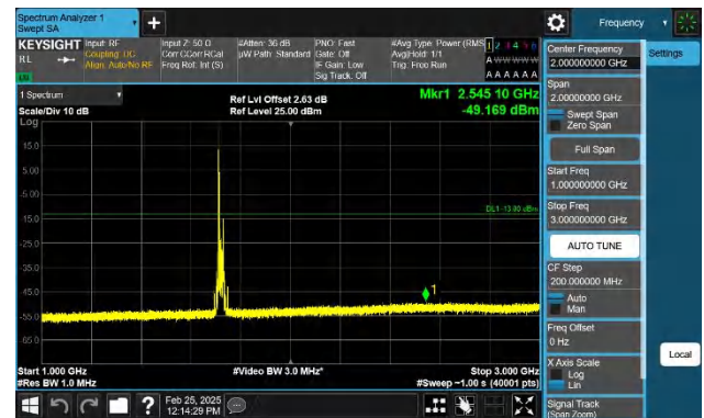
Band4-20MHz-QPSK-20050-1RB#0-1000~3000-PASS
