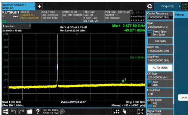
Band4-5MHz-QPSK-19975-1RB#24-1000~3000-PASS
