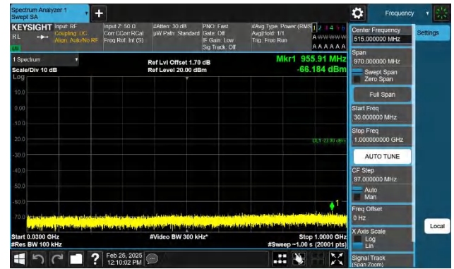
Band4-15MHz-QPSK-20025-1RB#74-30~1000-PASS
