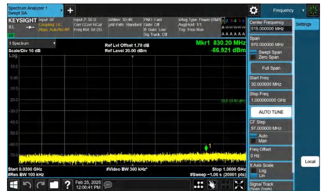
Band4-10MHz-QPSK-20175-1RB#49-30~1000-PASS
