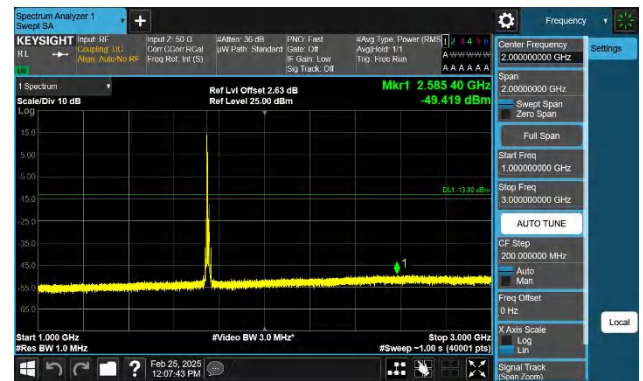
Band4-10MHz-QPSK-20350-1RB#0-1000~3000-PASS
