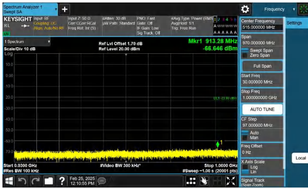
Band4-15MHz-QPSK-20175-1RB#0-30~1000-PASS
