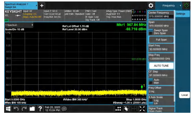
Band4-20MHz-QPSK-20050-1RB#99-30~1000-PASS
