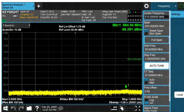
Band4-10MHz-QPSK-20350-1RB#0-30~1000-PASS
