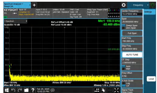
Band4-5MHz-QPSK-20375-1RB#0-0.15~30-PASS
