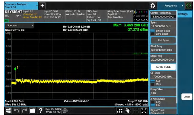
Band4-5MHz-QPSK-20175-1RB#24-3000~20000-PASS
