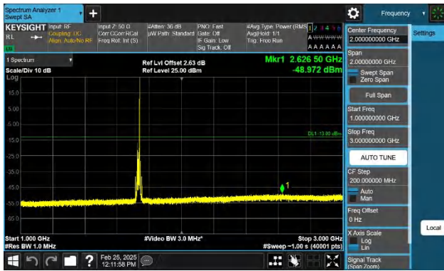
Band4-15MHz-QPSK-20175-1RB#74-1000~3000-PASS
