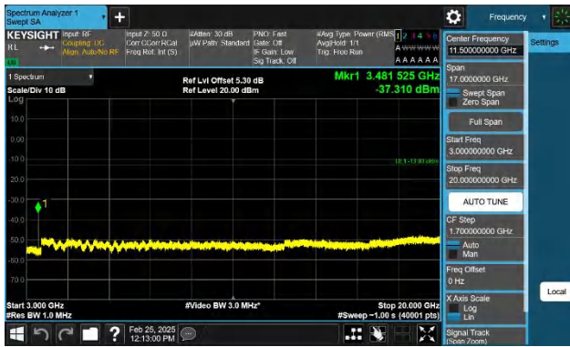
Band4-15MHz-QPSK-20325-1RB#0-3000~20000-PASS
