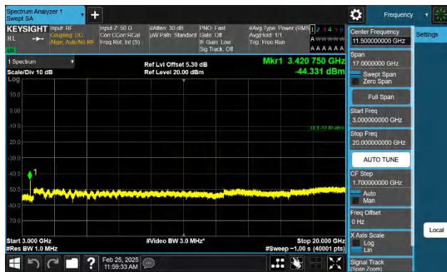
Band4-5MHz-QPSK-19975-1RB#0-3000~20000-PASS
