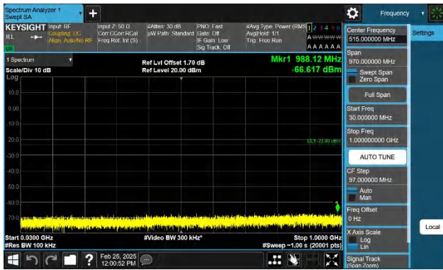
Band4-5MHz-QPSK-20175-1RB#0-30~1000-PASS
