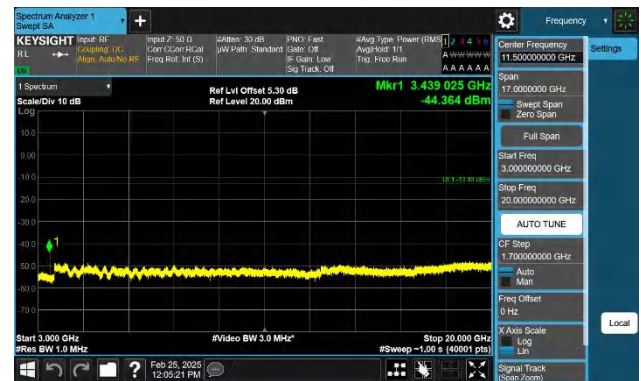
Band4-10MHz-QPSK-20000-1RB#49-3000~20000-PASS
