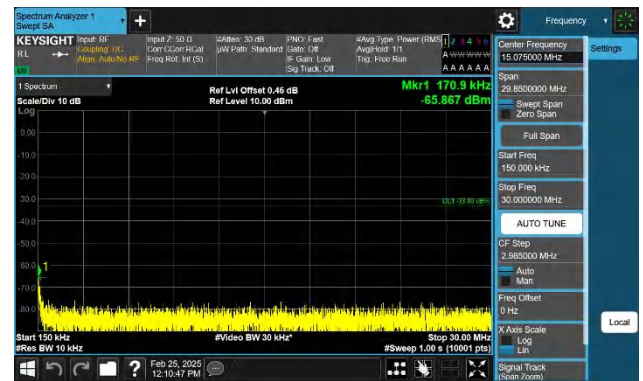
Band4-15MHz-QPSK-20175-1RB#0-0.15~30-PASS
