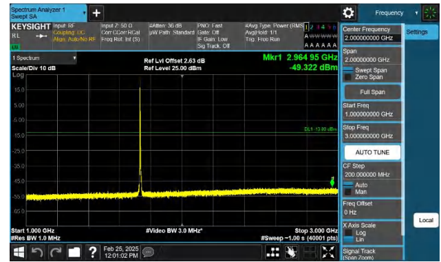
Band4-5MHz-QPSK-20175-1RB#0-1000~3000-PASS
