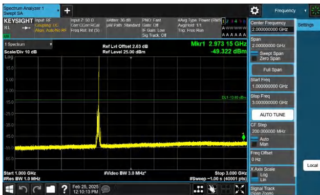
Band4-15MHz-QPSK-20025-1RB#74-1000~3000-PASS
