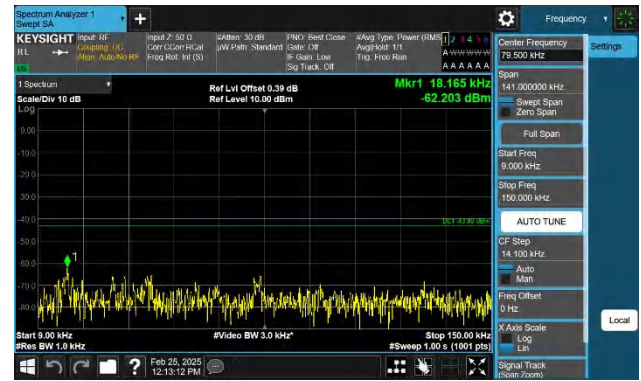
Band4-15MHz-QPSK-20325-1RB#74-0.009~0.15-PASS
