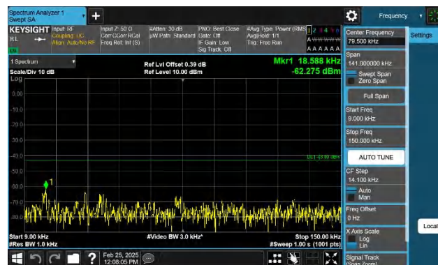
Band4-10MHz-QPSK-20350-1RB#49-0.009~0.15-PASS
