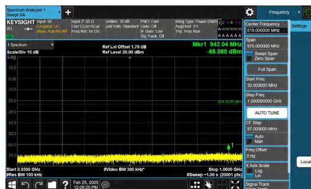
Band4-10MHz-QPSK-20350-1RB#49-30~1000-PASS
