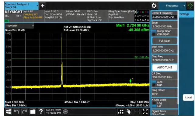
Band4-10MHz-QPSK-20175-1RB#0-1000~3000-PASS
