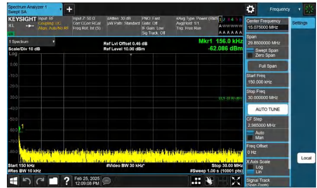
Band4-15MHz-QPSK-20025-1RB#0-0.15~30-PASS
