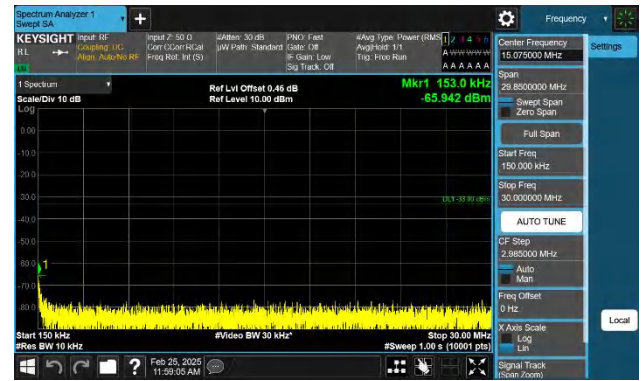
Band4-5MHz-QPSK-19975-1RB#0-0.15~30-PASS
