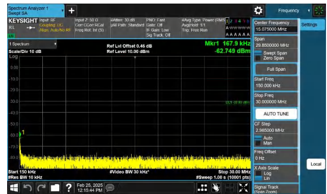
Band4-20MHz-QPSK-20175-1RB#0-0.15~30-PASS
