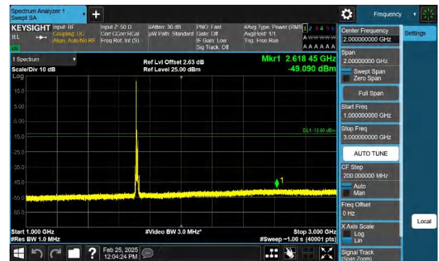
Band4-10MHz-QPSK-20000-1RB#0-1000~3000-PASS
