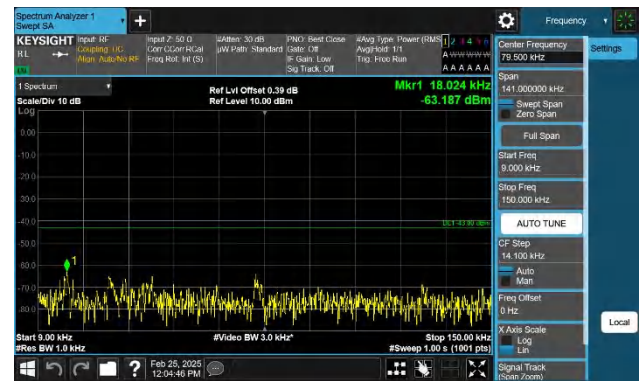
Band4-10MHz-QPSK-20000-1RB#49-0.009~0.15-PASS
